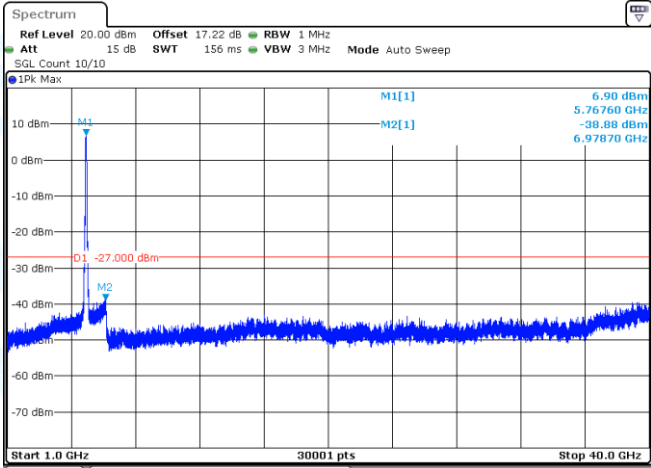
11AX80MIMO-Ant1-5775-1000~40000-PASS
