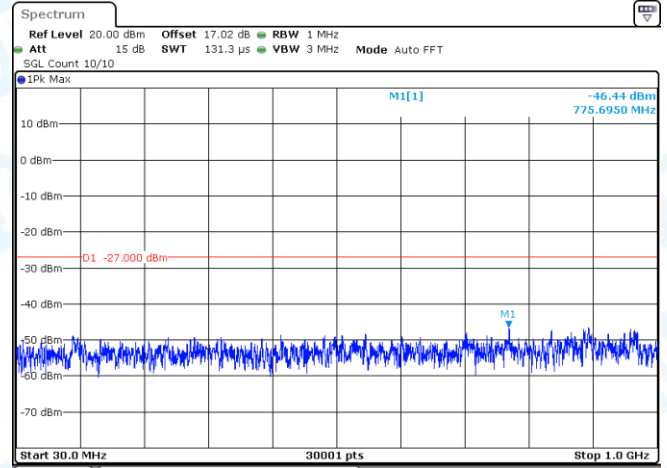
11AX40MIMO-Ant2-5270-30~1000-PASS
