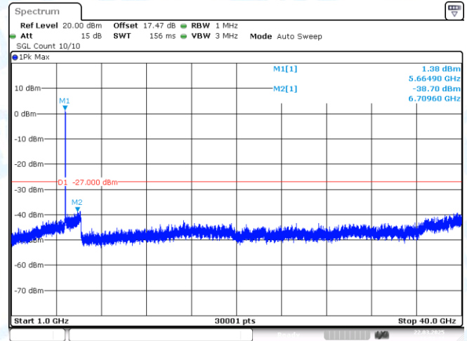
11AX40MIMO-Ant2-5670-1000~40000-PASS
