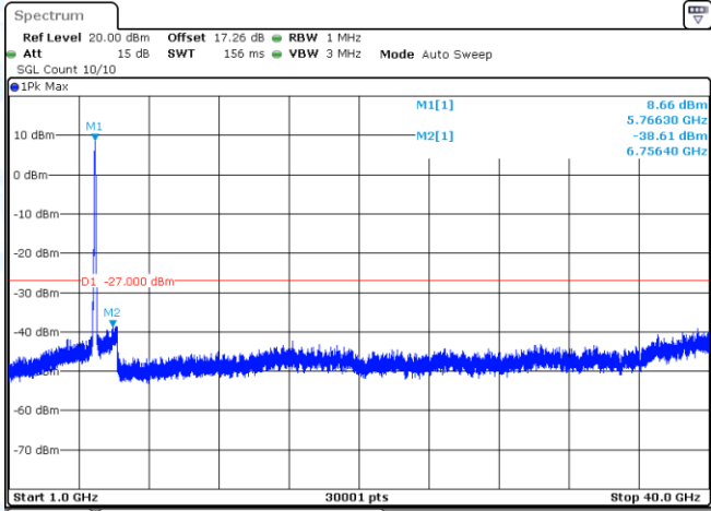
11AX80MIMO-Ant2-5775-1000~40000-PASS
