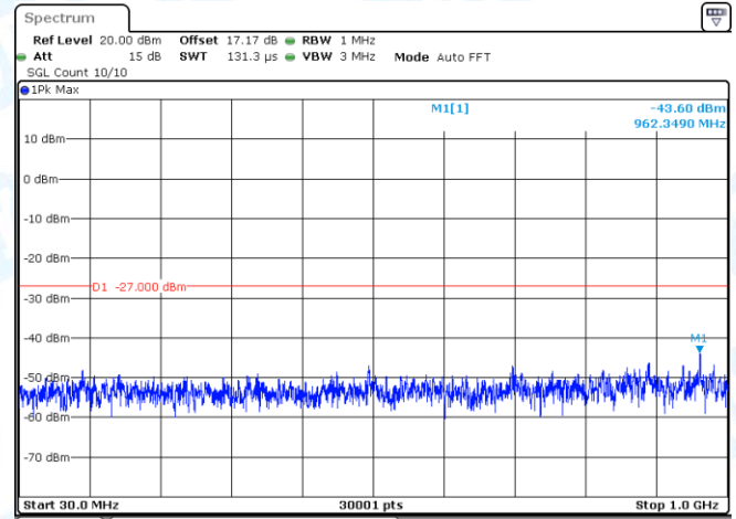
11AX40MIMO-Ant2-5550-30~1000-PASS
