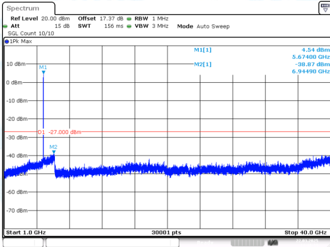
11AX40MIMO-Ant1-5670-1000~40000-PASS
