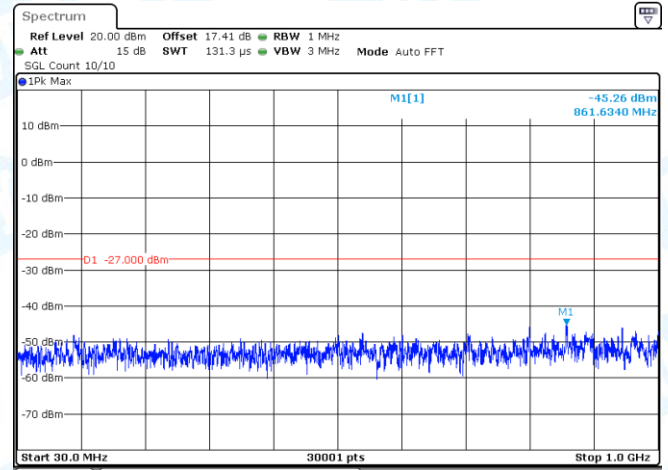
11AX80MIMO-Ant2-5690-30~1000-PASS
