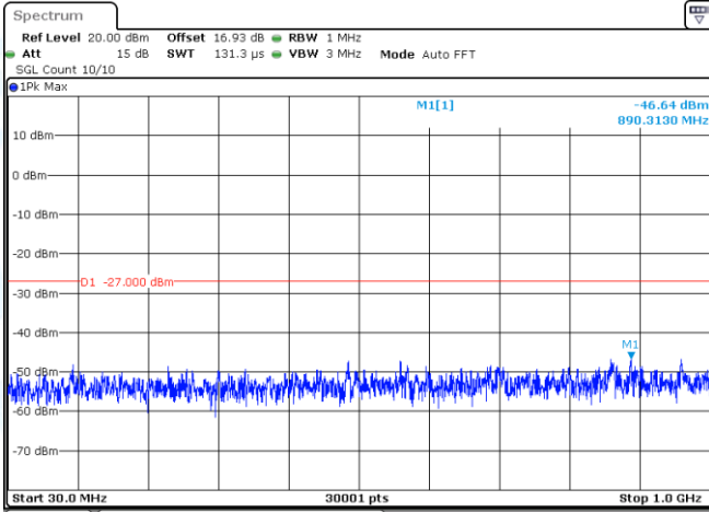
11AX80MIMO-Ant1-5290-30~1000-PASS
