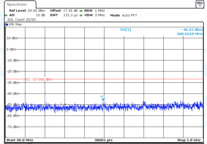
11AX20MIMO-Ant2-5825-30~1000-PASS
