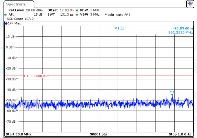
11AX80MIMO-Ant2-5290-30~1000-PASS
