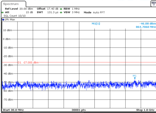
11AX80MIMO-Ant1-5690-30~1000-PASS
