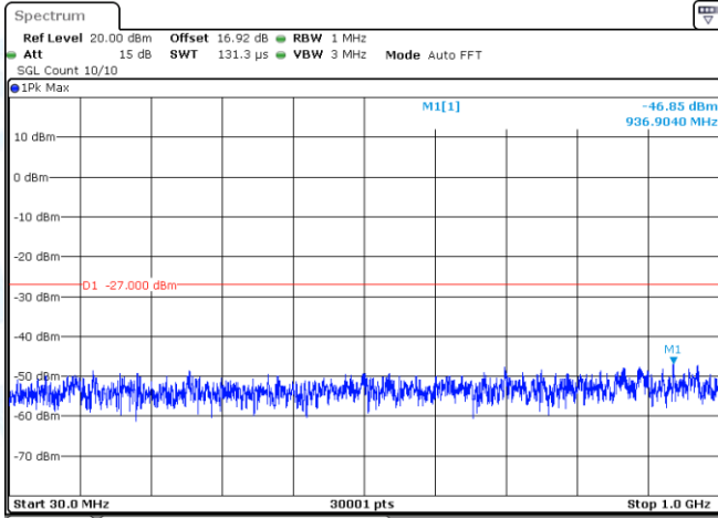
11AX40MIMO-Ant1-5270-30~1000-PASS
