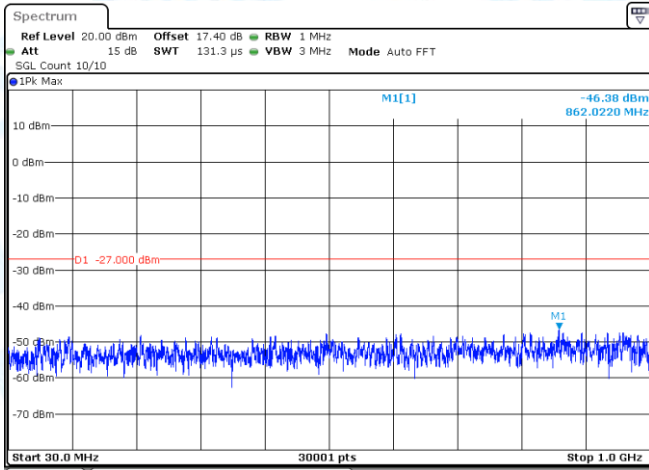
11AX20MIMO-Ant1-5720-30~1000-PASS
