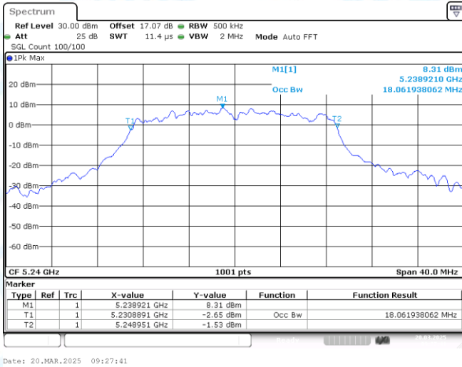
11N20MIMO-Ant2-5240
