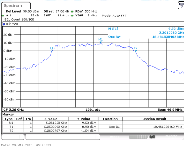
11N20MIMO-Ant2-5260
