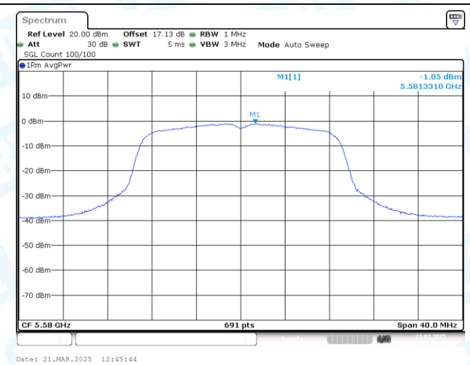
11AC20MIMO-Ant2-5580-PASS
