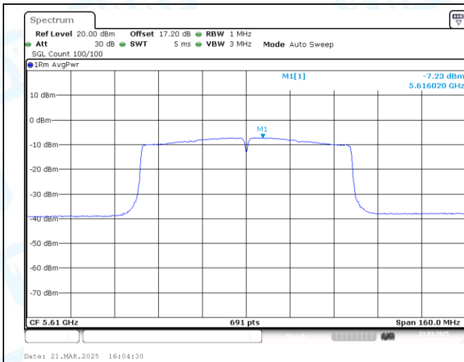
11AC80MIMO-Ant1-5610-PASS
