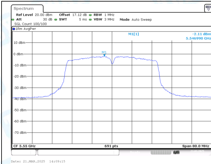
11AC40MIMO-Ant1-5550-PASS
