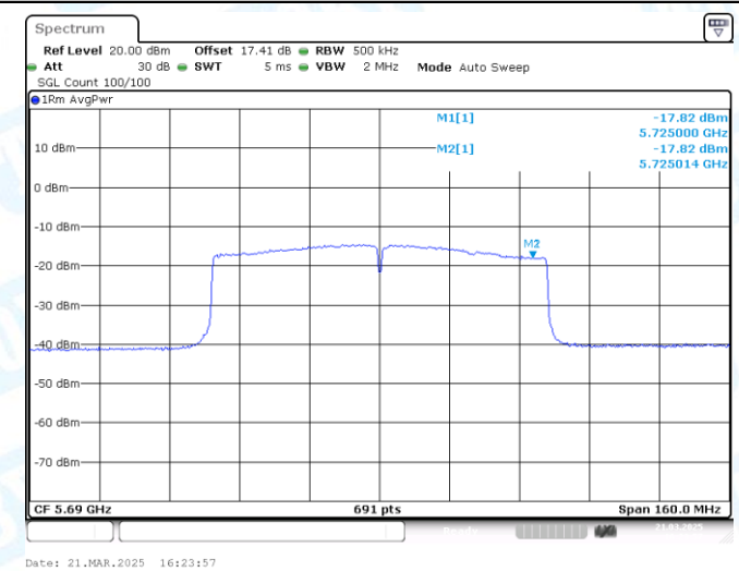
11AC80MIMO-Ant2-5690_UNII-3-PASS
