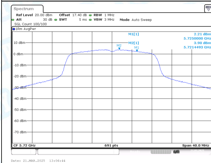
11AC20MIMO-Ant1-5720_UNII-2C-PASS
