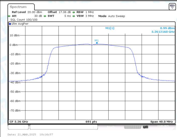
11AX20MIMO-Ant2-5260-PASS
