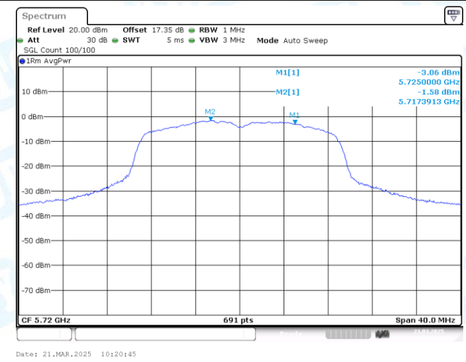
11N20MIMO-Ant2-5720_UNII-2C-PASS
