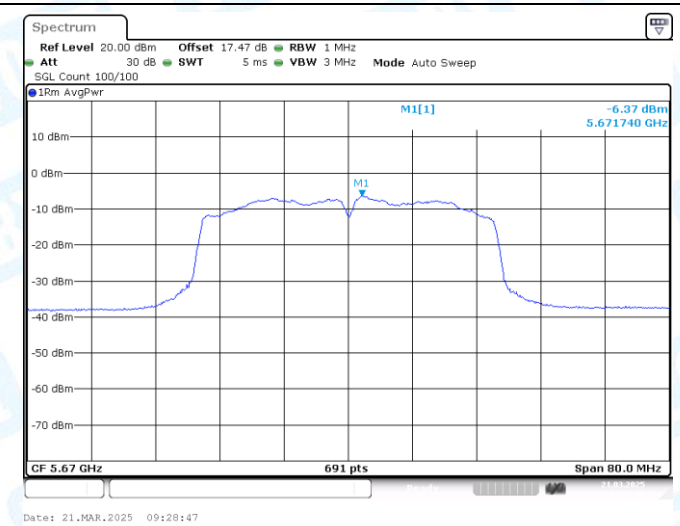
11N40MIMO-Ant2-5670-PASS
