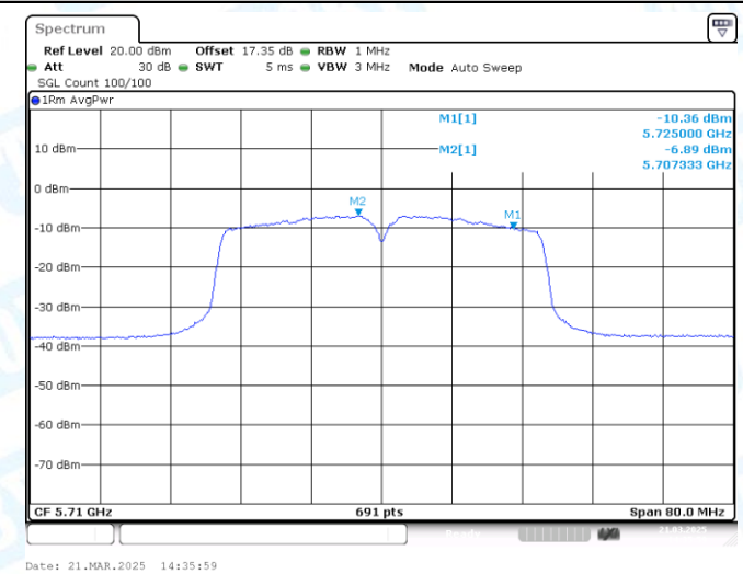
11AC40MIMO-Ant2-5710_UNII-2C-PASS
