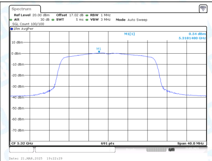
11AX20MIMO-Ant2-5320-PASS
