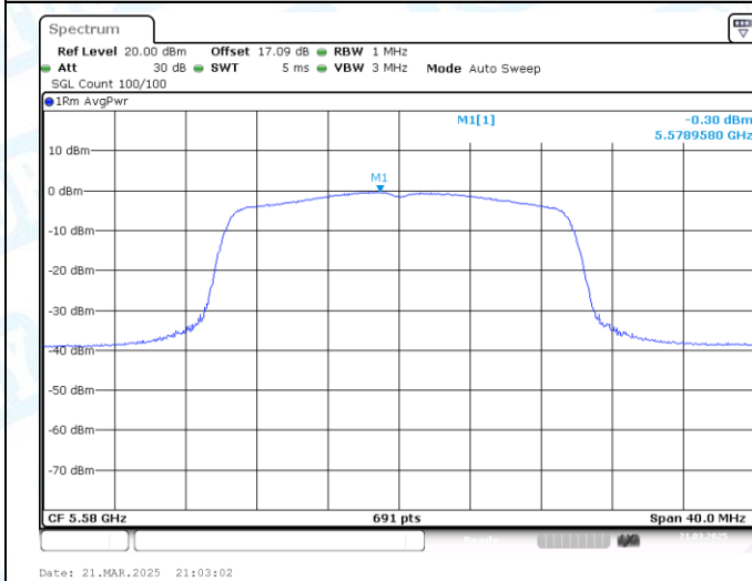
11AX20MIMO-Ant1-5580-PASS
