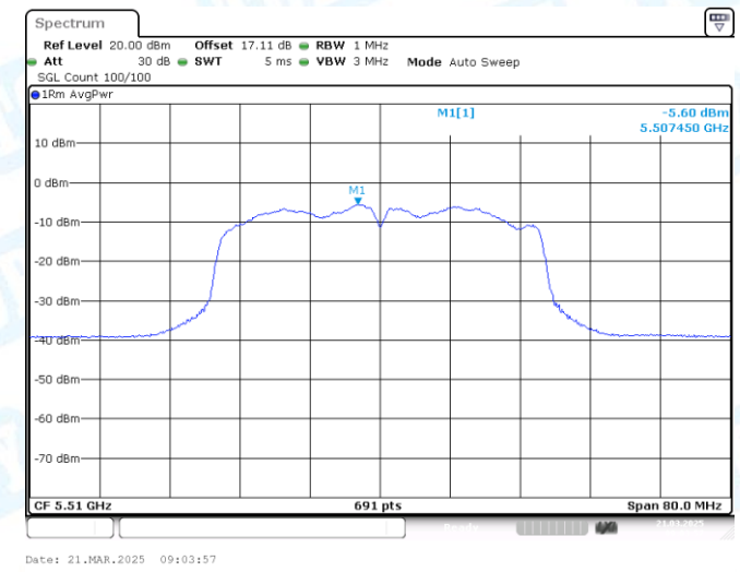
11N40MIMO-Ant2-5510-PASS
