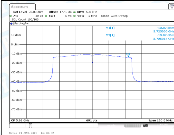
11AC80MIMO-Ant1-5690_UNII-3-PASS
