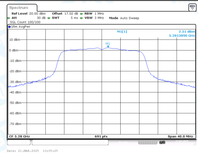
11N20MIMO-Ant2-5280-PASS
