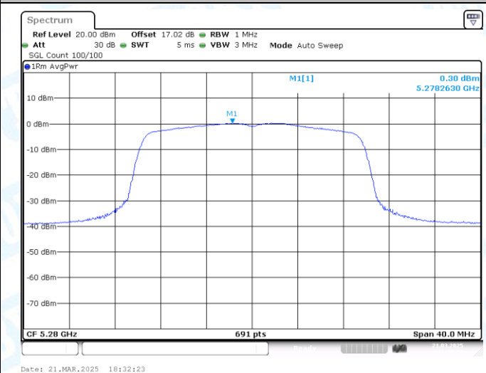
11AX20MIMO-Ant2-5280-PASS
