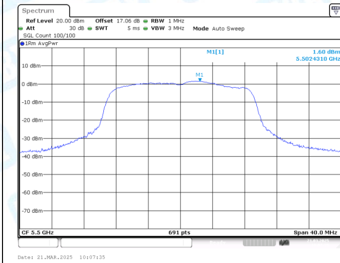
11N20MIMO-Ant1-5500-PASS
