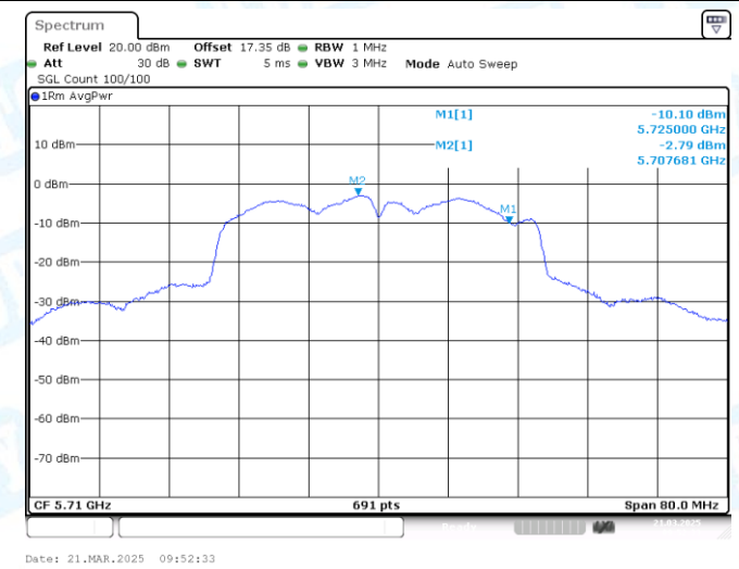
11N40MIMO-Ant2-5710_UNII-2C-PASS
