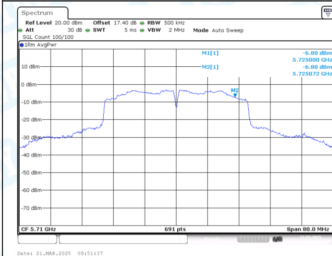
11N40MIMO-Ant1-5710_UNII-3-PASS
