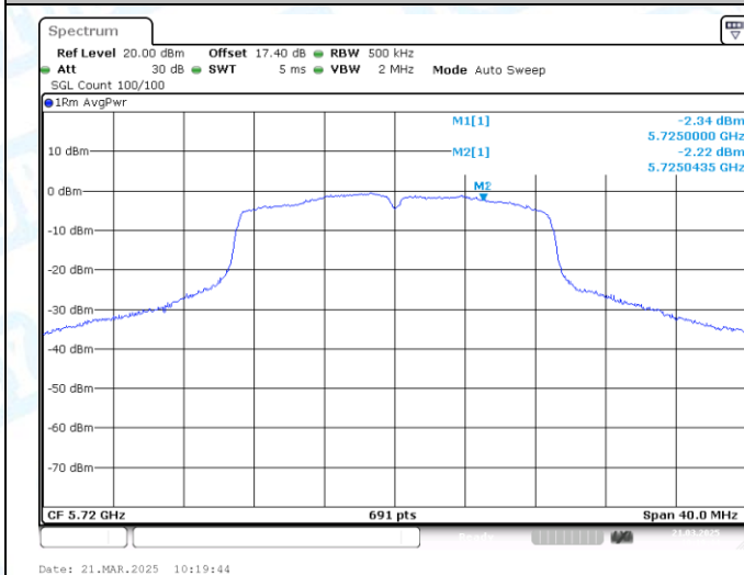
11N20MIMO-Ant1-5720_UNII-3-PASS
