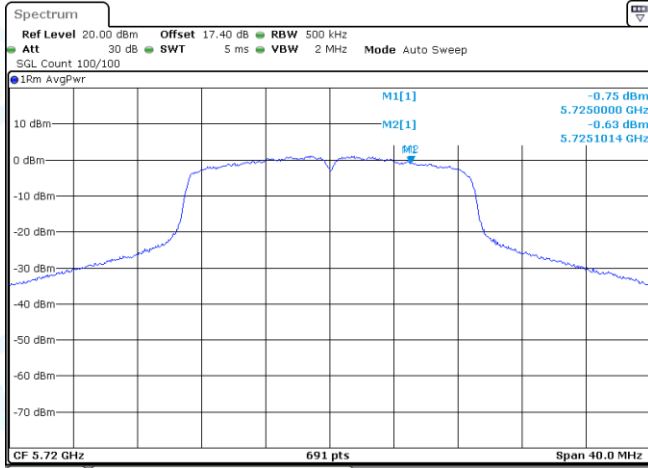
11AC20MIMO-Ant1-5720_UNII-3-PASS
