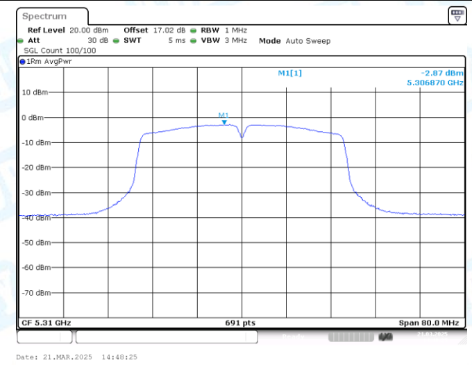
11AC40MIMO-Ant2-5310-PASS
