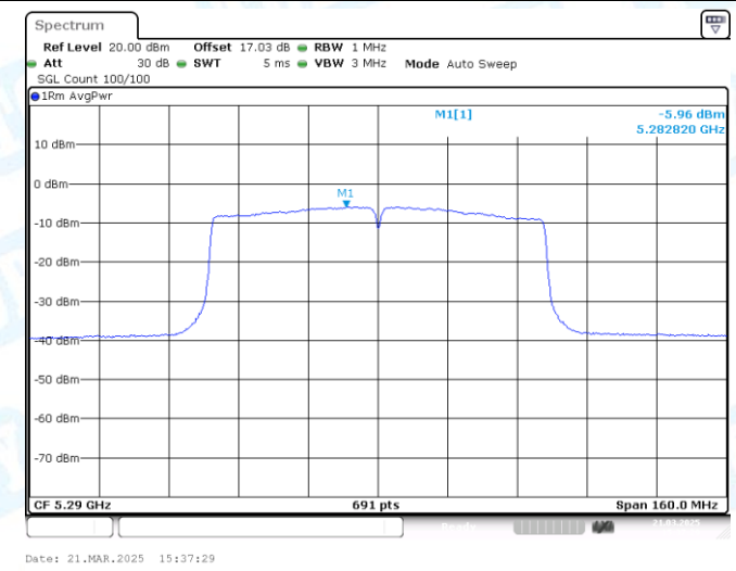
11AC80MIMO-Ant2-5290-PASS
