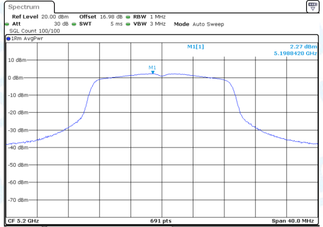
11AC20MIMO-Ant2-5200-PASS
