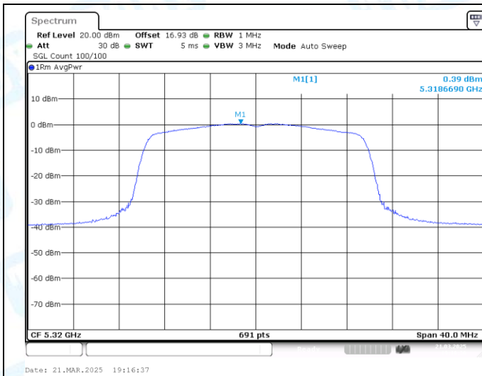
11AX20MIMO-Ant1-5320-PASS
