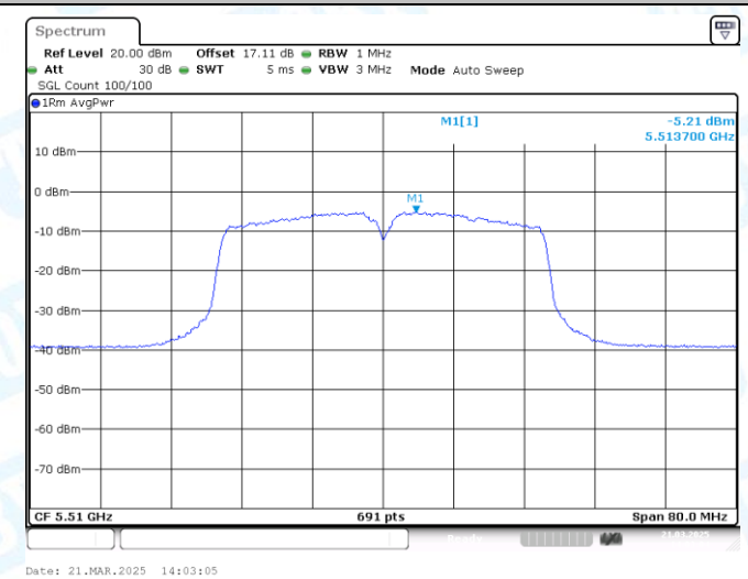
11AC40MIMO-Ant2-5510-PASS
