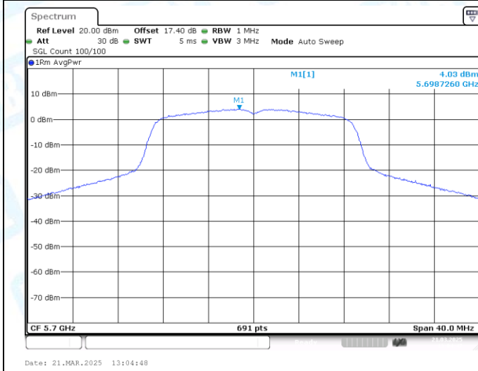
11AC20MIMO-Ant1-5700-PASS
