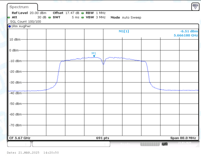
11AC40MIMO-Ant2-5670-PASS
