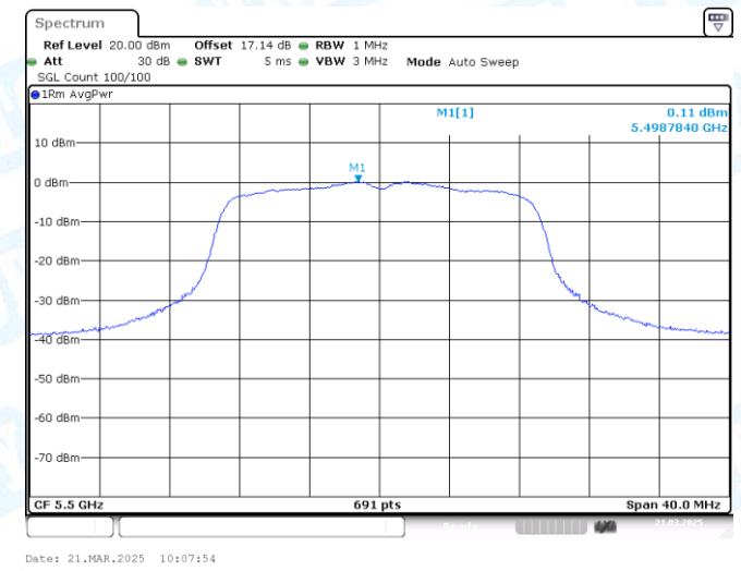
11N20MIMO-Ant2-5500-PASS
