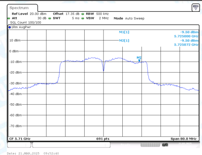
11N40MIMO-Ant2-5710_UNII-3-PASS
