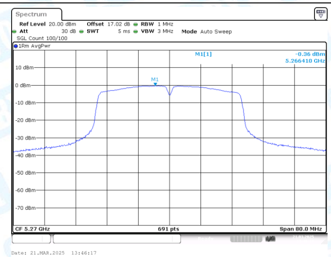
11AC40MIMO-Ant2-5270-PASS
