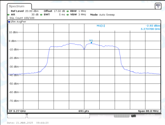
11N40MIMO-Ant2-5270-PASS
