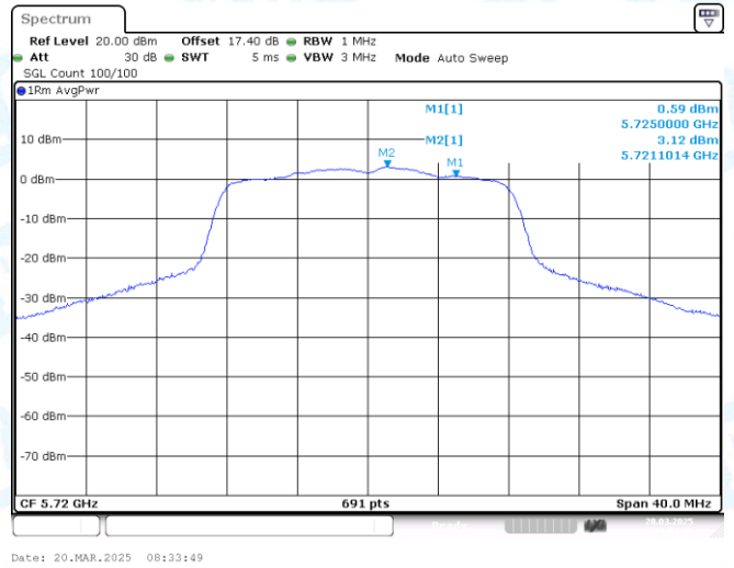
11A-Ant1-5720_PASS_UNII-2C-PASS
