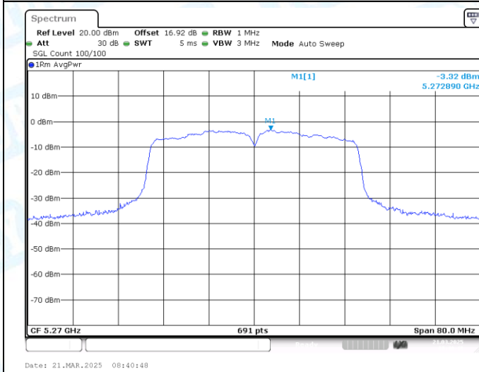
11N40MIMO-Ant1-5270-PASS
