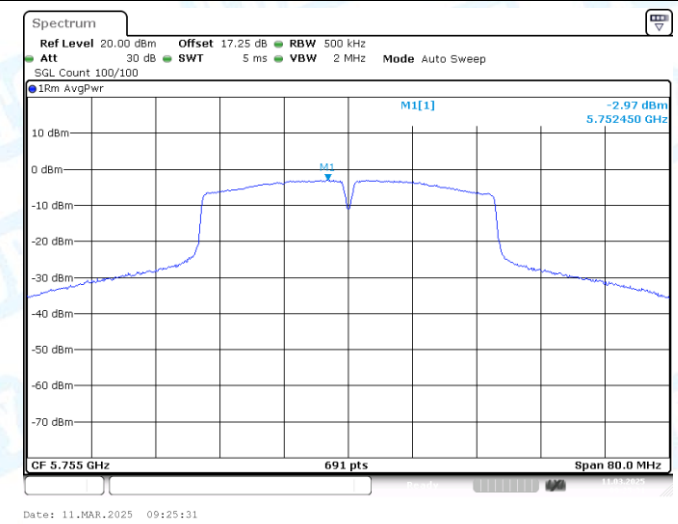
11AC40MIMO-Ant2-5755-PASS
