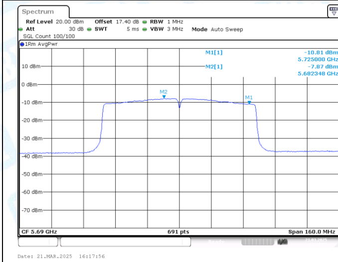
11AC80MIMO-Ant1-5690_UNII-2C-PASS
