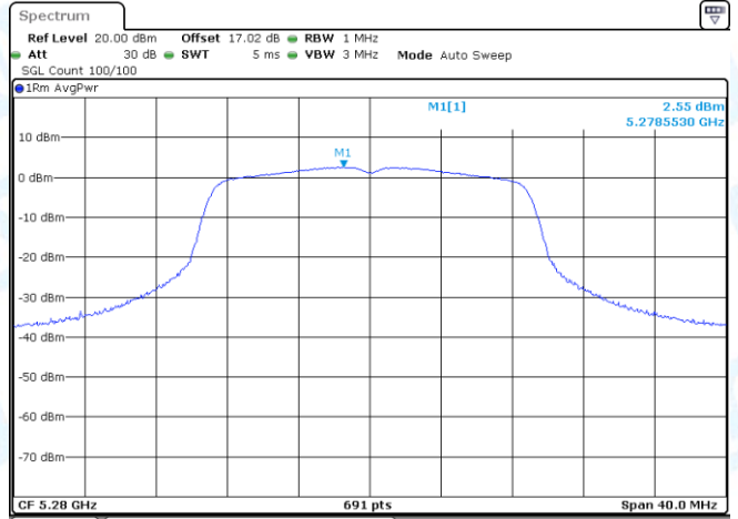
11AC20MIMO-Ant2-5280-PASS
