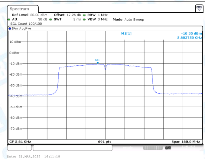
11AC80MIMO-Ant2-5610-PASS
