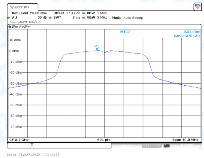
11AC20MIMO-Ant2-5700-PASS
