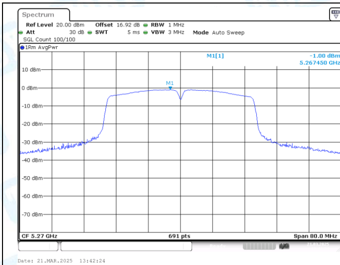
11AC40MIMO-Ant1-5270-PASS
