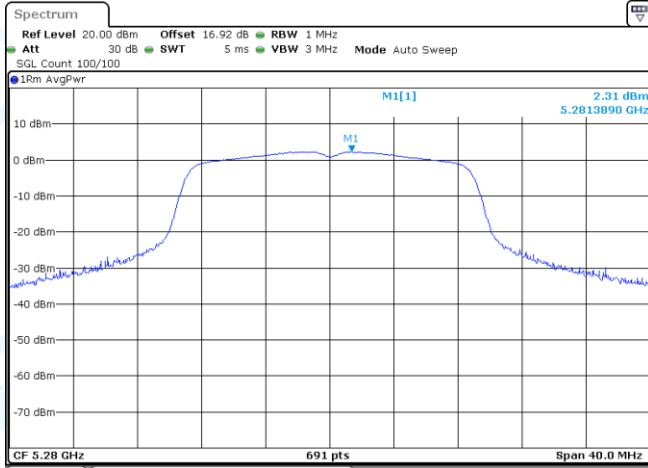
11AC20MIMO-Ant1-5280-PASS
