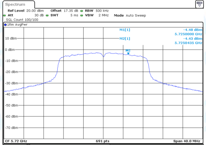
11AC20MIMO-Ant2-5720_UNII-3-PASS
