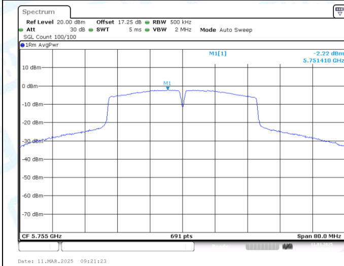
11AC40MIMO-Ant1-5755-PASS
