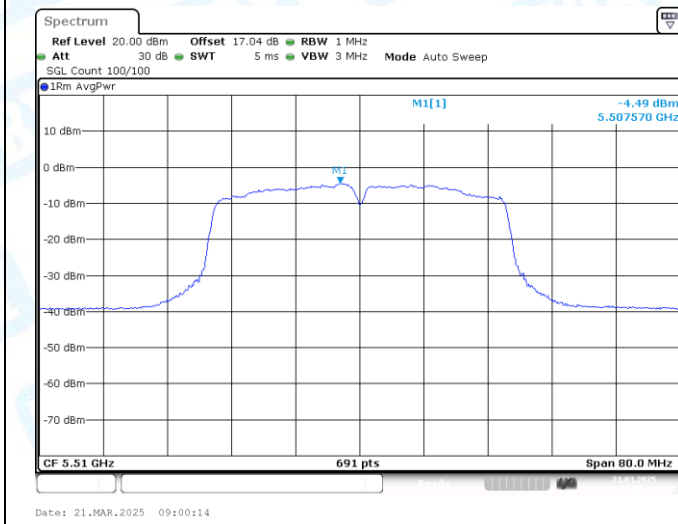
11N40MIMO-Ant1-5510-PASS
