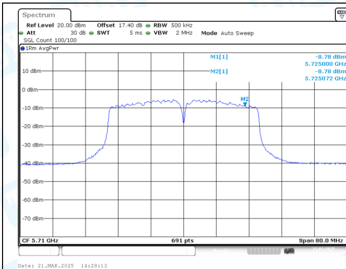
11AC40MIMO-Ant1-5710_UNII-3-PASS
