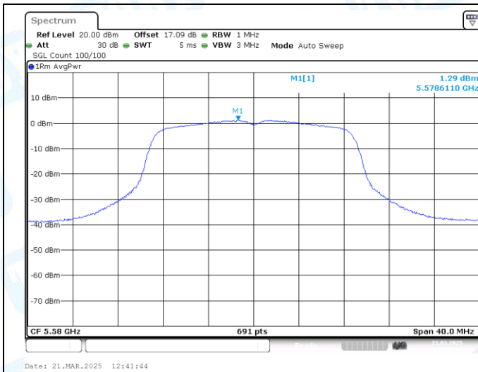
11AC20MIMO-Ant1-5580-PASS
