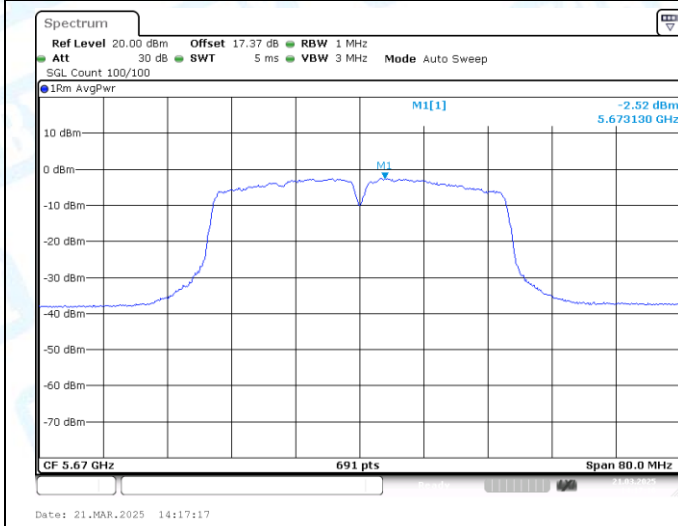
11AC40MIMO-Ant1-5670-PASS
