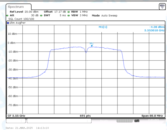
11AC40MIMO-Ant2-5550-PASS
