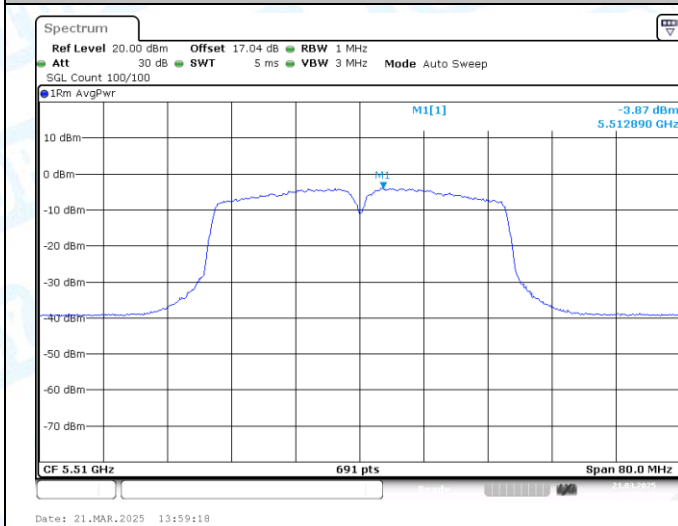
11AC40MIMO-Ant1-5510-PASS
