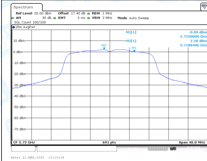
11N20MIMO-Ant1-5720_UNII-2C-PASS
