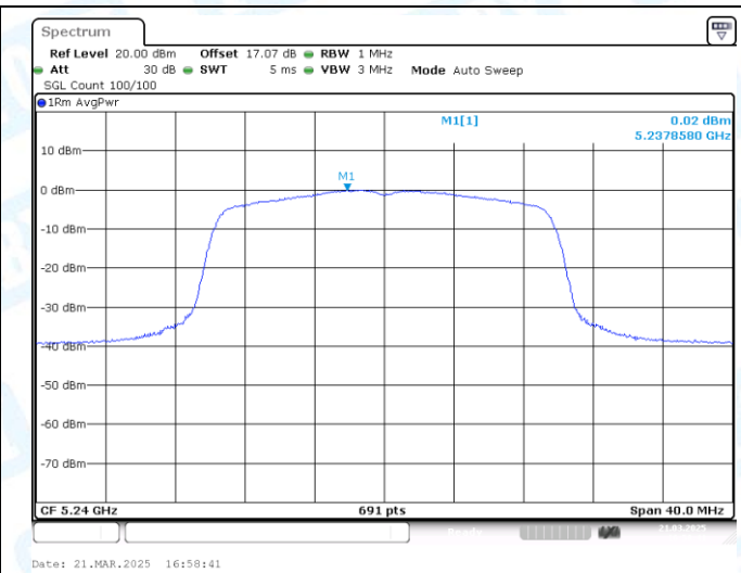
11AX20MIMO-Ant2-5240-PASS
