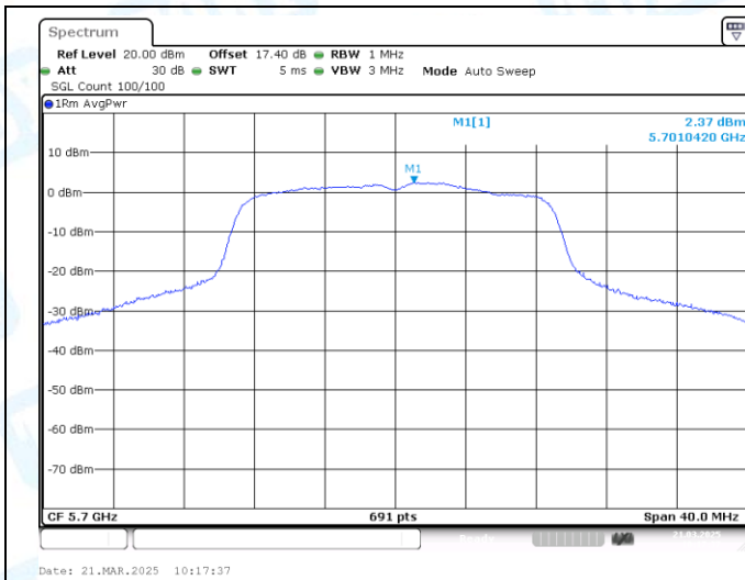
11N20MIMO-Ant1-5700-PASS
