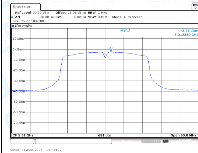
11AC40MIMO-Ant1-5310-PASS
