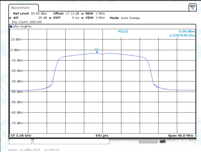
11AX20MIMO-Ant2-5580-PASS
