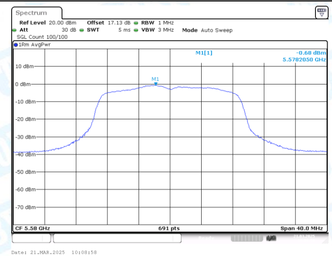
11N20MIMO-Ant2-5580-PASS
