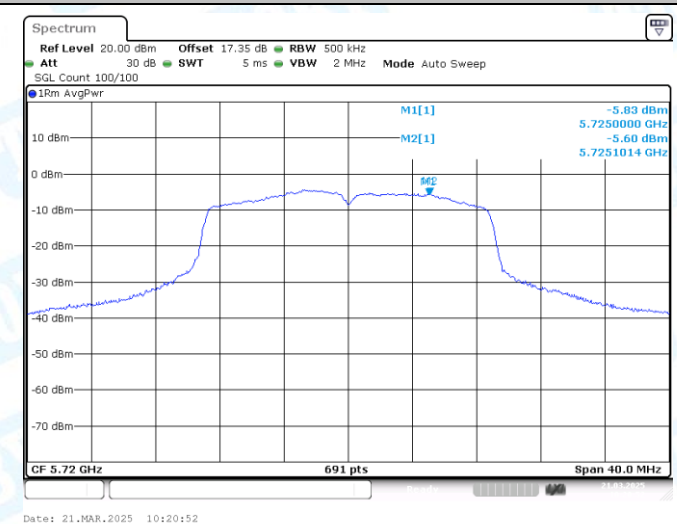
11N20MIMO-Ant2-5720_UNII-3-PASS
