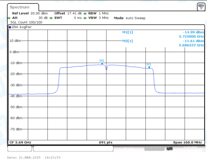
11AC80MIMO-Ant2-5690_UNII-2C-PASS
