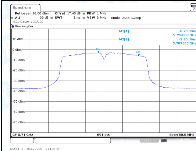
11AC40MIMO-Ant1-5710_UNII-2C-PASS
