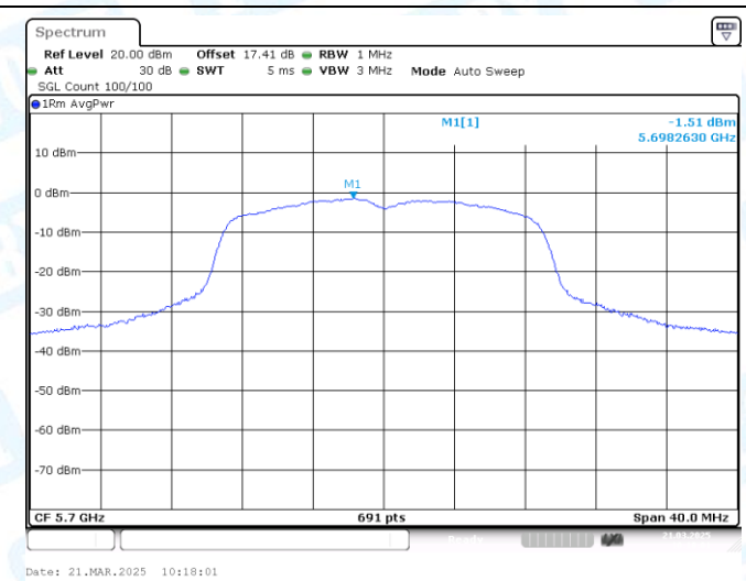
11N20MIMO-Ant2-5700-PASS
