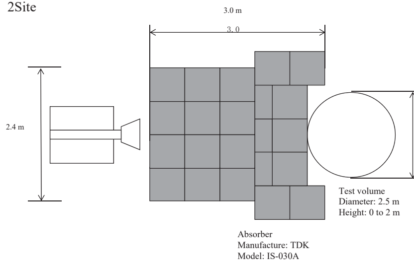
Figure. Absorber arrangement
