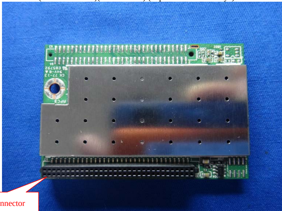
(6) EUT Photo (M/N: CY920-A)(Main Source) (64pin connector / Xinya)
