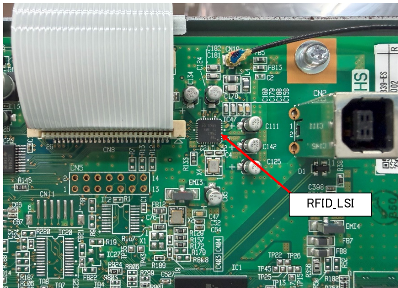
Radio Unit (Top side)
