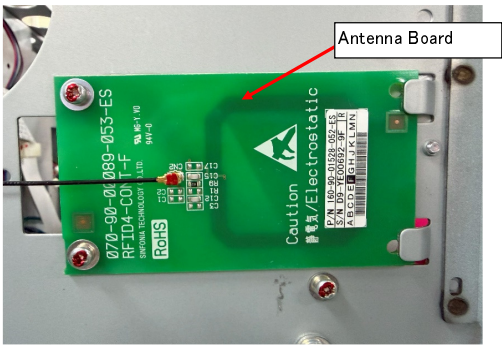
Mounting position (Antenna Board)
