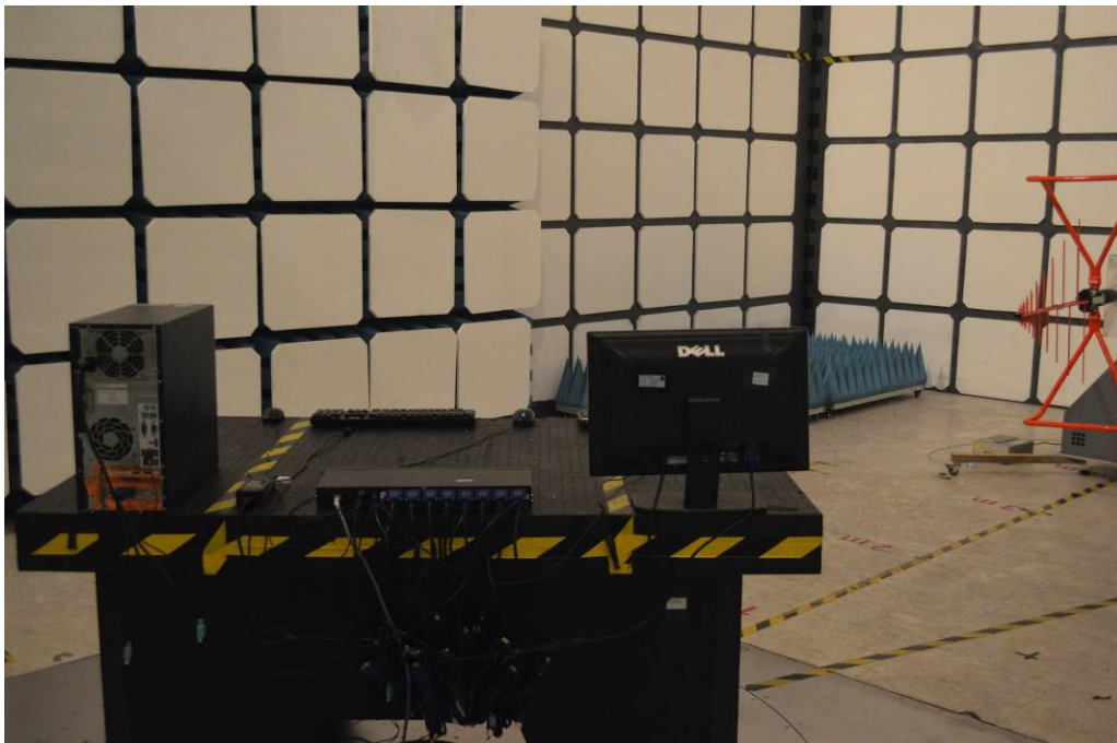
Back View of Radiated Emission Test (30MHz ~ 1GHz)
