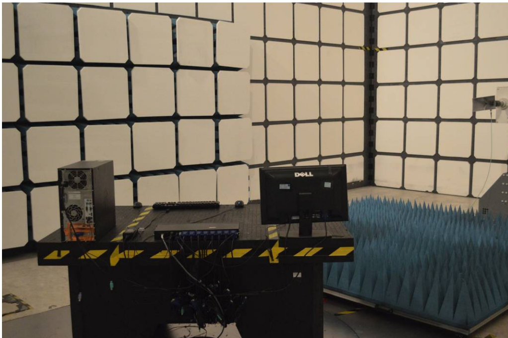
Back View of Radiated Emission Test (1GHz ~ 18GHz)
