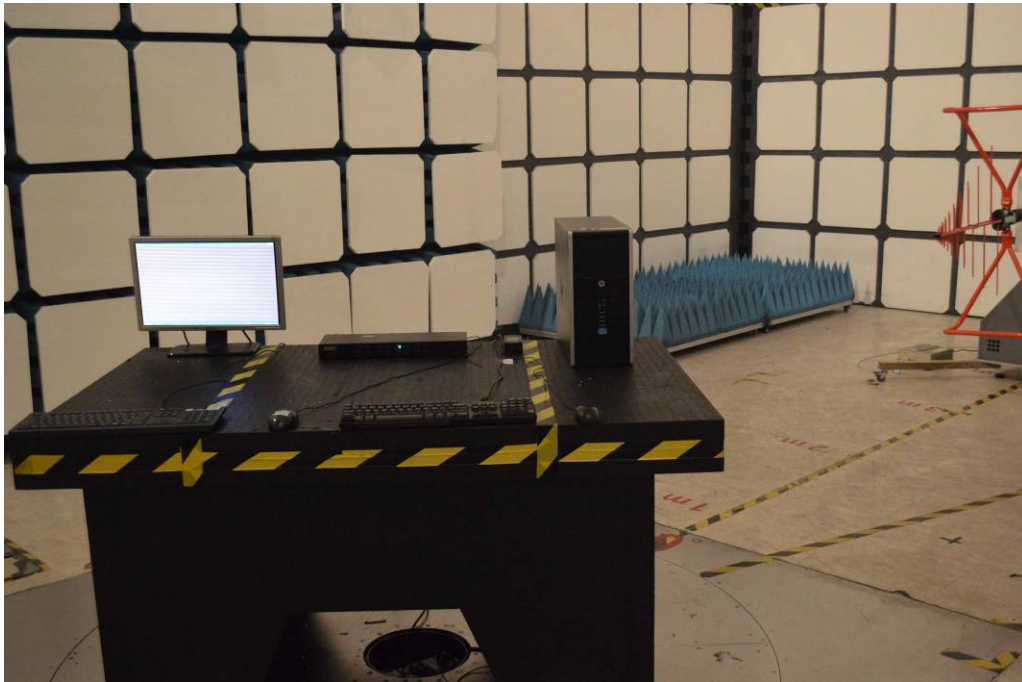
Front View of Radiated Emission Test (30MHz ~ 1GHz)
