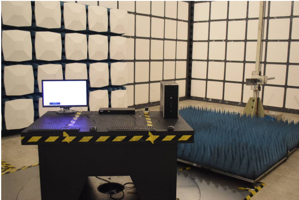
Front View of Radiated Emission Test (1GHz ~ 18GHz)
