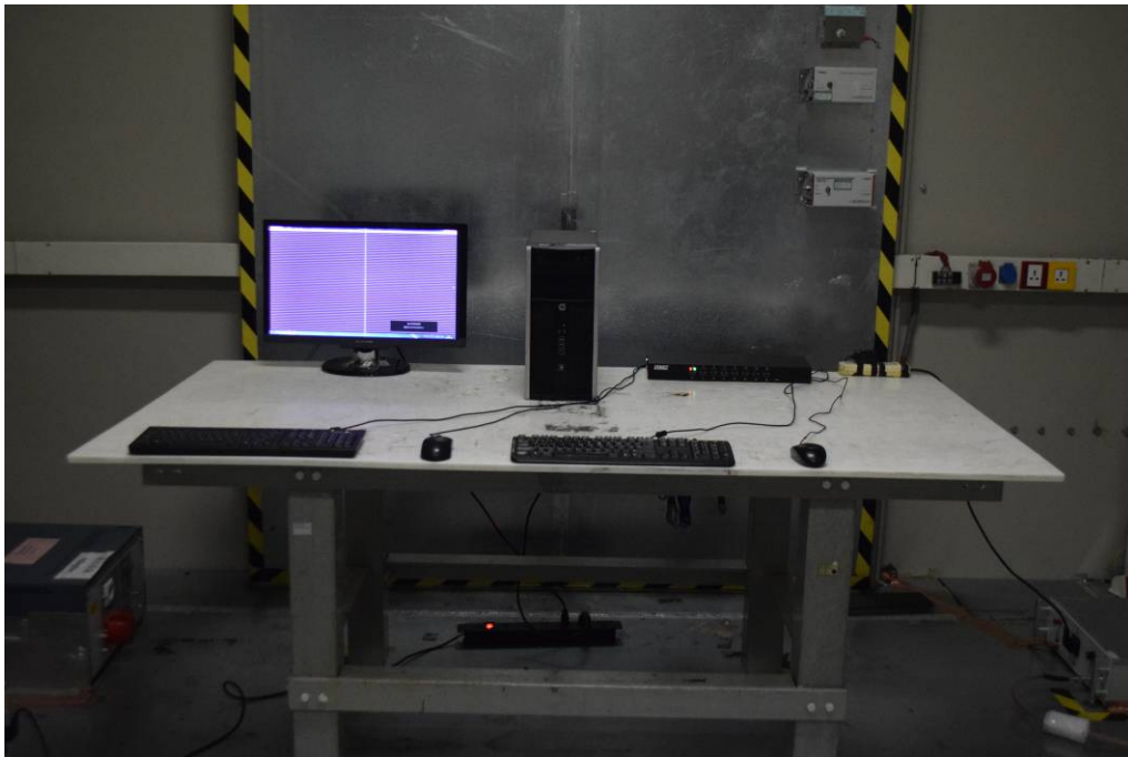
Front View of Conducted Emission Test
