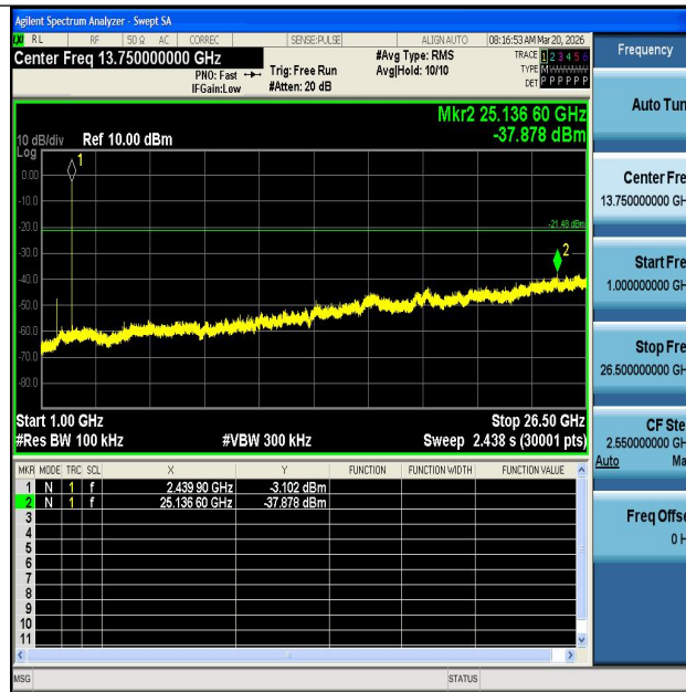
BLE_2M-Ant1-2440-1000~26500-PASS
