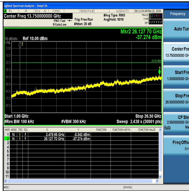
BLE_1M-Ant1-2480-1000~26500-PASS
