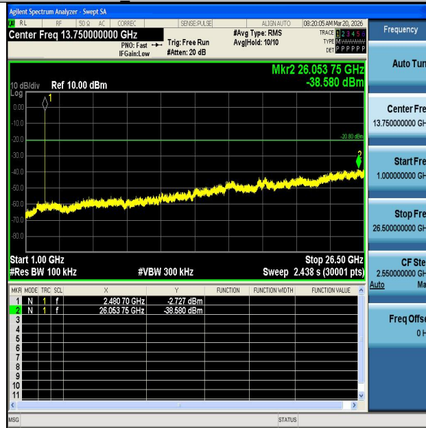
BLE_2M-Ant1-2480-1000~26500-PASS
