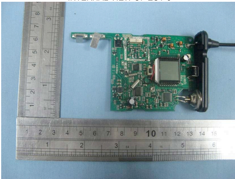
INTERNAL VIEW OF EUT-3
