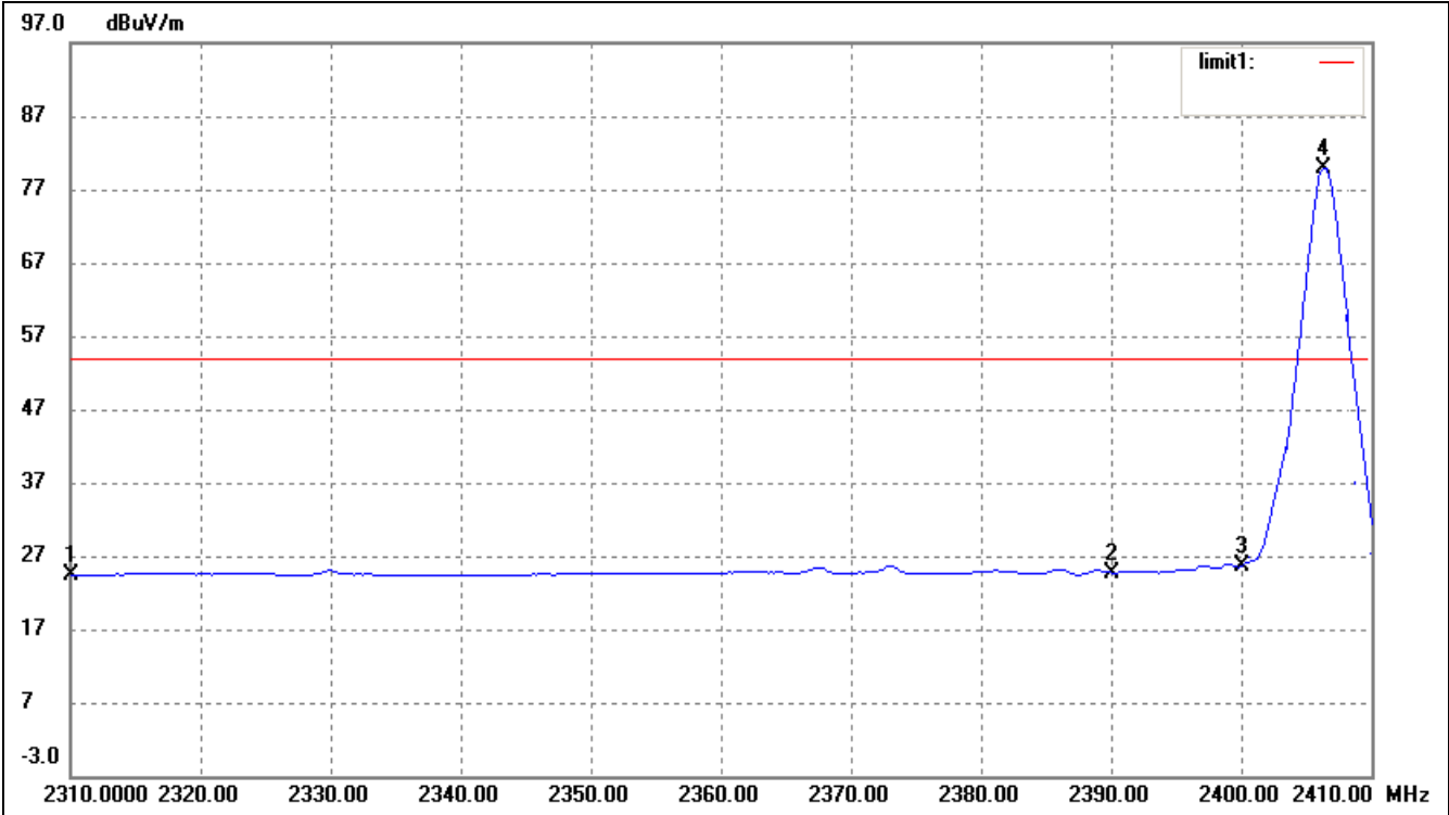
Lowest Bandedge
