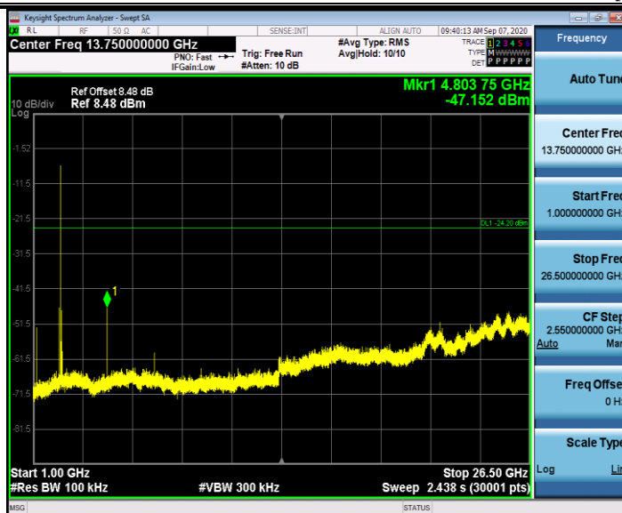
BLE_BT5.0_Ant1_2440_0-Reference
