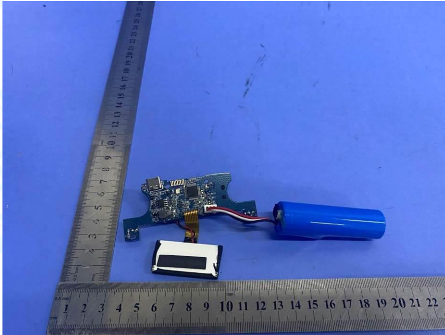
Photo 12 Internal of Battery
