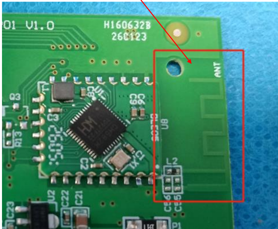
View of wireless antenna
