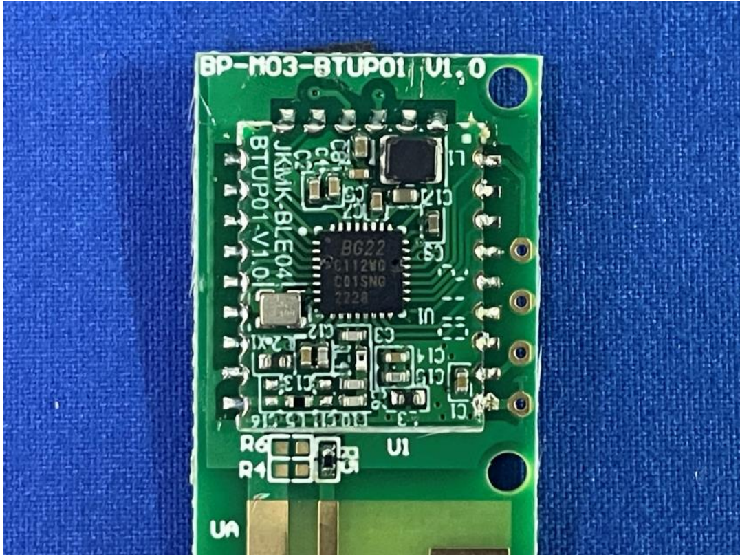
Photo 11: Internal View for PCB
