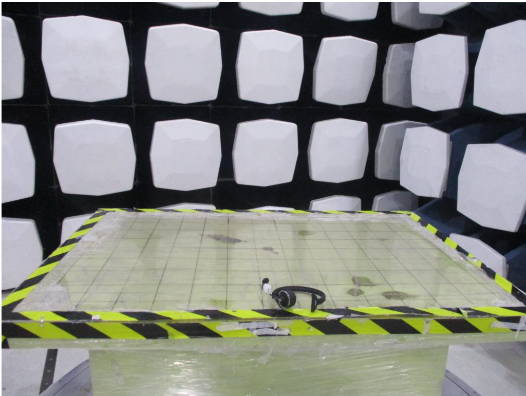
The EuT is placed at the center of turntable Below 1GHz
