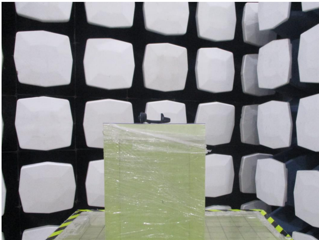
The EuT is placed at the center of turntable Above 1GHz
