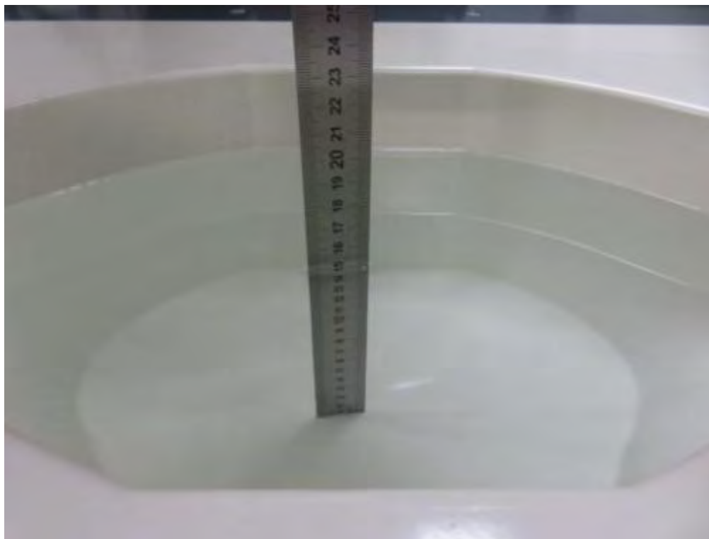
Photograph of the depth in the Body Phantom (2450MHz, 15.2cm depth)
