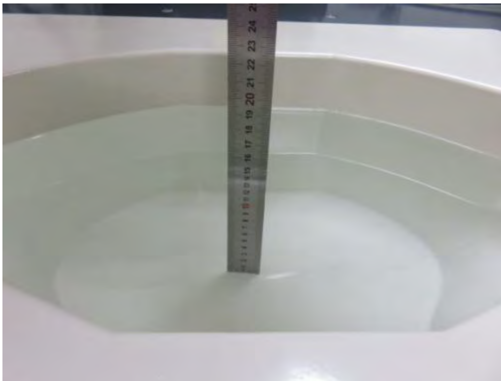
Photograph of the depth in the Body Phantom (750MHz, 15.2cm depth)
