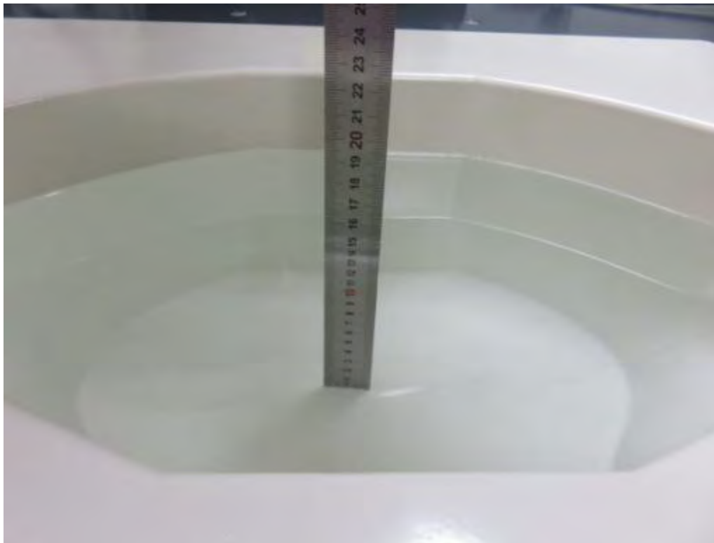
Photograph of the depth in the Body Phantom (1800MHz, 15.3cm depth)
