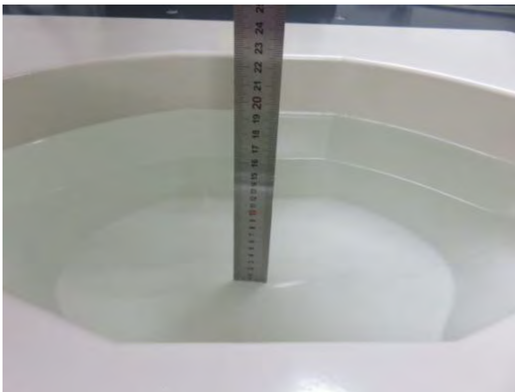
Photograph of the depth in the Body Phantom (1900MHz, 15.2cm depth)
