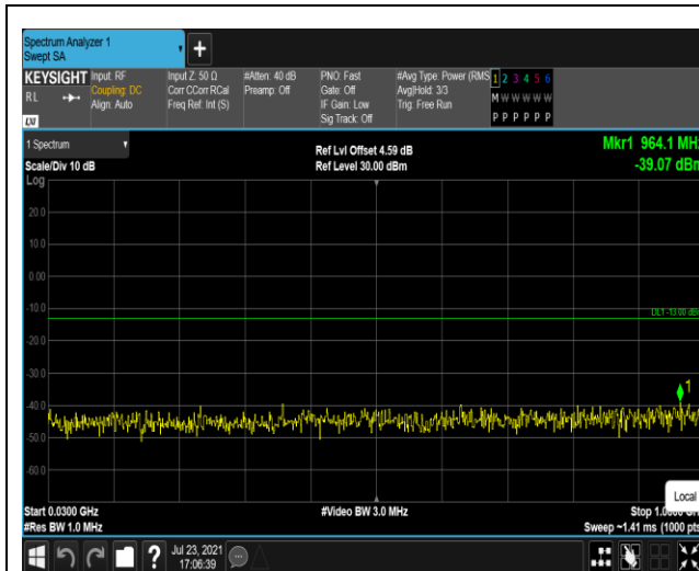
Band4-1.4MHz-16QAM-20393-1RB#0-Range1:30~1000MHz
