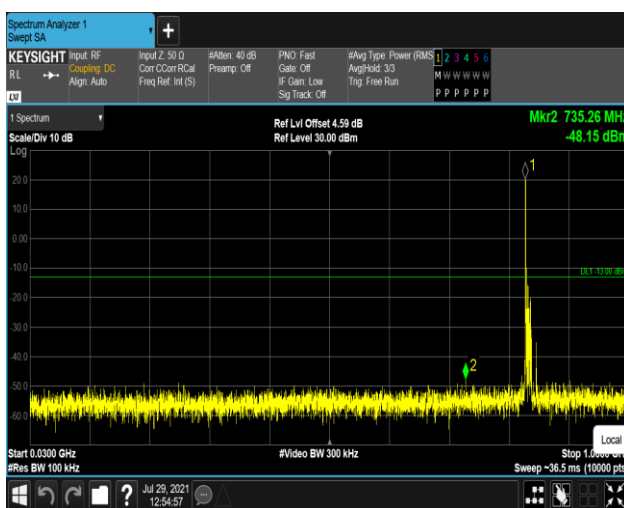
Band5-10MHz-QPSK-20525-1RB#0-Range1:30~1000MHz
