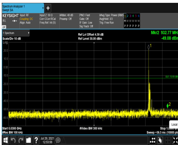
Band5-10MHz-QPSK-20450-1RB#0-Range1:30~1000MHz
