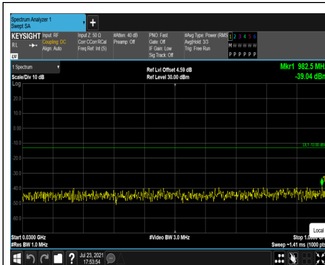
Band4-20MHz-16QAM-20175-1RB#0-Range1:30~1000MHz
