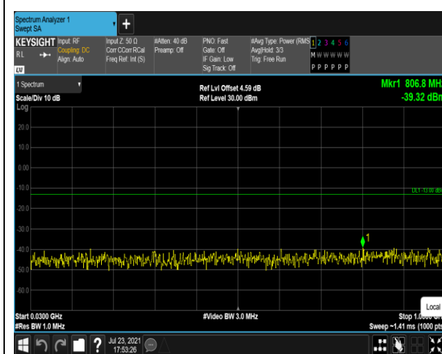
Band4-20MHz-QPSK-20050-1RB#0-Range1:30~1000MHz
