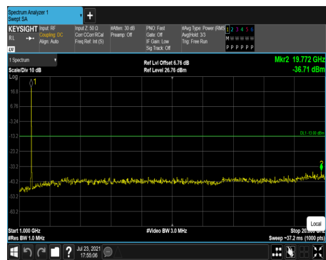
Band4-20MHz-16QAM-20300-1RB#0-Range2:1000~20000MHz
