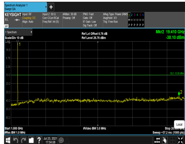
Band4-20MHz-16QAM-20175-1RB#0-Range2:1000~20000MHz
