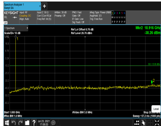
Band4-1.4MHz-16QAM-20393-1RB#0-Range2:1000~20000MHz
