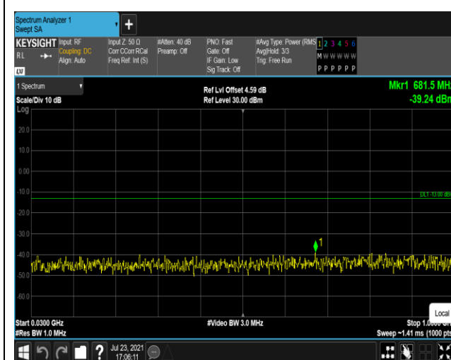
Band4-1.4MHz-QPSK-20175-1RB#0-Range1:30~1 000MHz
