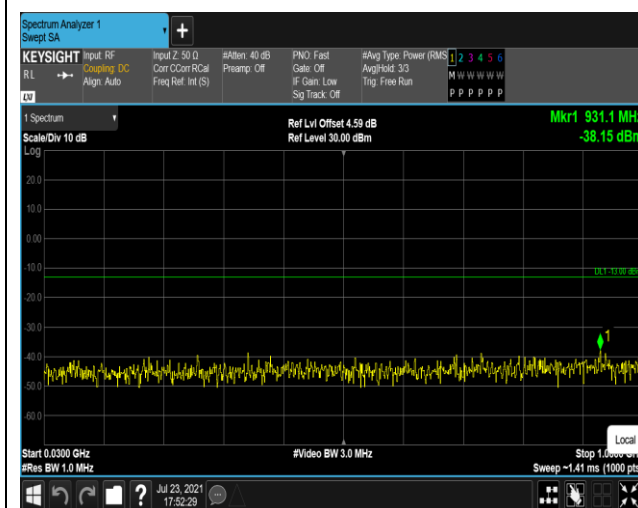
Band4-20MHz-QPSK-20050-1RB#0-Range1:30~1000MHz
