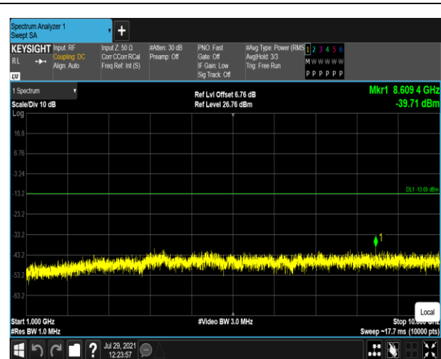
Band5-1.4MHz-16QAM-20407-1RB#0-Range2:1000~10000MHz
