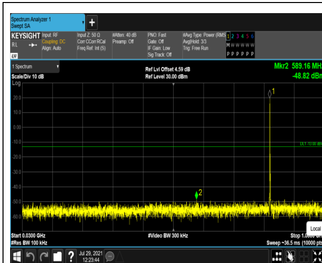
Band5-1.4MHz-16QAM-20407-1RB#0-Range1:30~1000MHz
