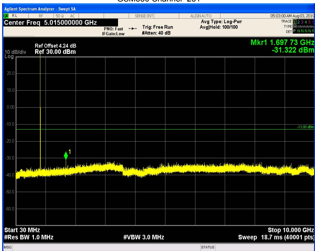
GSM850 Channel=251
