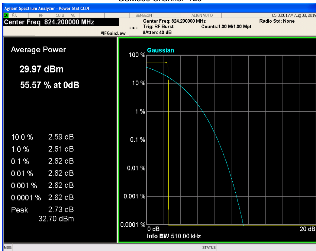
GSM850 Channel=128
