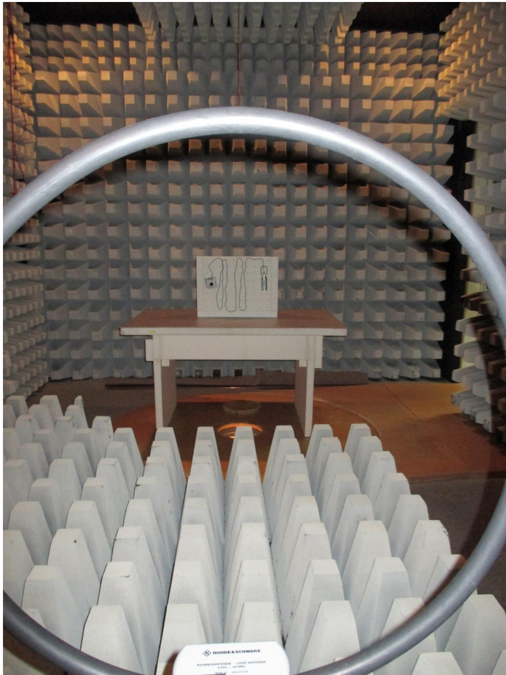
153494_X_U_G.JPG: ZONESCAN 820 Logger with integrated antenna, test setup fully anechoic chamber
