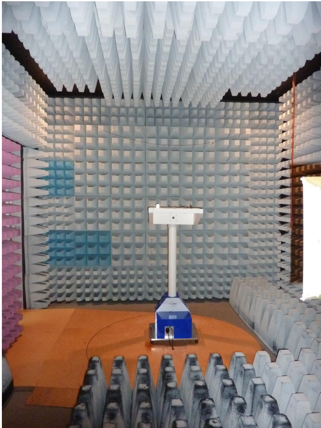
153494_X_U_P.JPG: ZONESCAN 820 Logger with external antenna, test setup fully anechoic chamber
