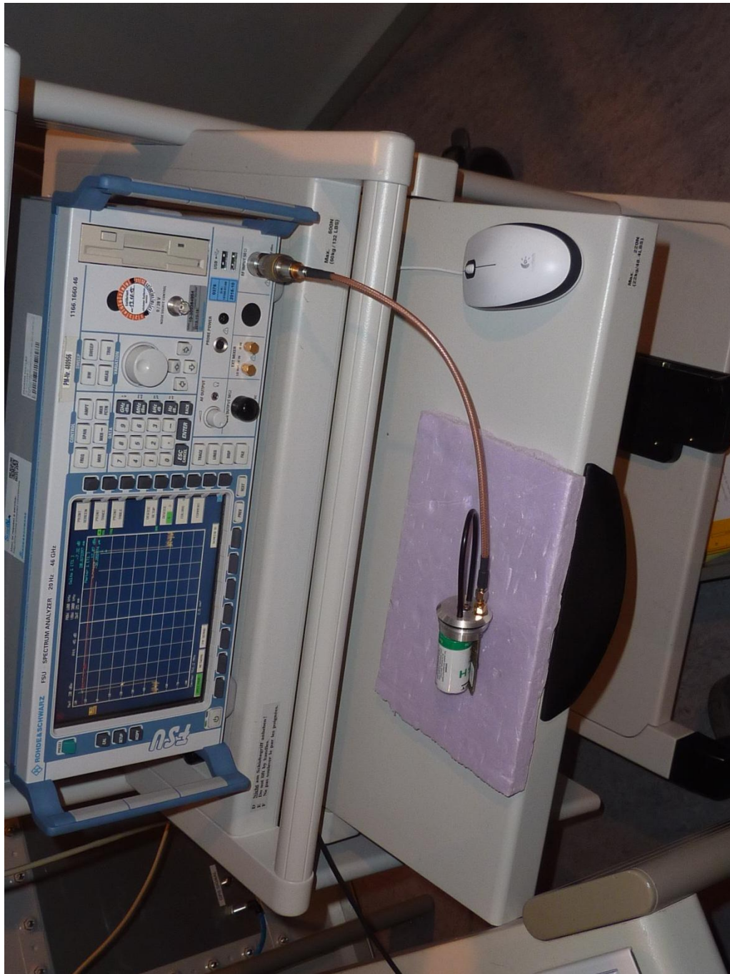
153494_X_U_R.JPG: ZONESCAN 820 Logger with external antenna, test setup conducted measurements
