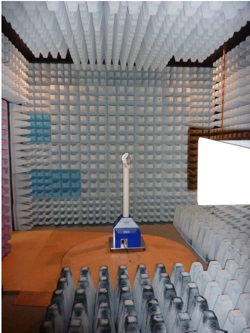
153494_E_U_E.JPG: EASYSCAN SENSOR, test setup fully anechoic chamber
