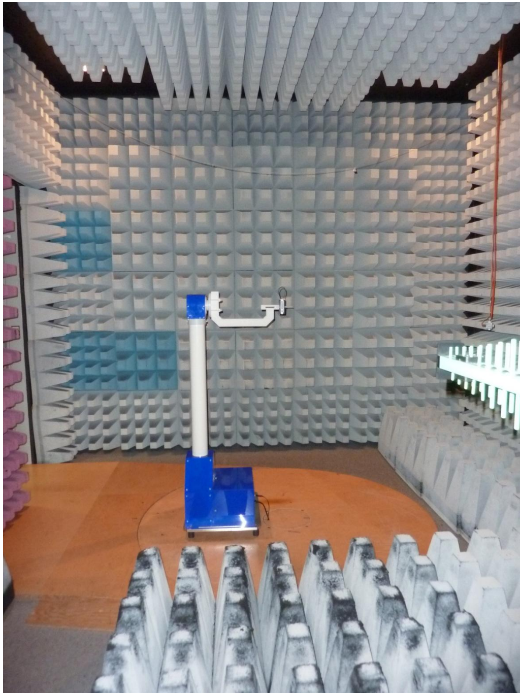
153494_I_U_I.JPG: ZONESCAN 820 Logger with integrated antenna, test setup fully anechoic chamber
