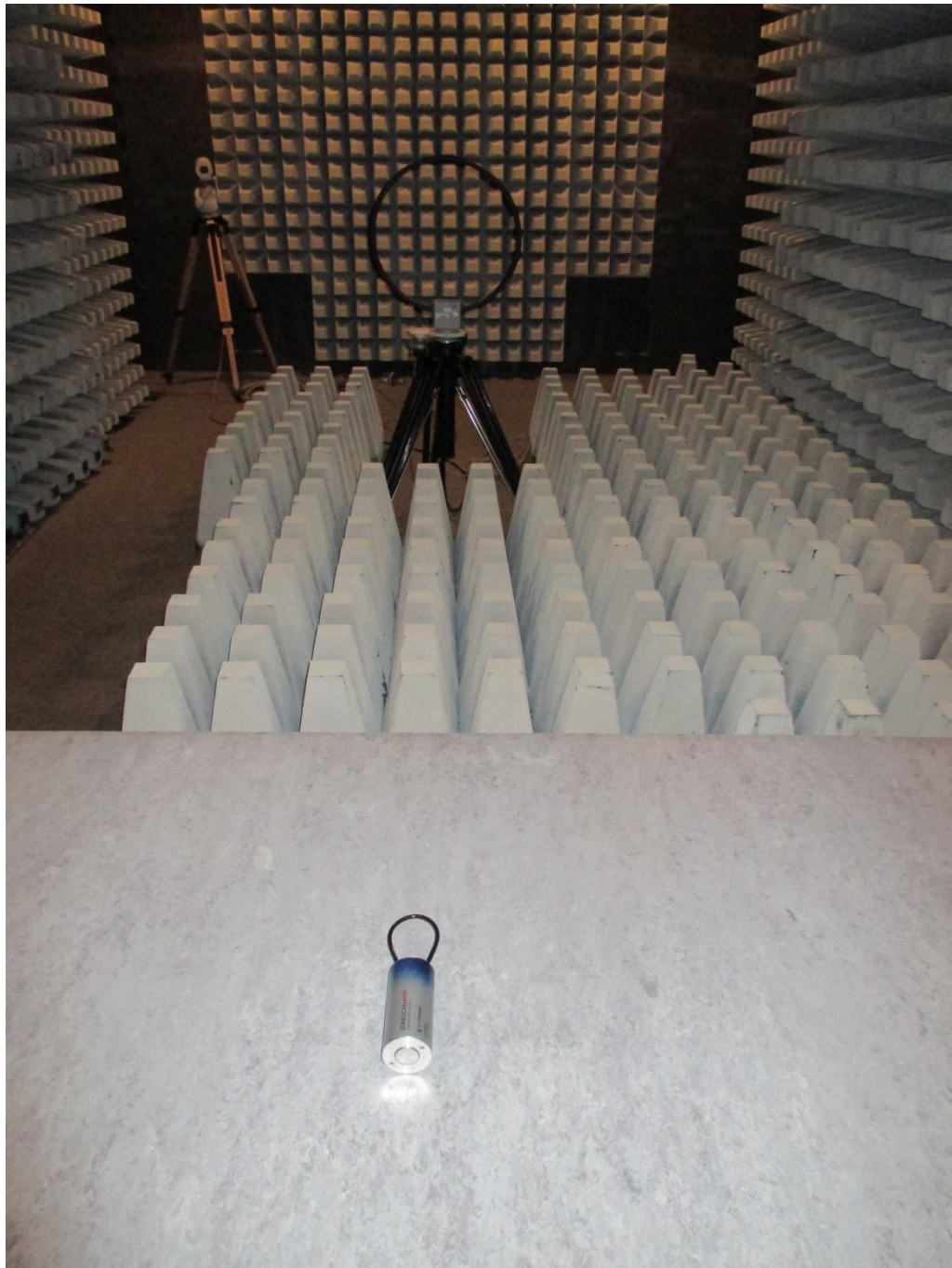
153494_I_U_G.JPG: ZONESCAN 820 Logger with integrated antenna, test setup fully anechoic chamber
