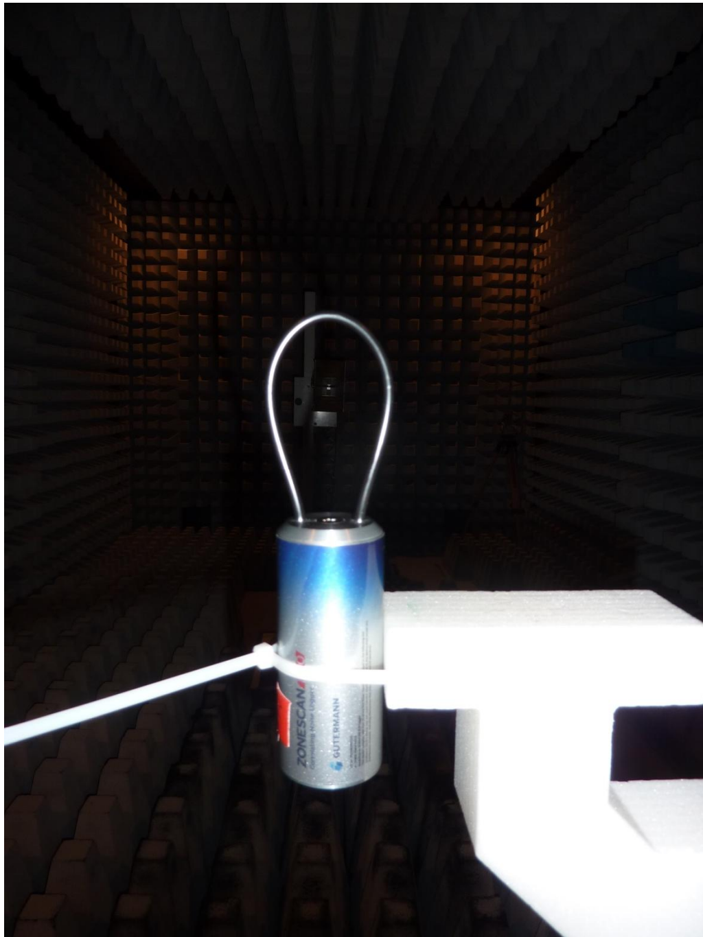
153494_I_U_A.JPG: ZONESCAN 820 Logger with integrated antenna, test setup fully anechoic chamber
