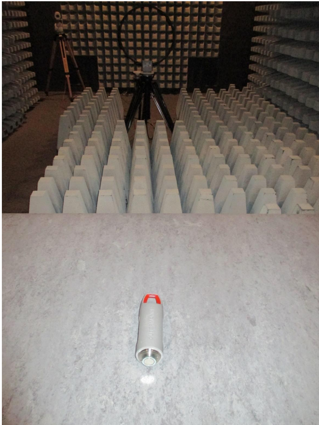
153494_E_U_G.JPG: EASYSCAN SENSOR, test setup fully anechoic chamber
