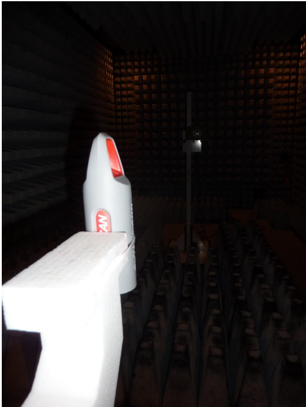
153494_E_U_C.JPG: EASYSCAN SENSOR, test setup fully anechoic chamber
