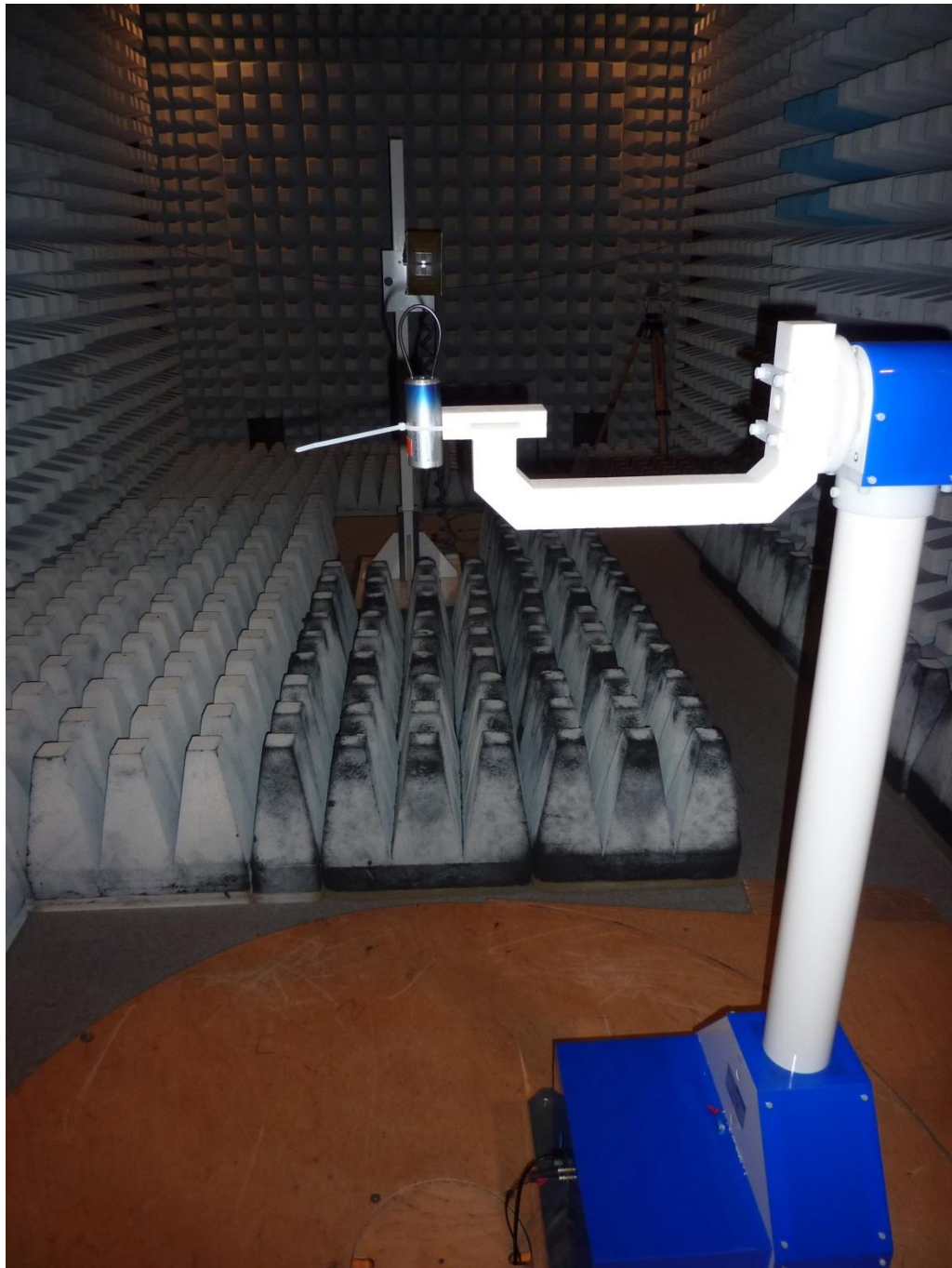
153494_I_U_B.JPG: ZONESCAN 820 Logger with integrated antenna, test setup fully anechoic chamber
