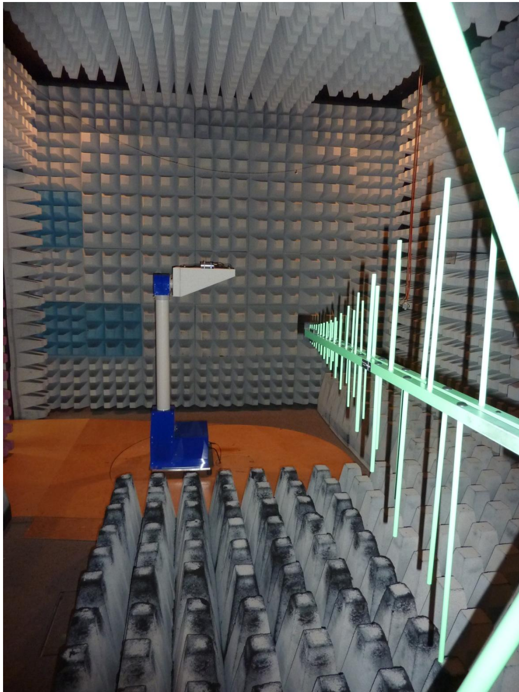
153494_X_U_L.JPG: ZONESCAN 820 Logger with external antenna, test setup fully anechoic chamber
