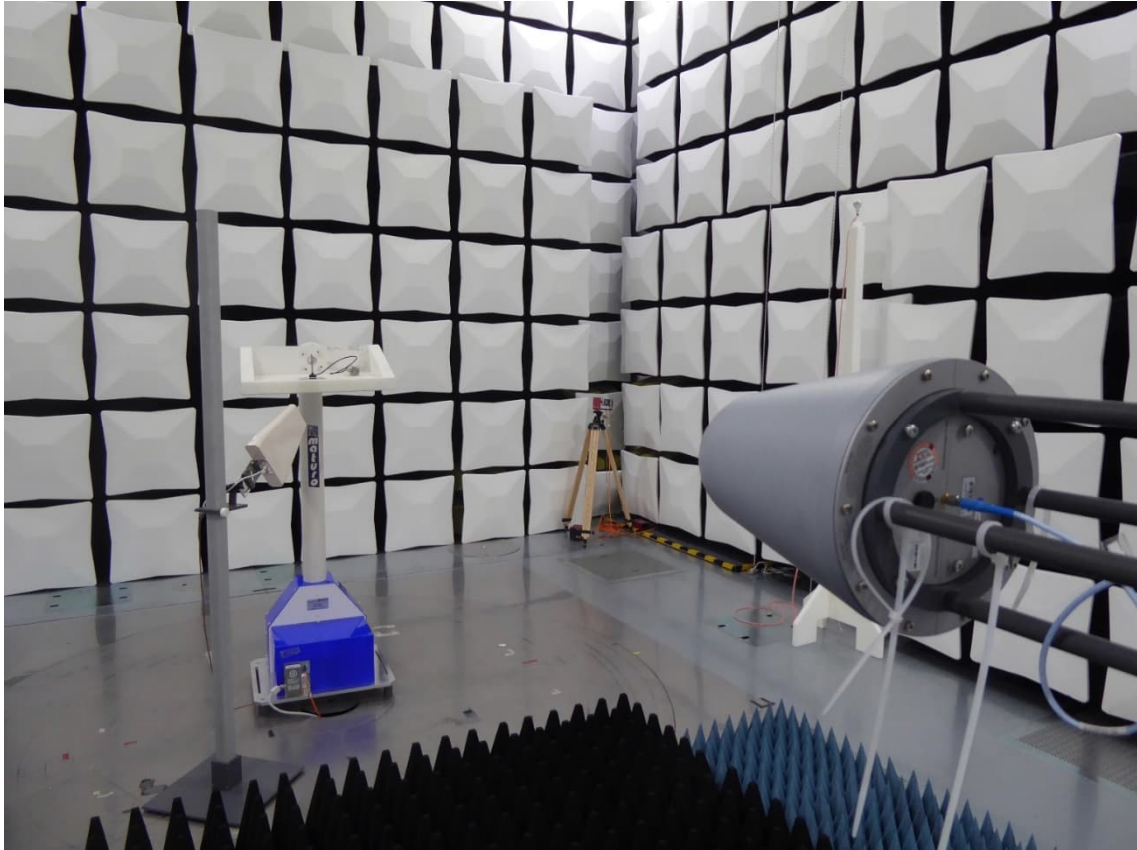
Test setup from 1 to 4 GHz
