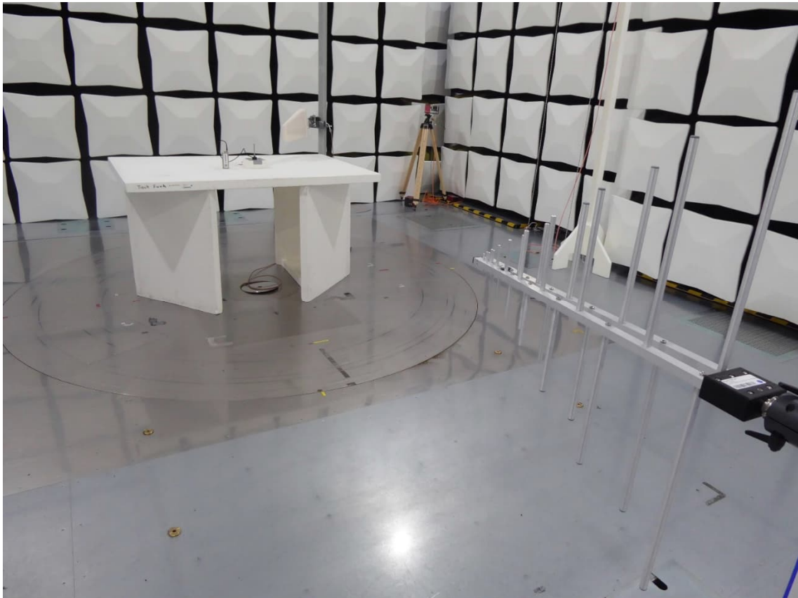
Test setup from 200 to 1000 MHz
