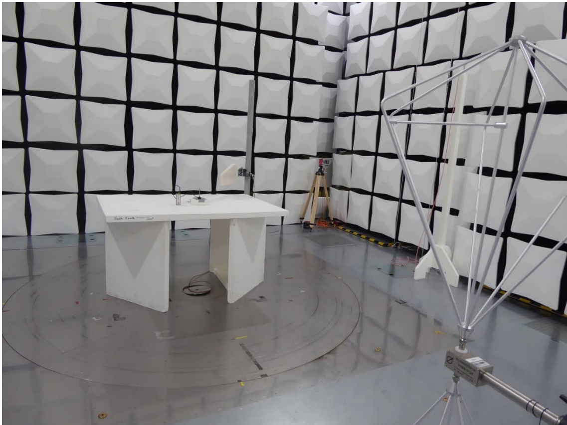
Test setup from 30 to 200 MHz
