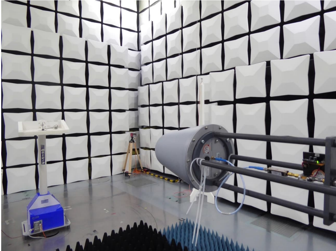
Test setup from 4 to 18 GHz
