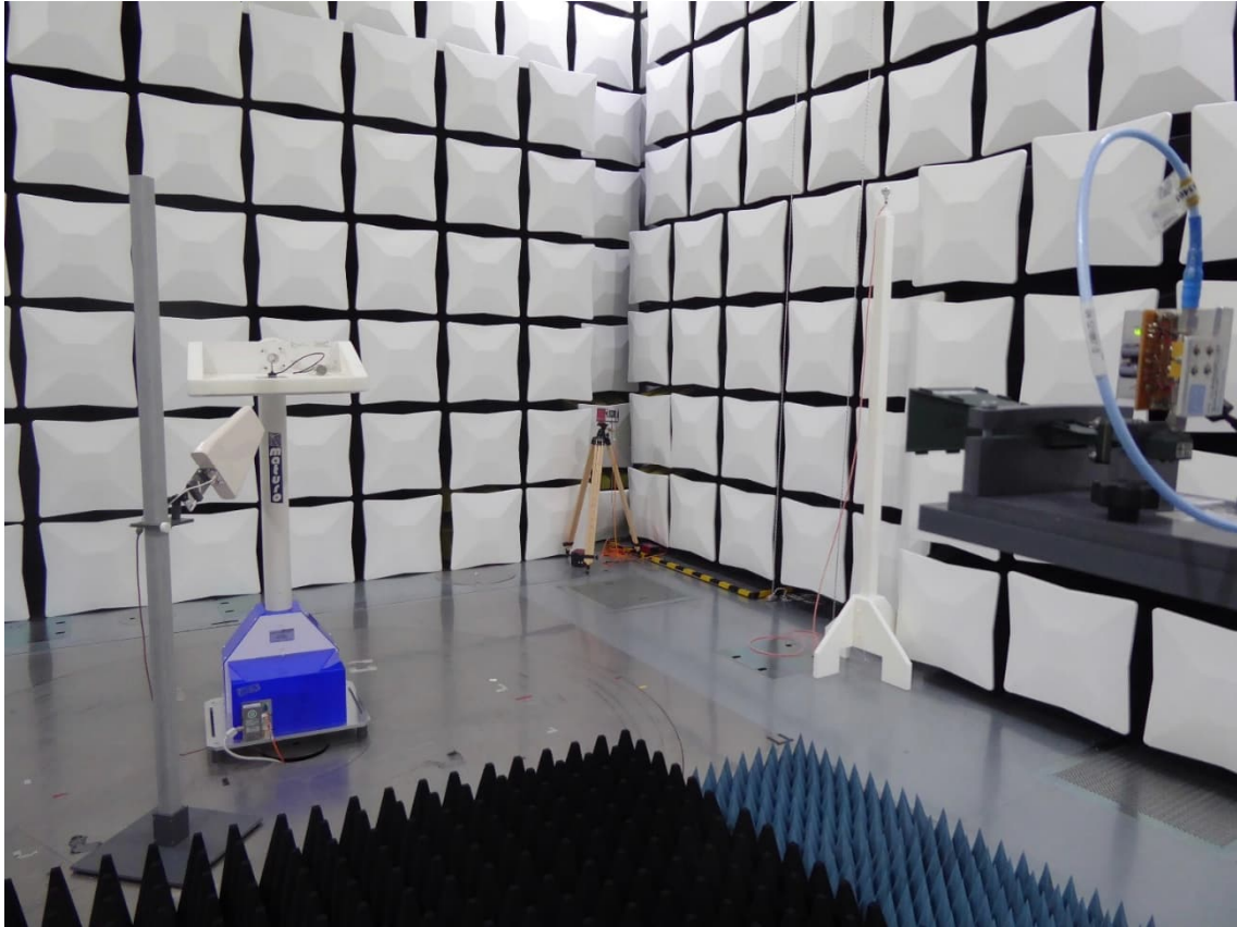
Test setup from 18 to 26.5 GHz
