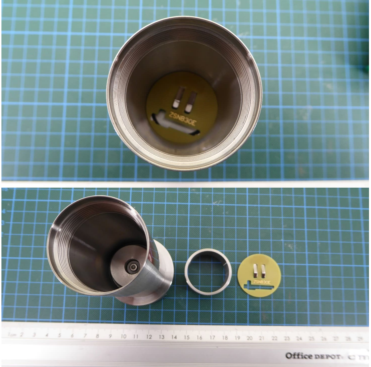
EUT – housing
