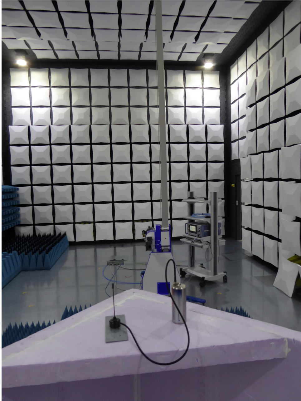
Test Setup SAC from 18 GHz to 20 GHz
