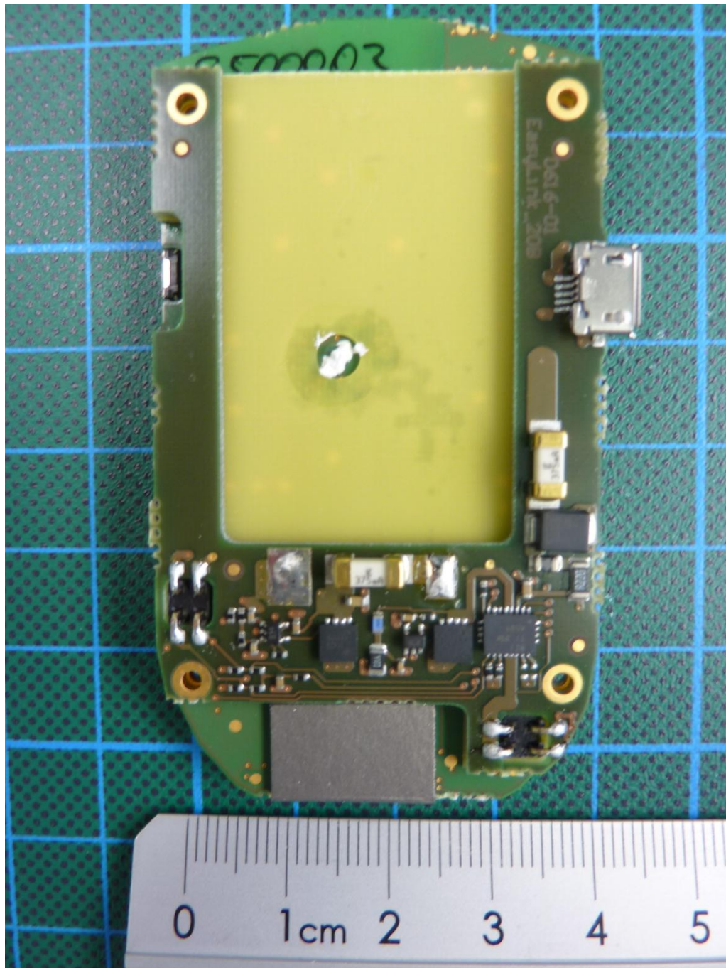
170032_6.JPG: EASYSCAN Link, PCB sandwich, battery removed
