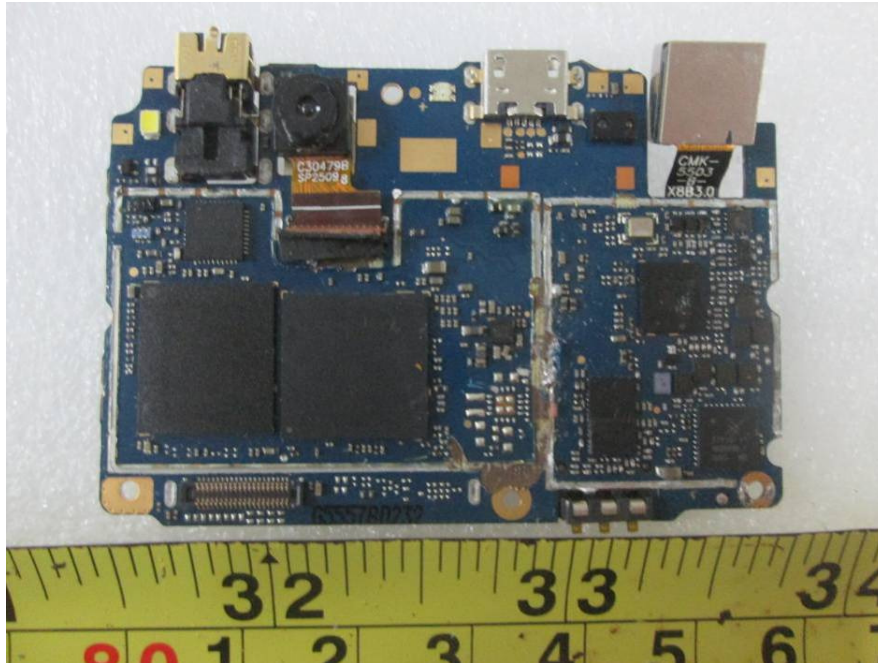
EUT – Main Baord 1 Top Shielding off View
