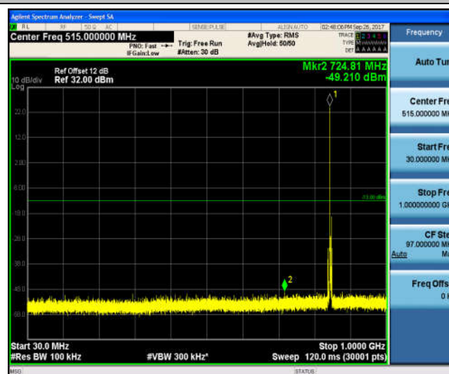
Band5_3MHz_16QAM_20635_1RB#0_Range2:1000~26000MHz_-30.5_PASS
