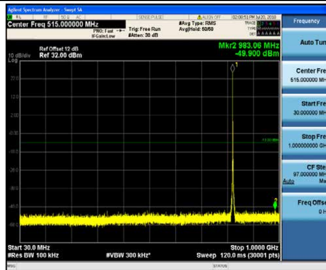
Band5_1.4MHz_16QAM_20415_1RB#0
