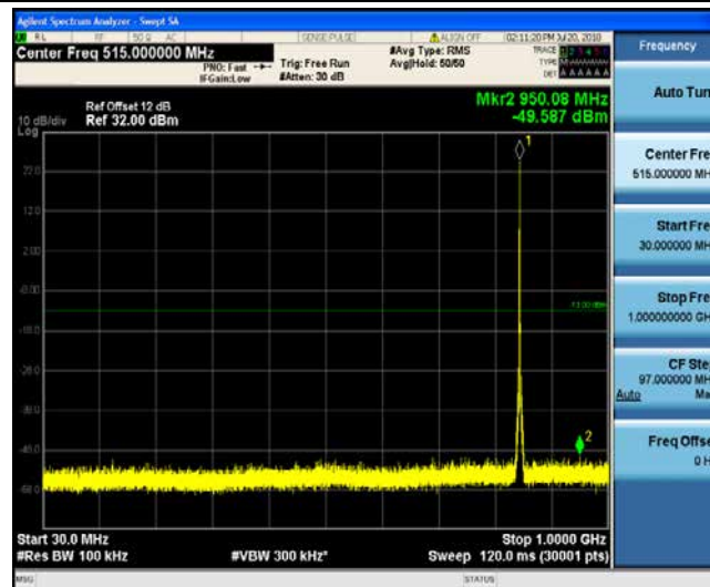
Band5_1.4MHz_16QAM_20635_1RB#0
