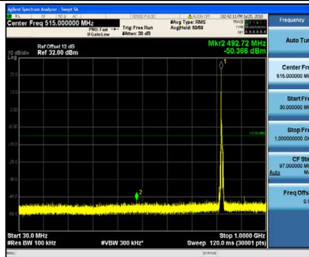
Band5_5MHz_16QAM_20415_1RB#0
