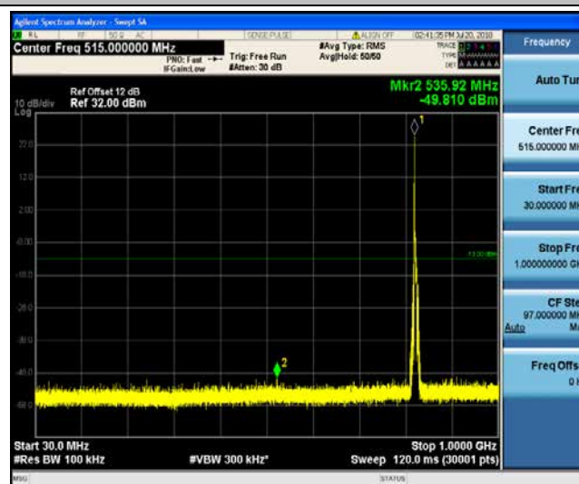
Band5_5MHz_QPSK_20415_1RB#0
