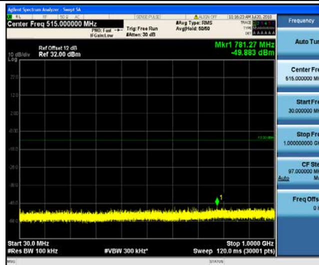
Band4_10MHz_16QAM_20385_1RB#0
