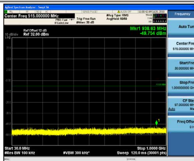
Band4_5MHz_16QAM_20385_1RB#0
