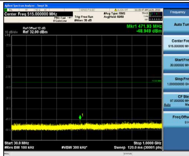
Band4_10MHz_QPSK_20385_1RB#0
