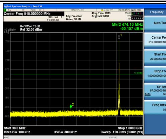
Band5_1.4MHz_QPSK_20415_1RB#0
