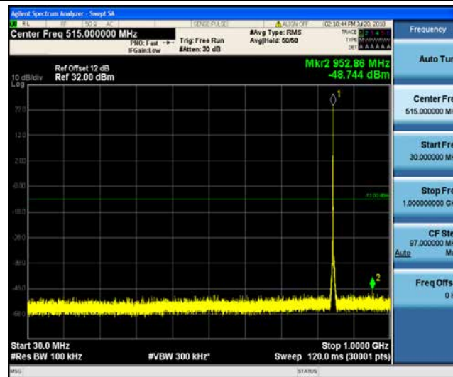
Band5_1.4MHz_QPSK_20635_1RB#0
