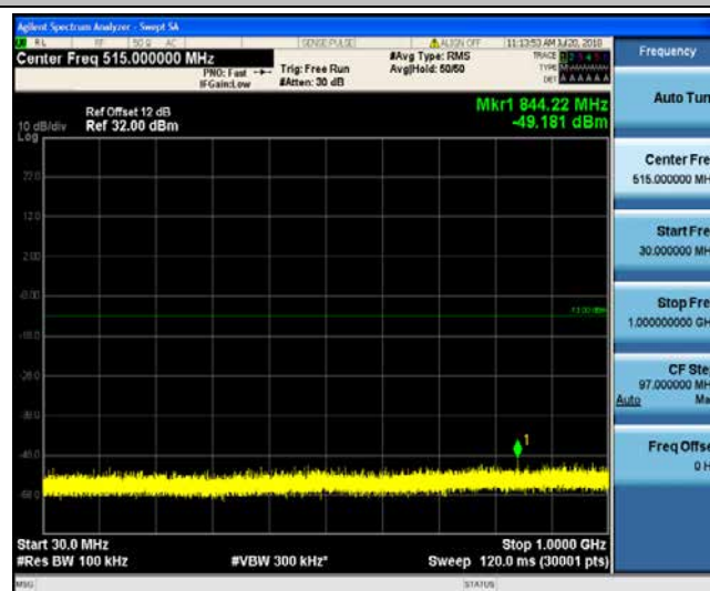
Band4_10MHz_16QAM_19965_1RB#0
