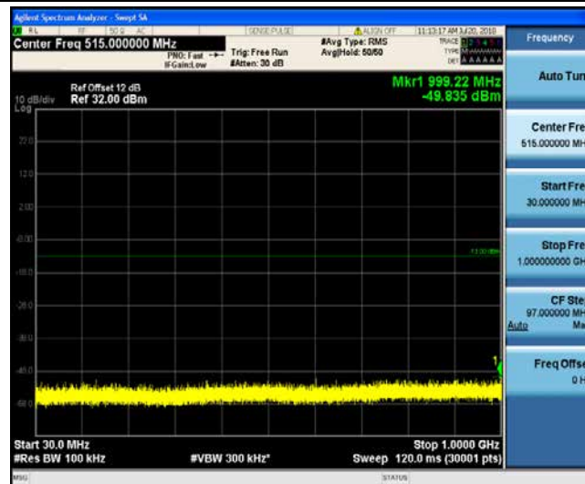
Band4_10MHz_QPSK_19965_1RB#0
