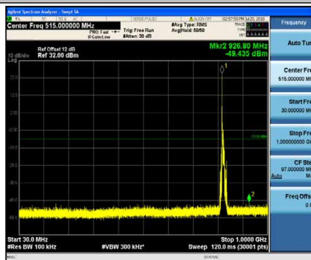
Band5_10MHz_16QAM_20415_1RB#0
