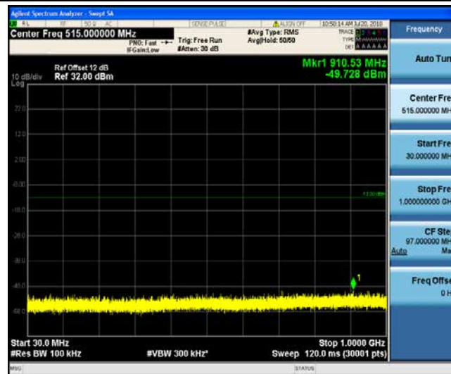
Band4_5MHz_16QAM_19965_1RB#0
