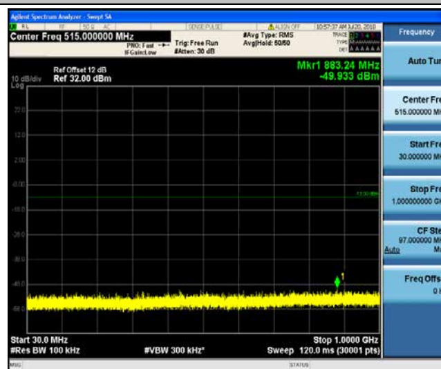
Band4_5MHz_QPSK_19965_1RB#0
