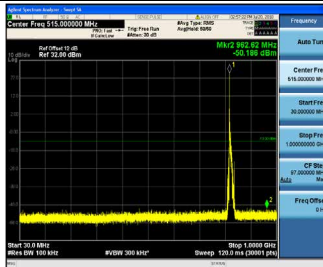
Band5_10MHz_QPSK_20415_1RB#0
