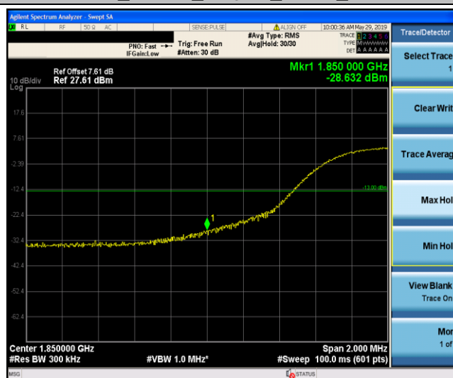
Band2 15MHz 16QAM 18675 75RB#0
