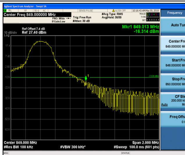
Band5_10MHz_QPSK_20600_1RB#49
