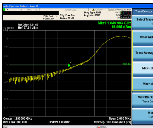
Band2 15MHz 16QAM 18675 1RB#0
