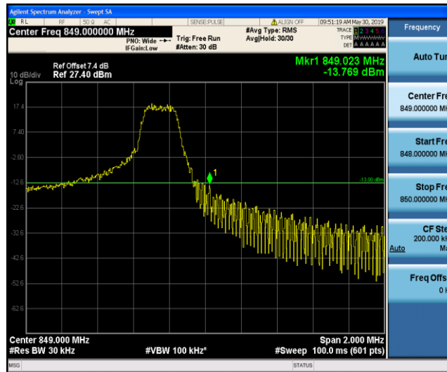
Band5_1.4MHz_16QAM_20643_1RB#5
