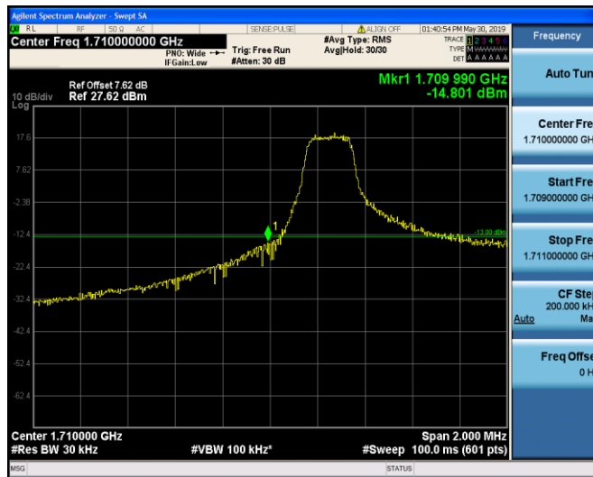
Band4_1.4MHz_QPSK_19957_1RB#0
