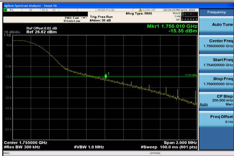
Band4-15MHz-QPSK-20325-1RB#74
