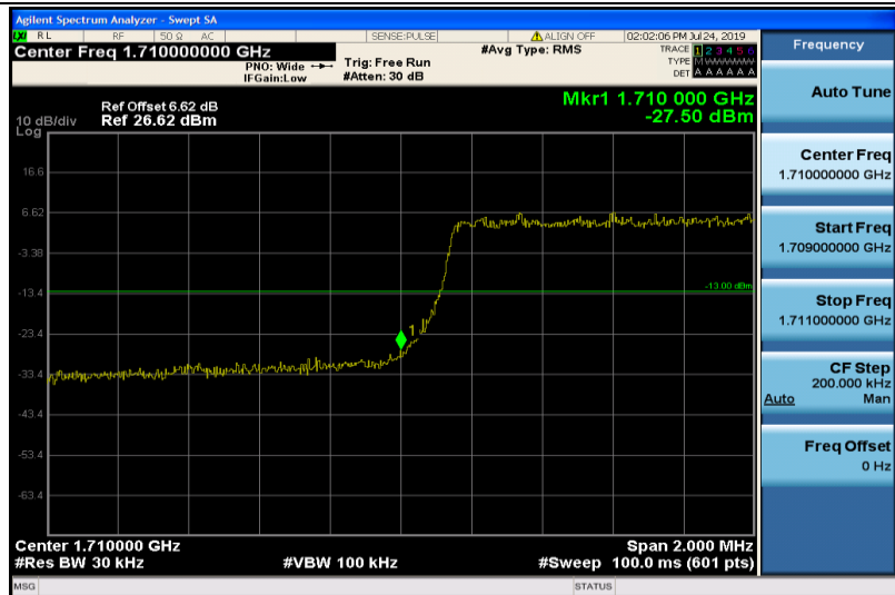
Band4-3MHz-QPSK-19965-15RB#0
