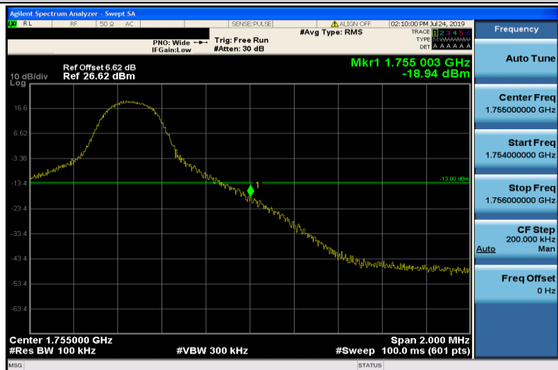
Band4-5MHz-16QAM-20375-1RB#24
