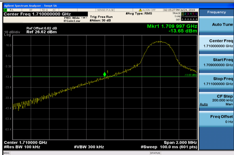
Band4-10MHz-16QAM-20000-1RB#0
