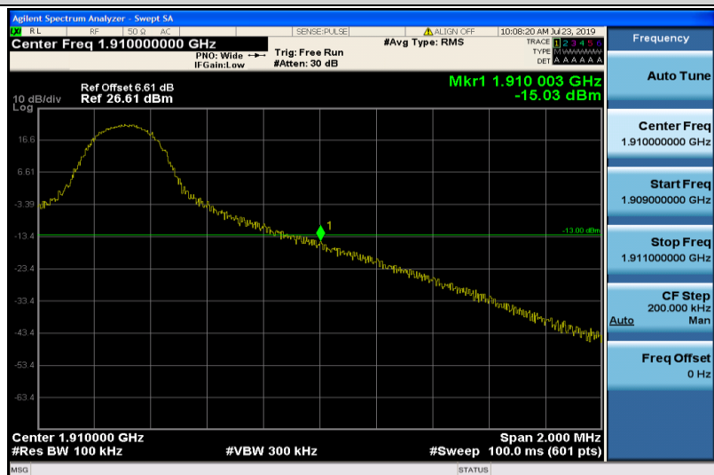
Band2-10MHz-QPSK-19150-1RB#49
