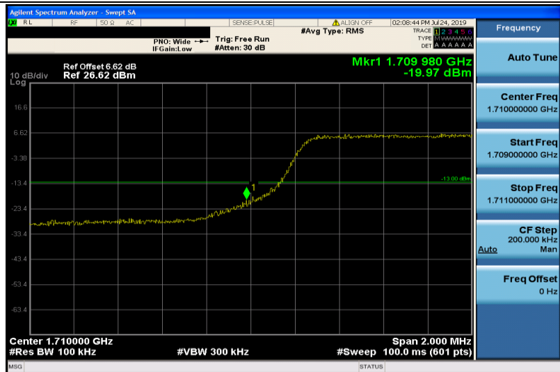
Band4-5MHz-16QAM-19975-25RB#0
