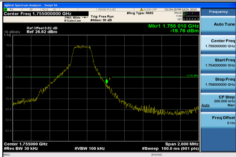
Band4-1.4MHz-16QAM-20393-1RB#5
