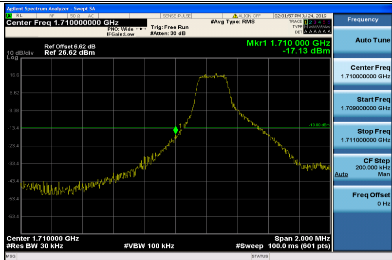
Band4-3MHz-16QAM-19965-1RB#0
