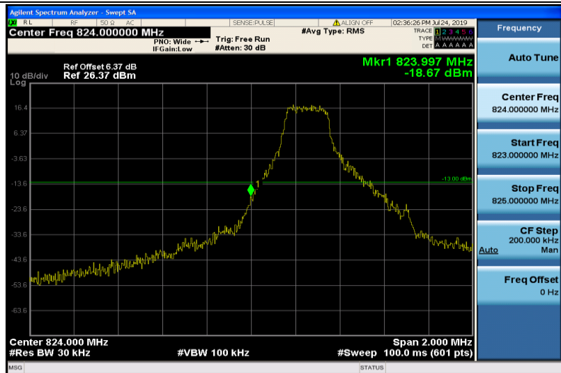
Band5-1.4MHz-QPSK-20407-1RB#0
