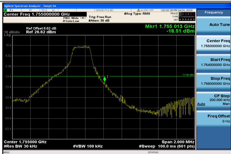
Band4-3MHz-16QAM-20385-1RB#14
