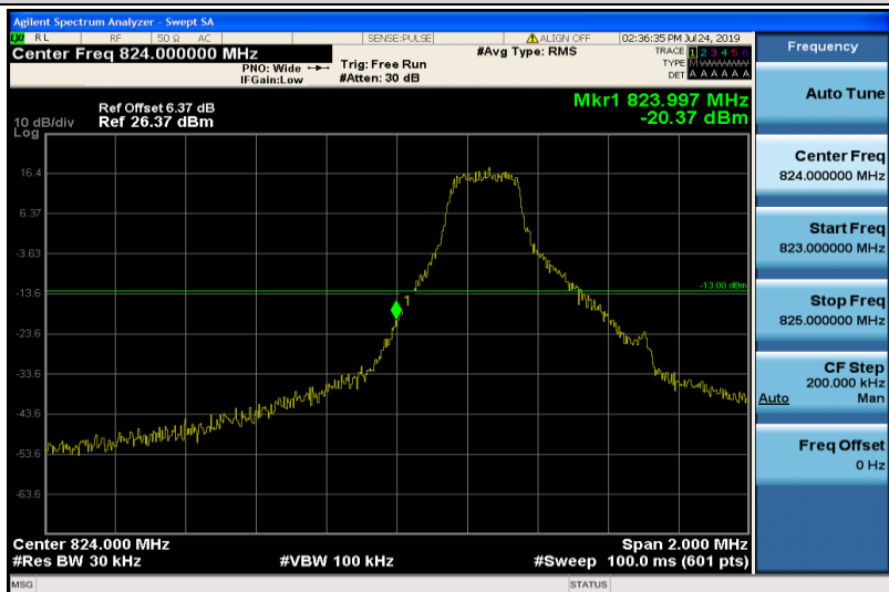
Band5-1.4MHz-16QAM-20407-1RB#0
