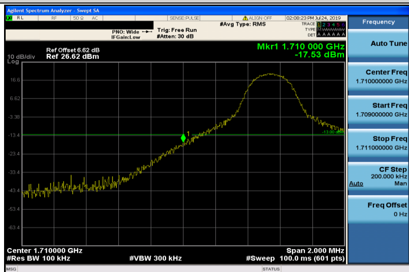
Band4-5MHz-16QAM-19975-1RB#0
