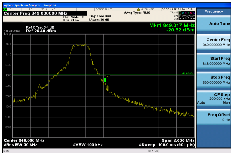
Band5-1.4MHz-16QAM-20643-1RB#5
