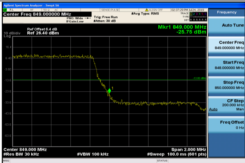
Band5-1.4MHz-QPSK-20643-6RB#0
