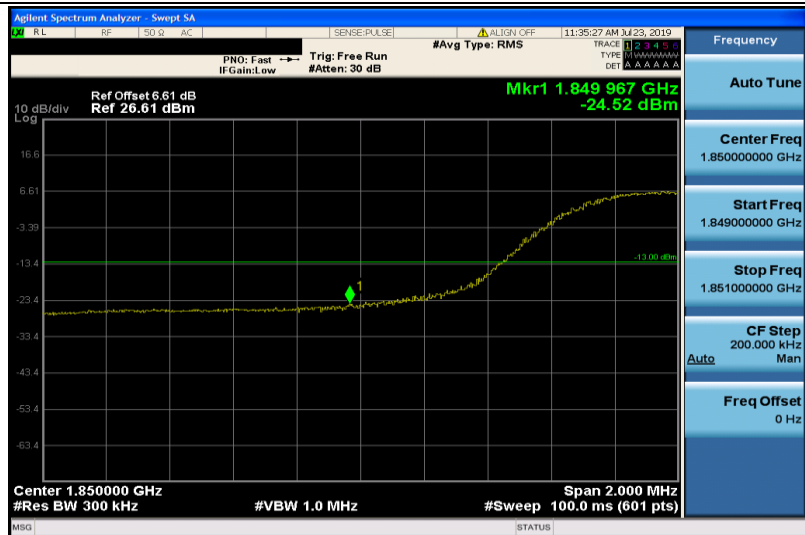
Band2-15MHz-QPSK-18675-75RB#0
