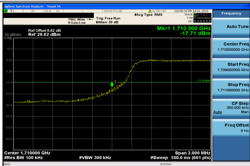
Band4-5MHz-QPSK-19975-25RB#0
