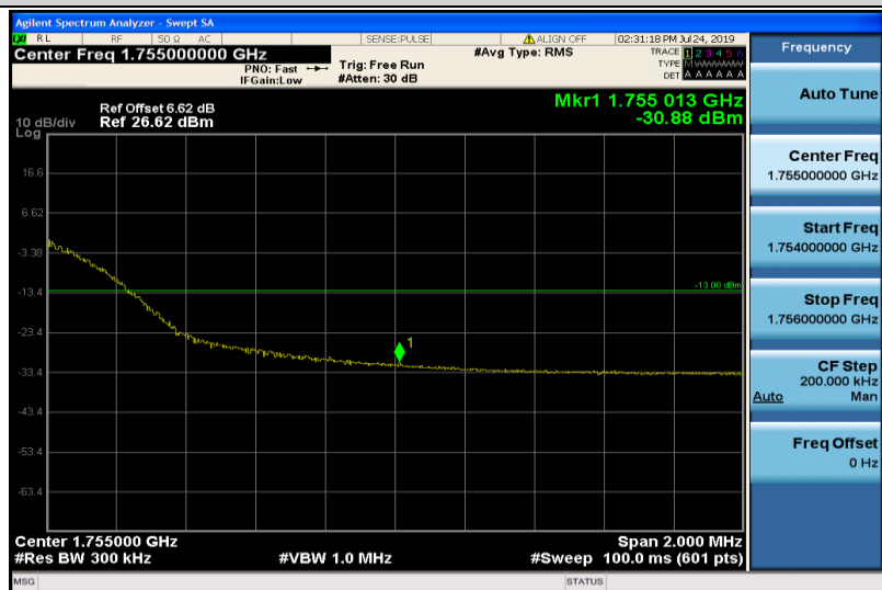
Band4-20MHz-16QAM-20300-100RB#0
