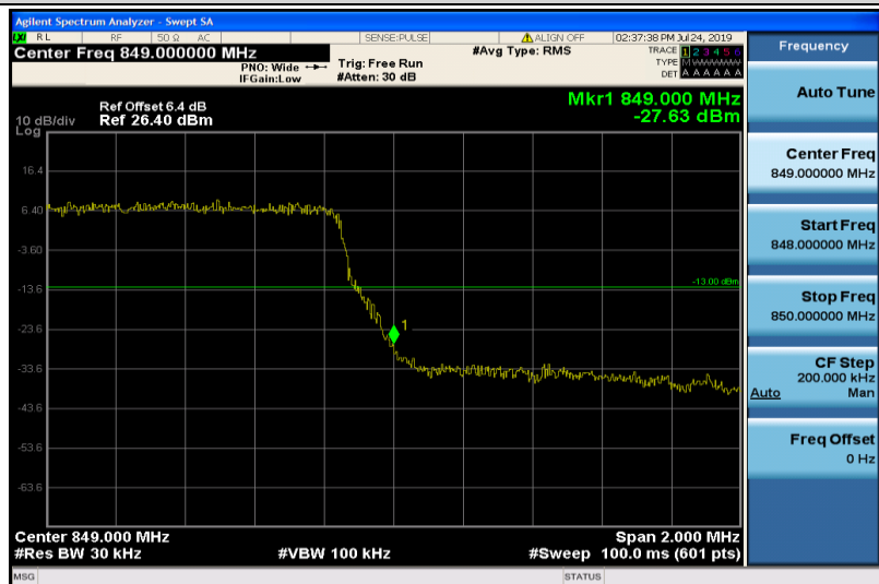
Band5-1.4MHz-16QAM-20643-6RB#0
