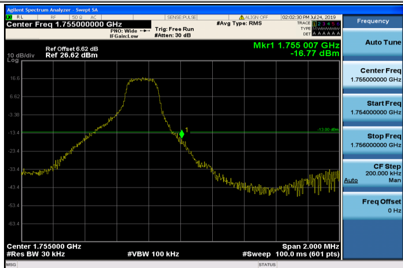
Band4-3MHz-QPSK-20385-1RB#14
