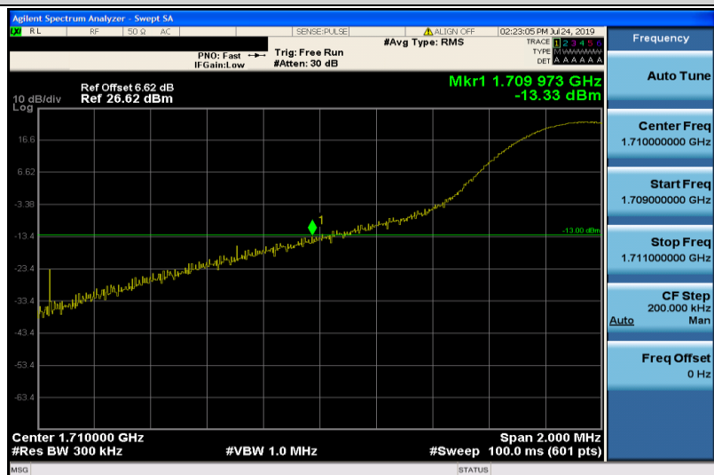
Band4-15MHz-QPSK-20025-1RB#0
