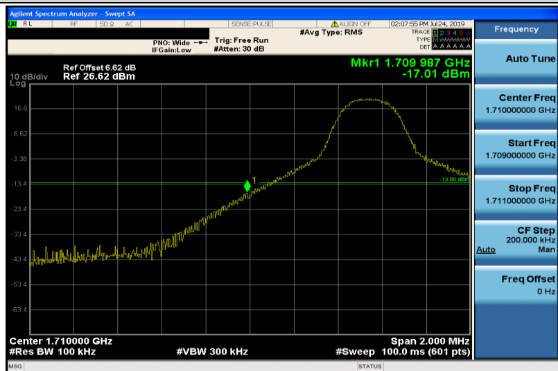
Band4-5MHz-QPSK-19975-1RB#0
