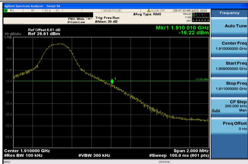
Band2-5MHz-16QAM-19175-1RB#24
