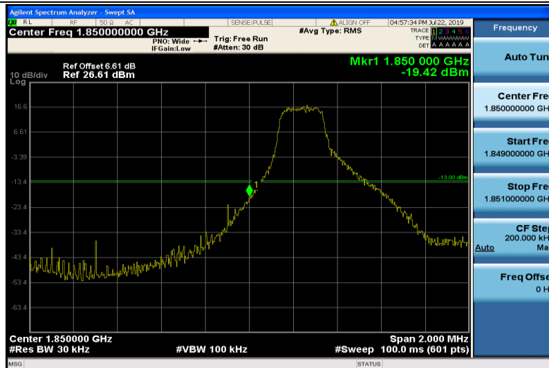
Band2-3MHz-16QAM-18615-1RB#0
