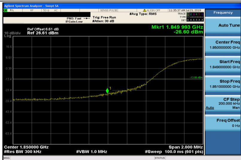
Band2-15MHz-16QAM-18675-75RB#0
