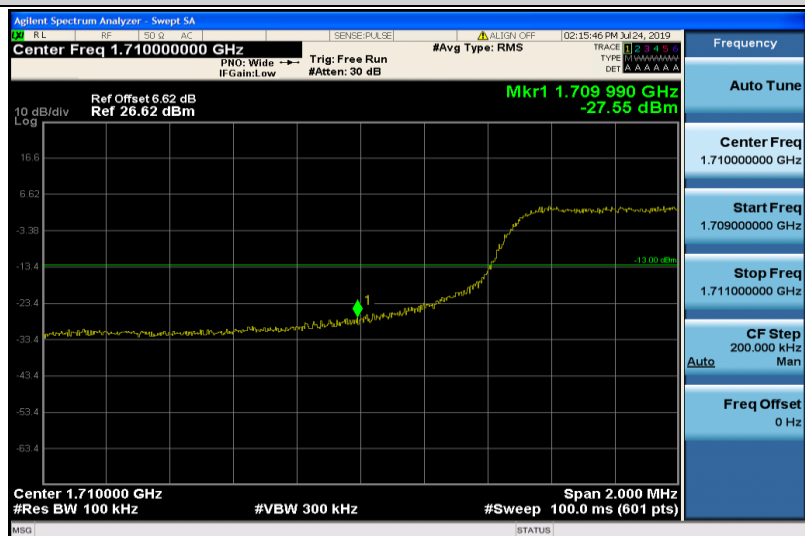
Band4-10MHz-16QAM-20000-50RB#0
