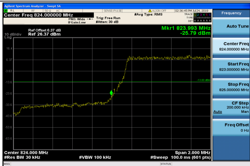
Band5-1.4MHz-QPSK-20407-6RB#0
