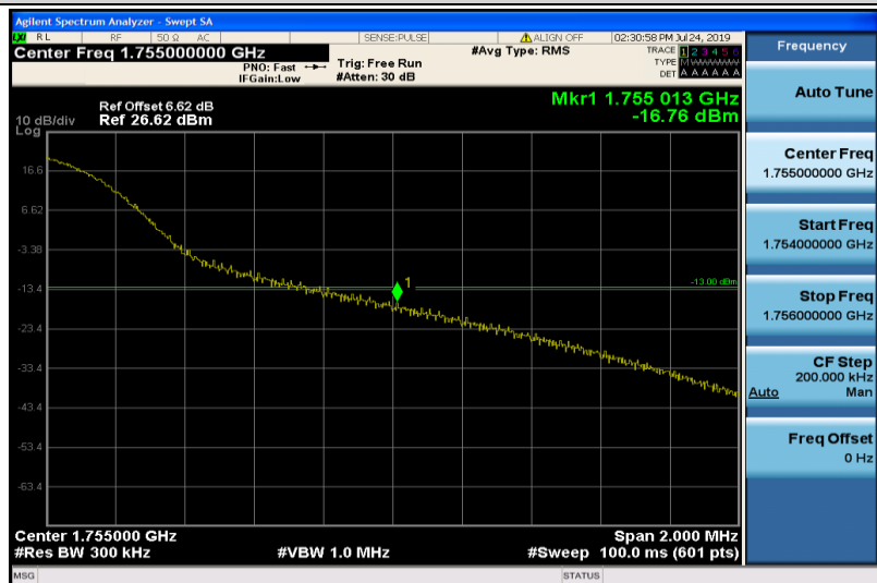
Band4-20MHz-16QAM-20300-1RB#99
