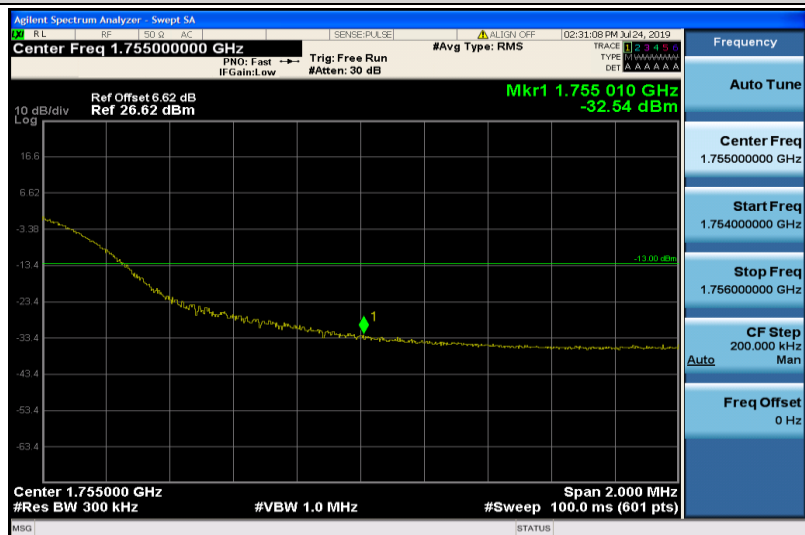
Band4-20MHz-QPSK-20300-100RB#0
