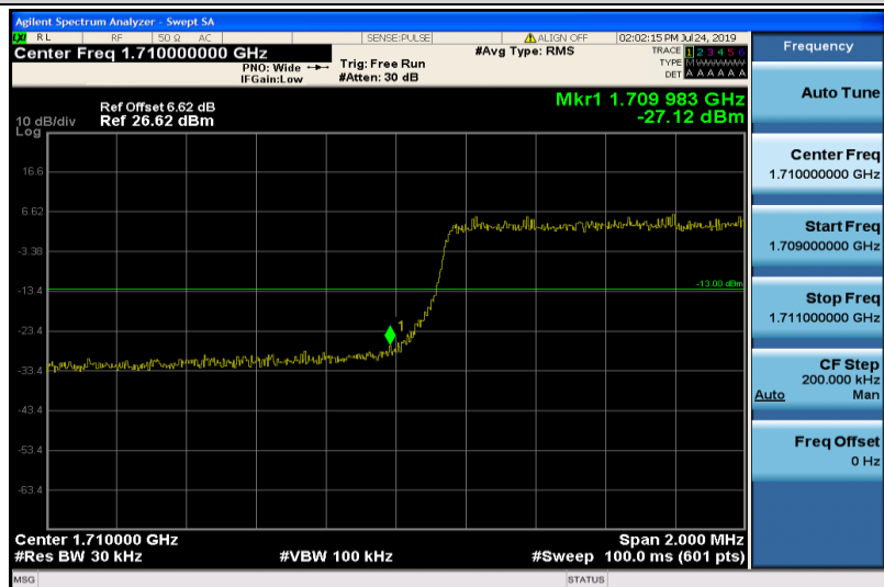
Band4-3MHz-16QAM-19965-15RB#0
