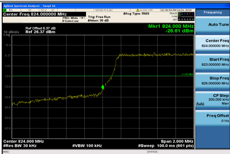
Band5-1.4MHz-16QAM-20407-6RB#0
