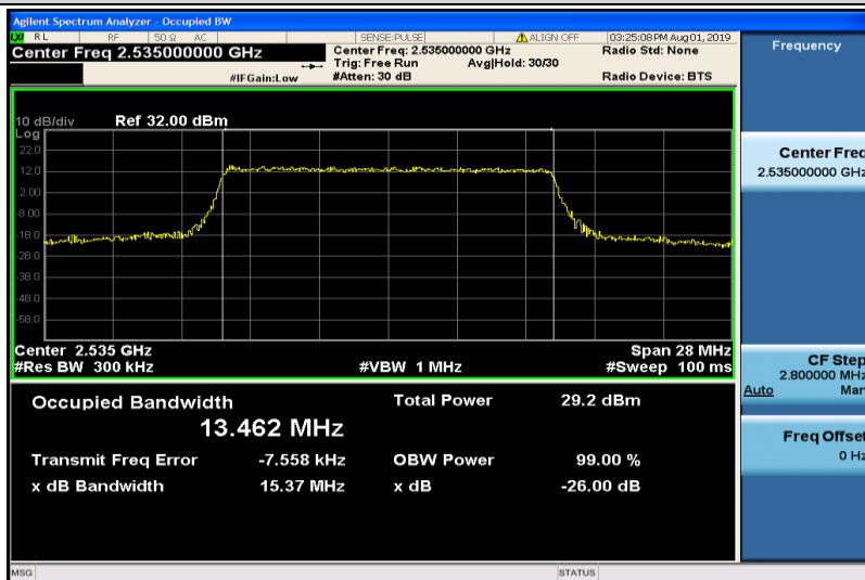
Band7-15MHz-QPSK-21100-75RB#0-13.462
