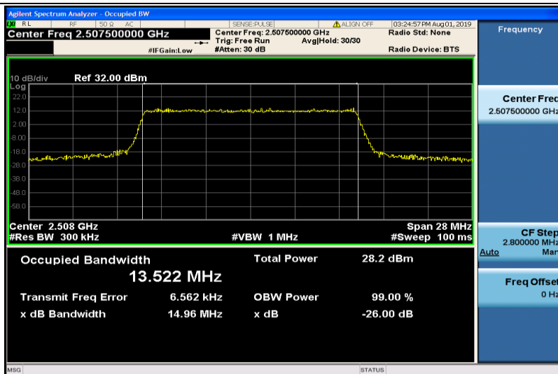
Band7-15MHz-16QAM-20825-75RB#0-13.522
