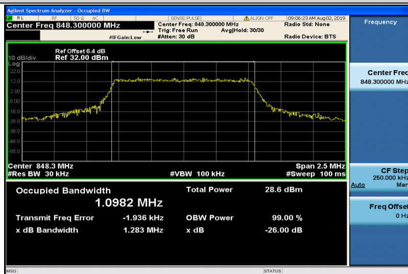
Band5-1.4MHz-QPSK-20643-6RB#0-1.0982
