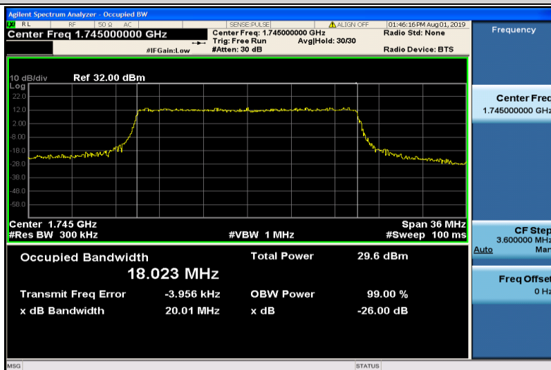
Band4-20MHz-QPSK-20300-100RB#0-18.023
