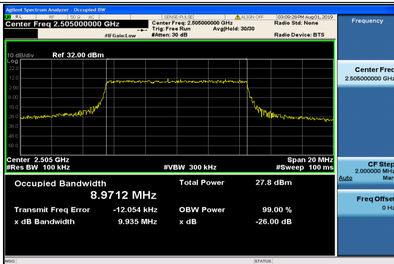
Band7-10MHz-16QAM-20800-50RB#0-8.9712
