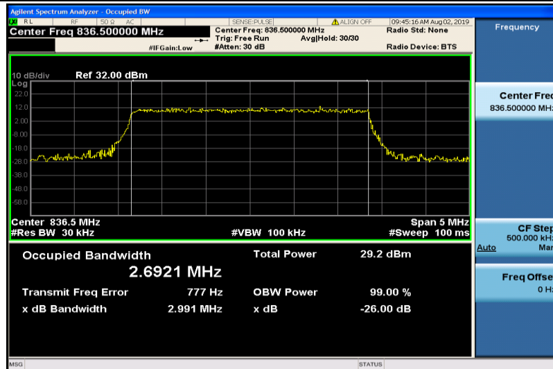
Band5-3MHz-QPSK-20525-15RB#0-2.6921
