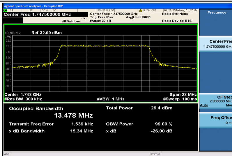
Band4-15MHz-QPSK-20325-75RB#0-13.478
