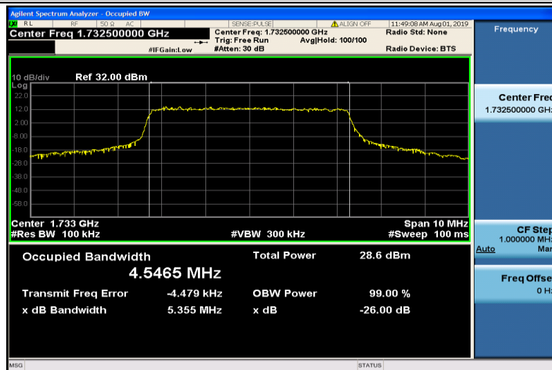
Band4-5MHz-16QAM-20175-25RB#0-4.5465
