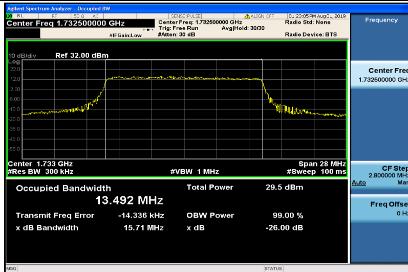
Band4-15MHz-QPSK-20175-75RB#0-13.492
