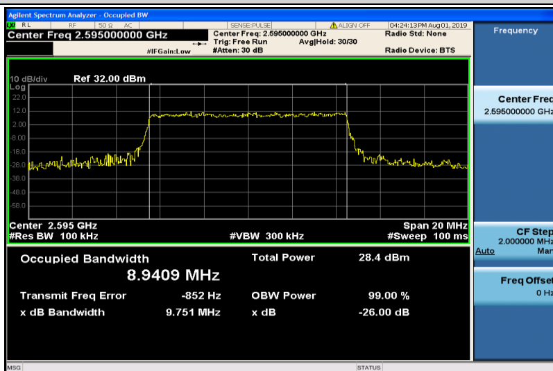
Band38-10MHz-QPSK-38000-50RB#0-8.9409
