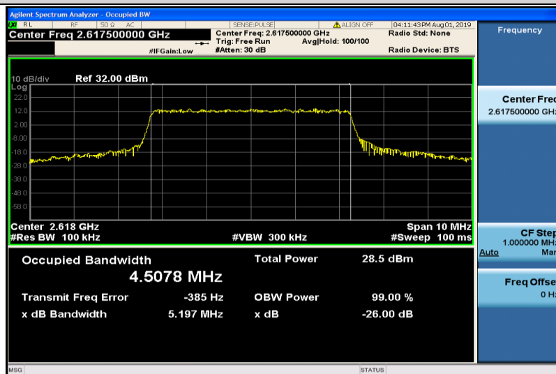
Band38-5MHz-QPSK-38225-25RB#0-4.5078
