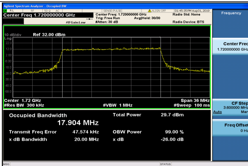
Band4-20MHz-QPSK-20050-100RB#0-17.904
