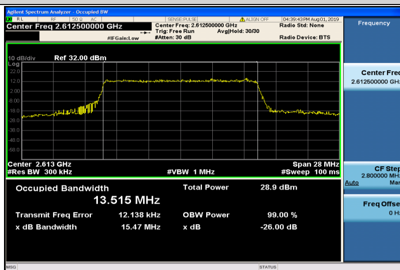
Band38-15MHz-QPSK-38175-75RB#0-13.515
