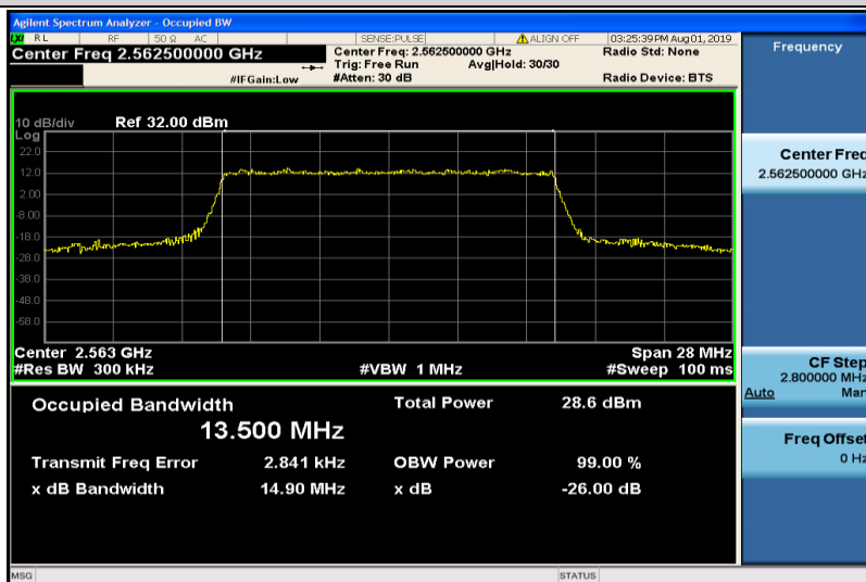
Band7-15MHz-16QAM-21375-75RB#0-13.500
