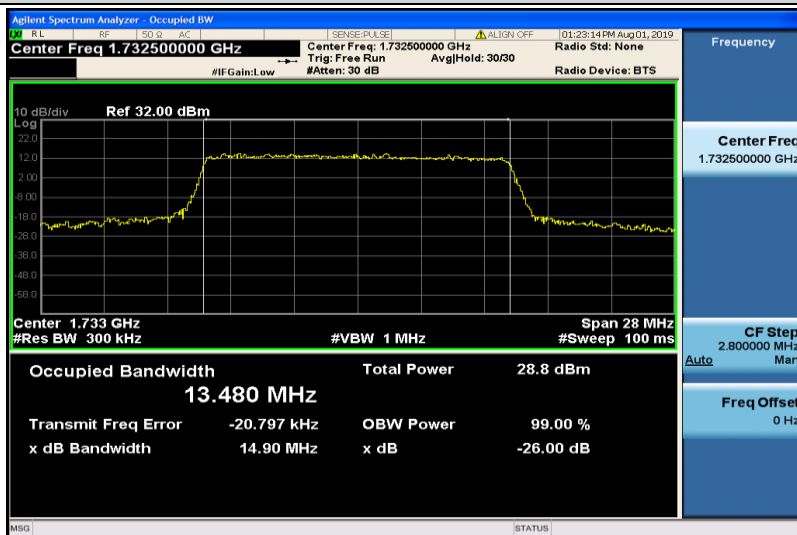
Band4-15MHz-16QAM-20175-75RB#0-13.480
