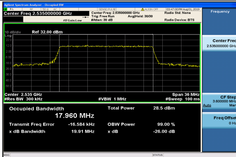
Band7-20MHz-16QAM-21100-100RB#0-17.960
