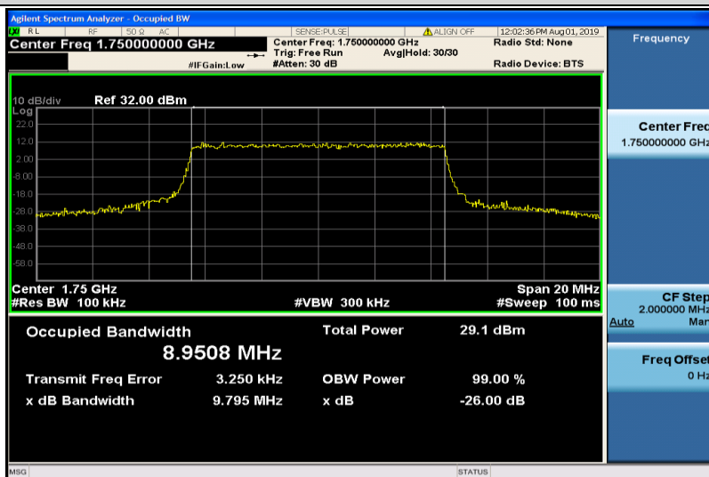
Band4-10MHz-QPSK-20350-50RB#0-8.9508
