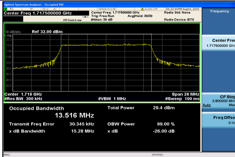
Band4-15MHz-QPSK-20025-75RB#0-13.516
