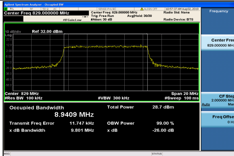
Band5-10MHz-16QAM-20450-50RB#0-8.9409
