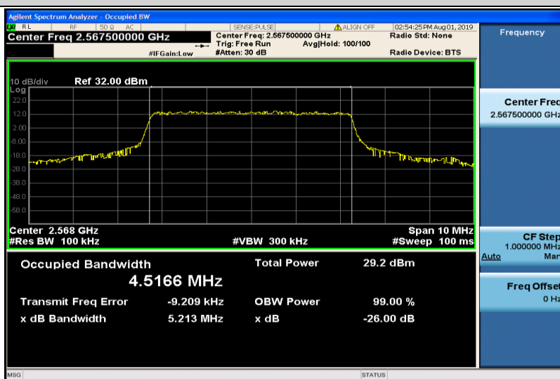
Band7-5MHz-QPSK-21425-25RB#0-4.5166
