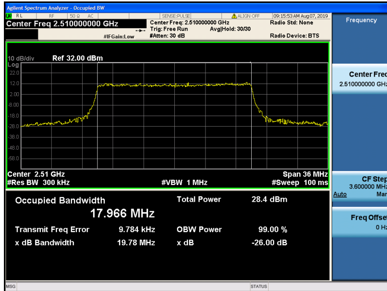
Band7-20MHz-QPSK-20850-100RB#0-9.4625
