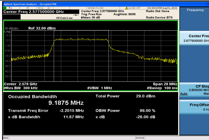
Band38-15MHz-QPSK-37825-75RB#0-9.1875
