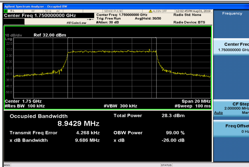
Band4-10MHz-16QAM-20350-50RB#0-8.9429
