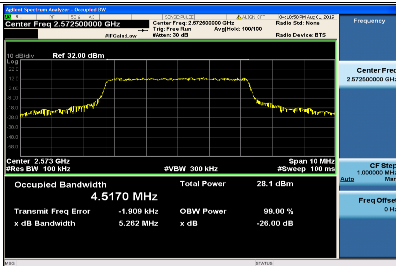
Band38-5MHz-16QAM-37775-25RB#0-4.5170
