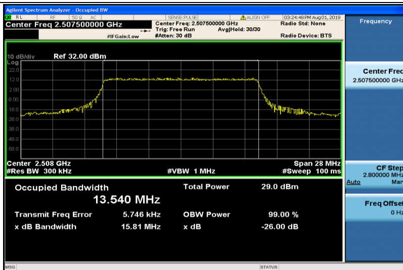
Band7-15MHz-QPSK-20825-75RB#0-13.540
