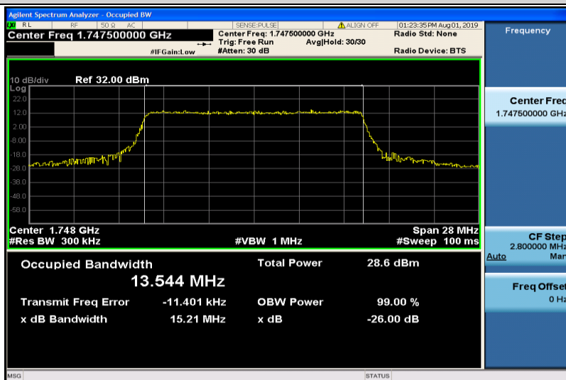
Band4-15MHz-16QAM-20325-75RB#0-13.544
