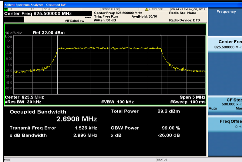
Band5-3MHz-QPSK-20415-15RB#0-2.6908
