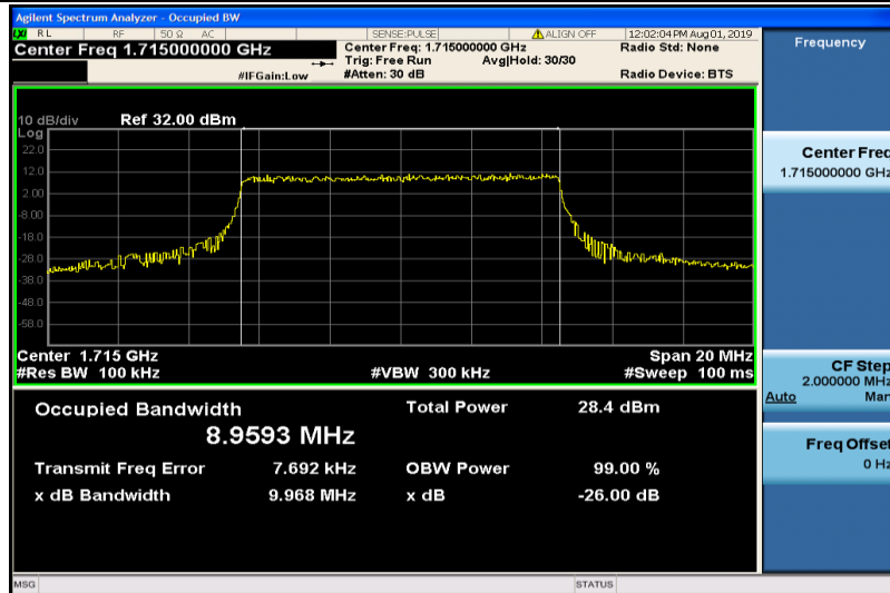
Band4-10MHz-16QAM-20000-50RB#0-8.9593
