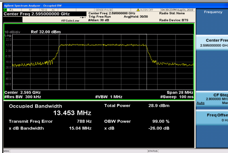
Band38-15MHz-QPSK-38000-75RB#0-13.453
