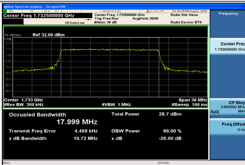
Band4-20MHz-16QAM-20175-100RB#0-17.999
