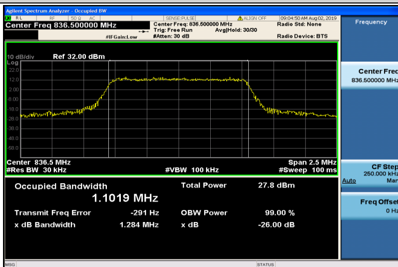
Band5-1.4MHz-16QAM-20525-6RB#0-1.1019
