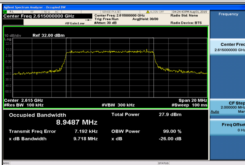
Band38-10MHz-16QAM-38200-50RB#0-8.9487
