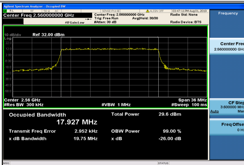
Band7-20MHz-QPSK-21350-100RB#0-17.927
