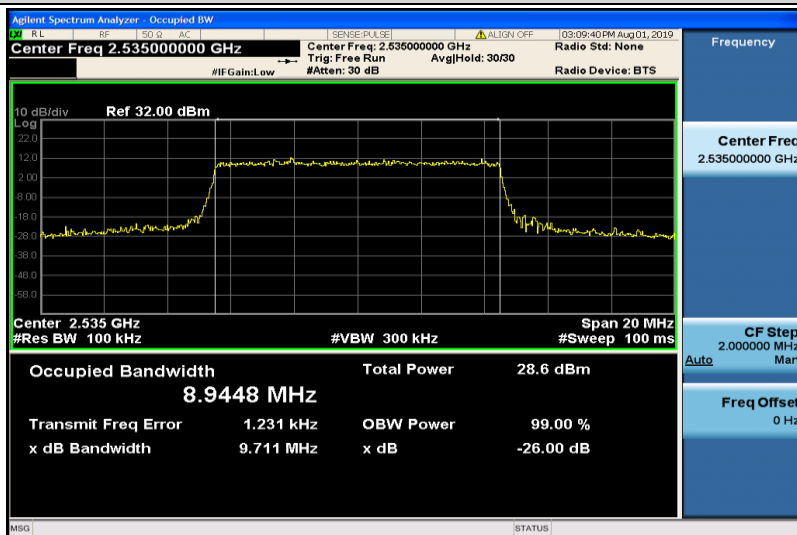
Band7-10MHz-QPSK-21100-50RB#0-8.9448
