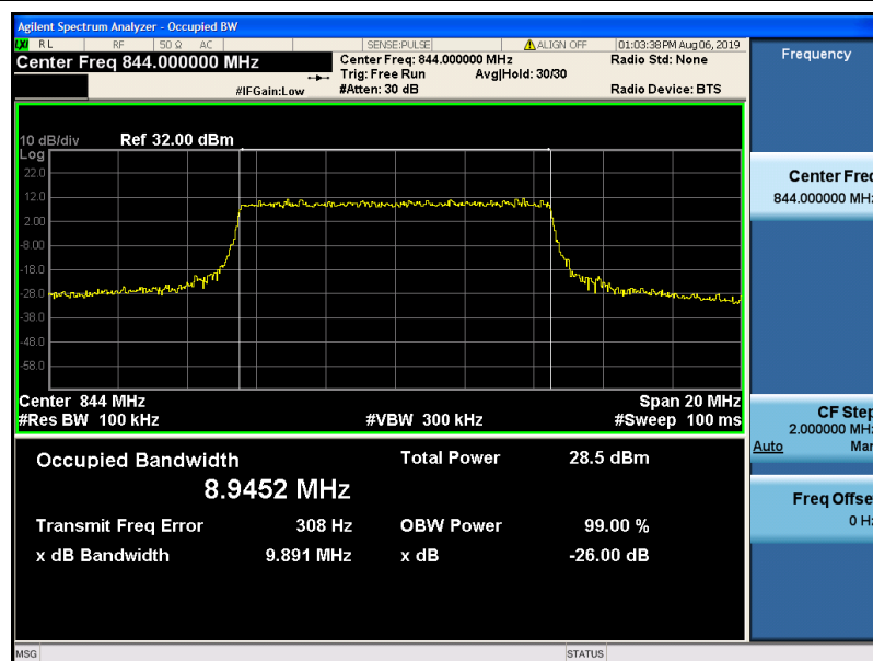
Band5-10MHz-16QAM-20600-50RB#0-8.9452
