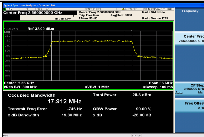
Band7-20MHz-16QAM-21350-100RB#0-17.912
