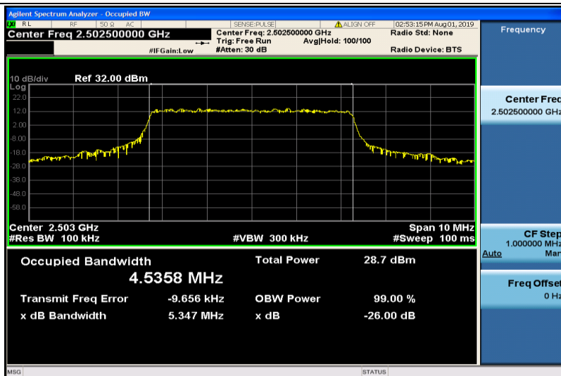
Band7-5MHz-QPSK-20775-25RB#0-4.5358
