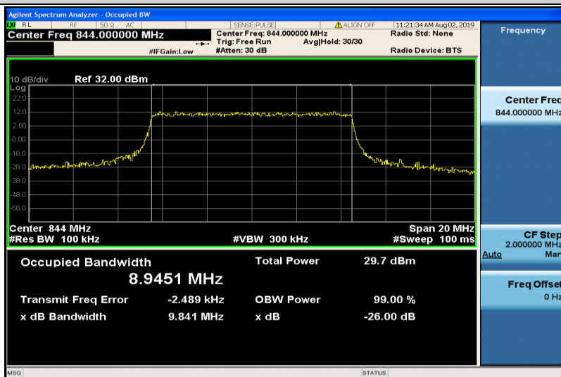
Band5-10MHz-QPSK-20600-50RB#0-8.9451
