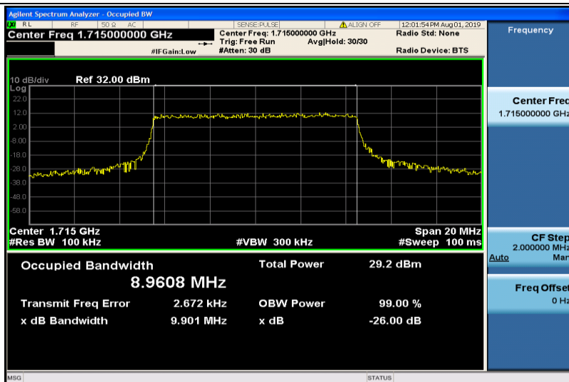
Band4-10MHz-QPSK-20000-50RB#0-8.9608
