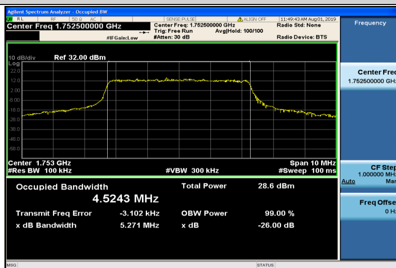
Band4-5MHz-16QAM-20375-25RB#0-4.5243
