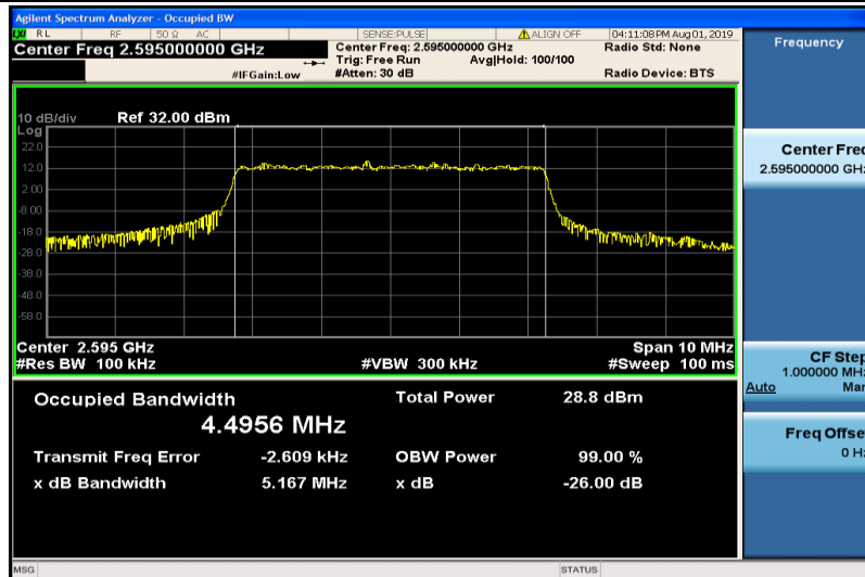
Band38-5MHz-QPSK-38000-25RB#0-4.4956
