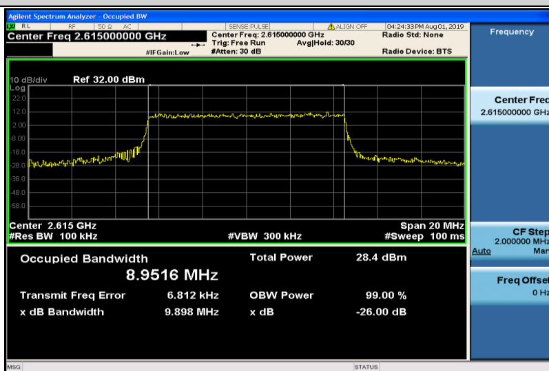
Band38-10MHz-QPSK-38200-50RB#0-8.9516
