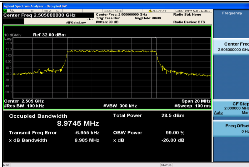
Band7-10MHz-QPSK-20800-50RB#0-8.9745
