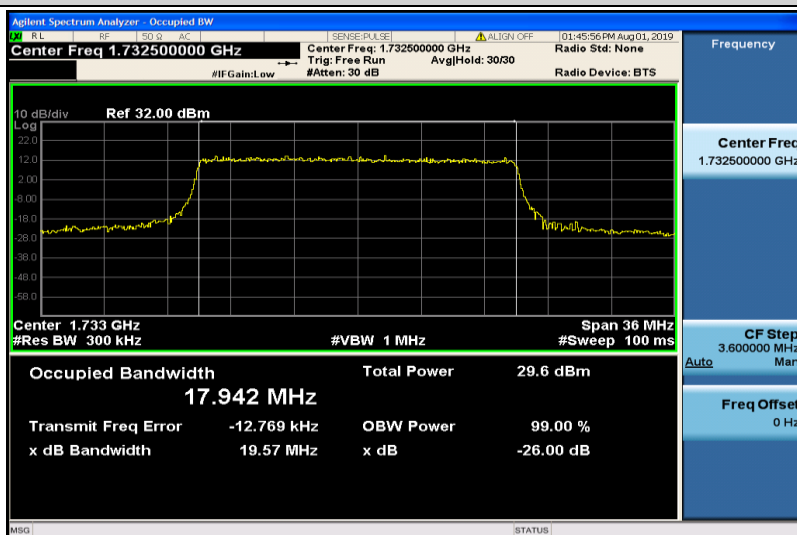
Band4-20MHz-QPSK-20175-100RB#0-17.942
