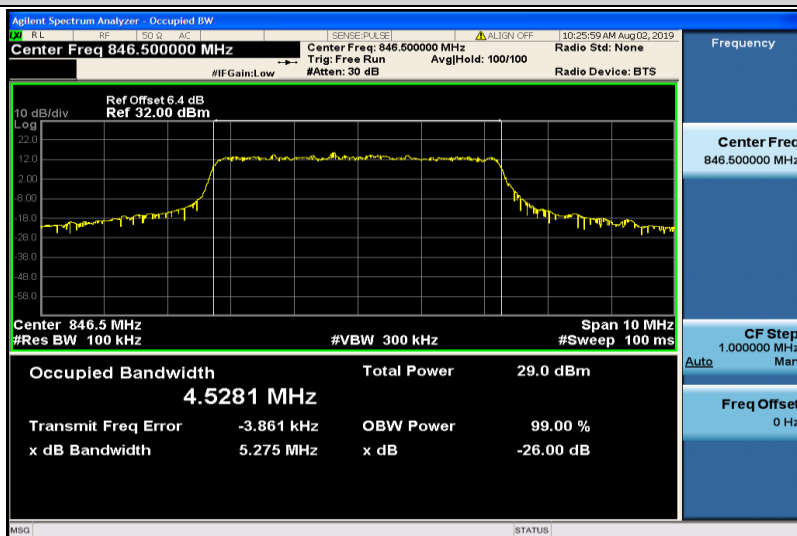
Band5-5MHz-16QAM-20625-25RB#0-4.5281
