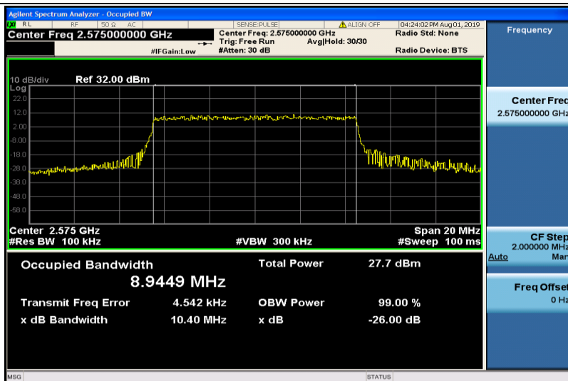
Band38-10MHz-16QAM-37800-50RB#0-8.9449
