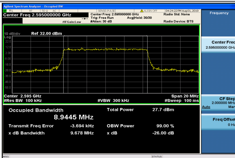
Band38-10MHz-16QAM-38000-50RB#0-8.9445
