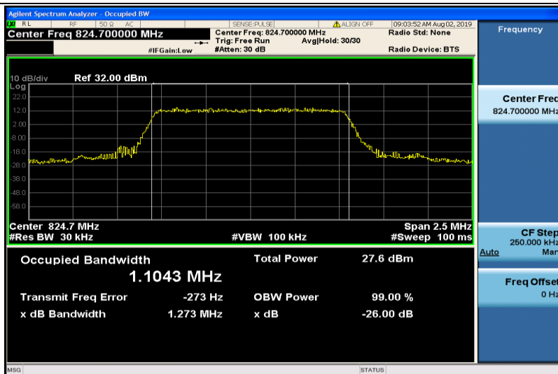
Band5-1.4MHz-16QAM-20407-6RB#0-1.1043
