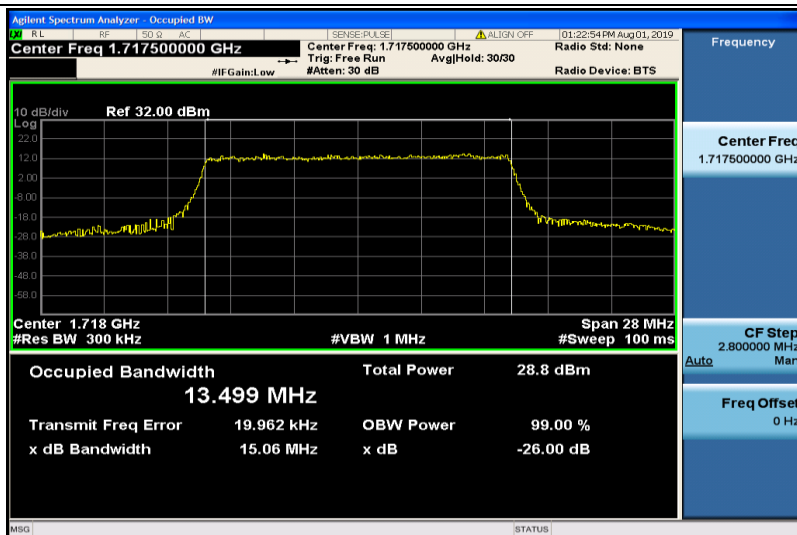
Band4-15MHz-16QAM-20025-75RB#0-13.499
