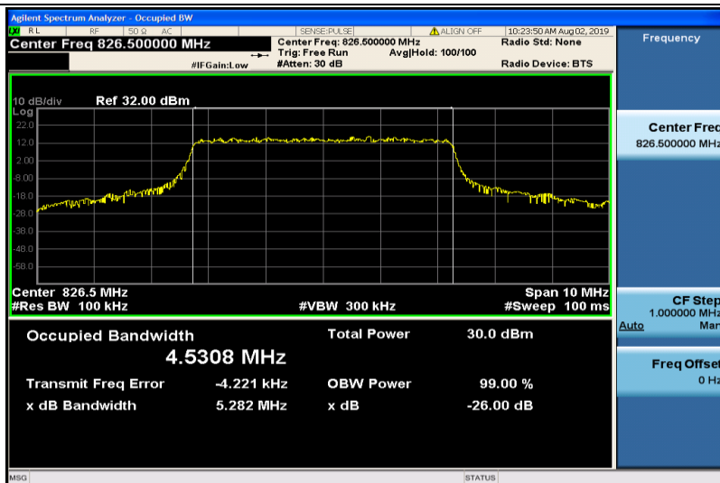
Band5-5MHz-QPSK-20425-25RB#0-4.5308
