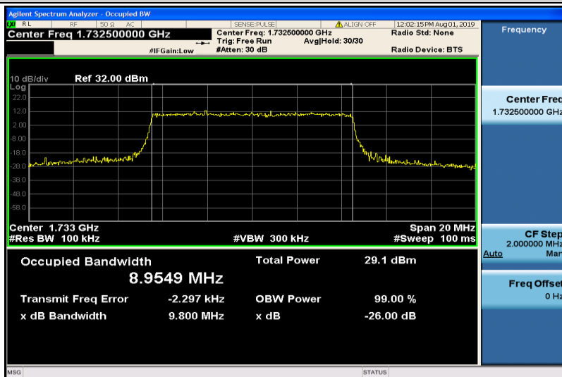
Band4-10MHz-QPSK-20175-50RB#0-8.9549
