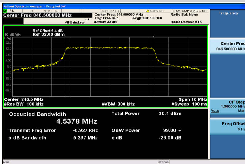
Band5-5MHz-QPSK-20625-25RB#0-4.5378
