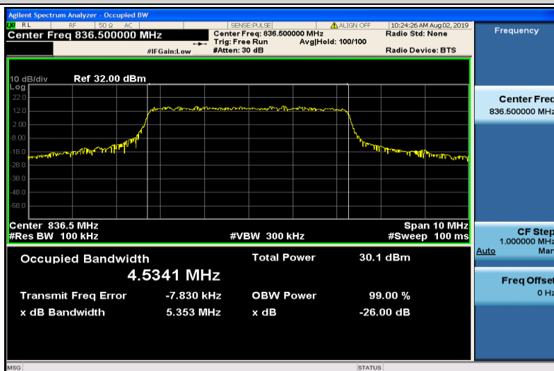
Band5-5MHz-QPSK-20525-25RB#0-4.5341
