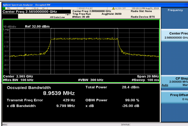
Band7-10MHz-16QAM-21400-50RB#0-8.9539
