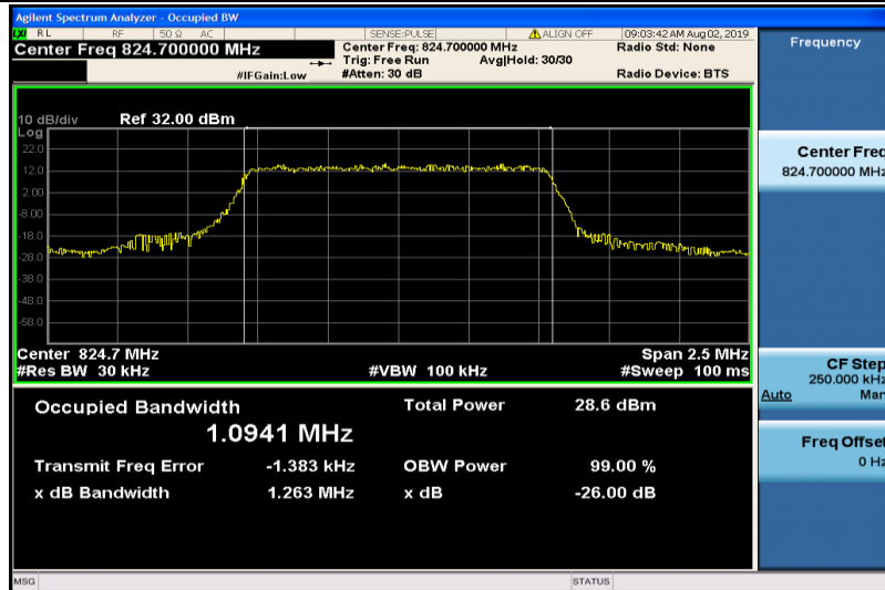
Band5-1.4MHz-QPSK-20407-6RB#0-1.0941
