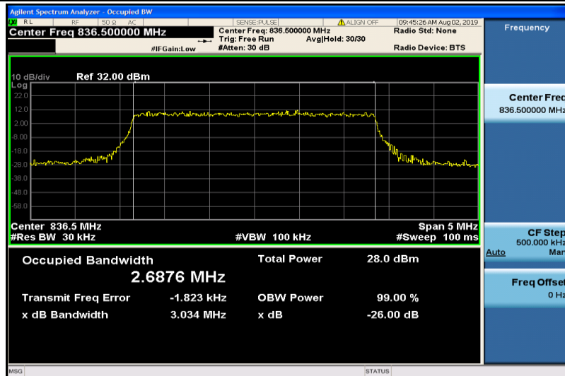
Band5-3MHz-16QAM-20525-15RB#0-2.6876
