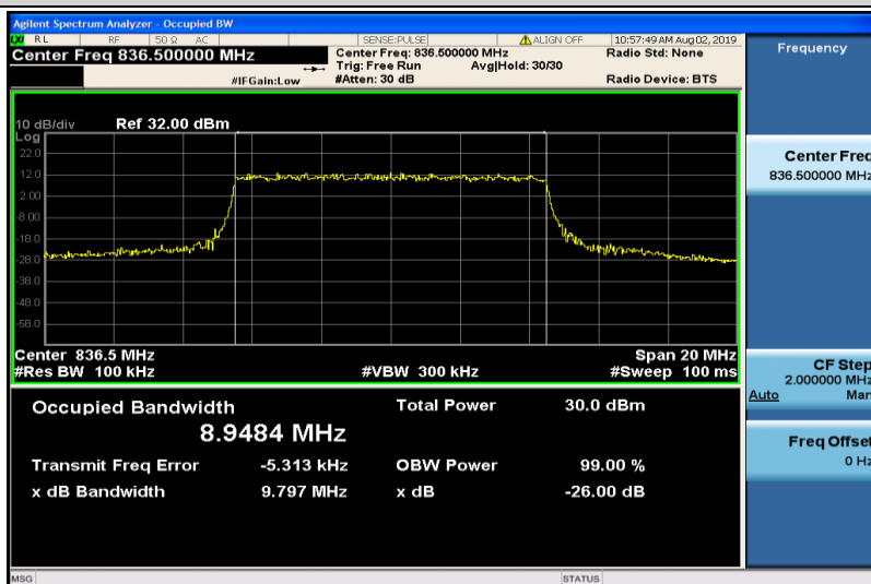
Band5-10MHz-QPSK-20525-50RB#0-8.9484
