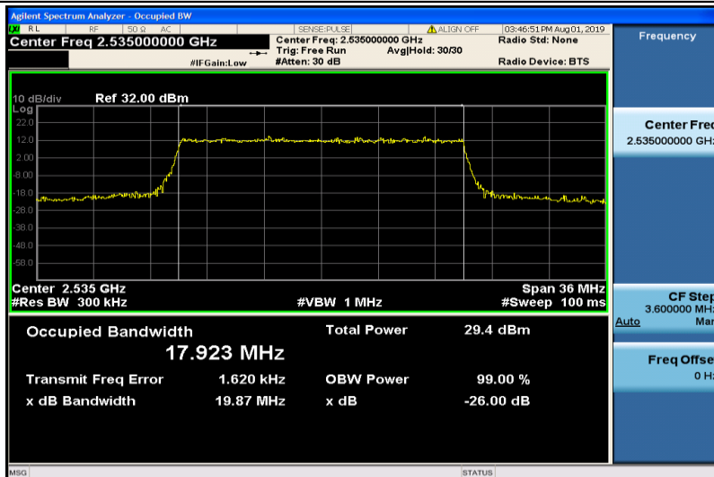
Band7-20MHz-QPSK-21100-100RB#0-17.923
