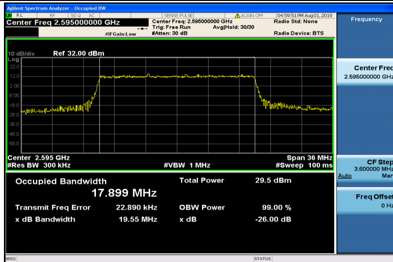
Band38-20MHz-QPSK-38000-100RB#0-17.899
