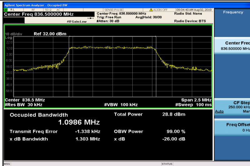
Band5-1.4MHz-QPSK-20525-6RB#0-1.0986
