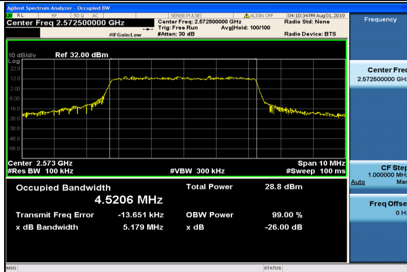
Band38-5MHz-QPSK-37775-25RB#0-4.5206
