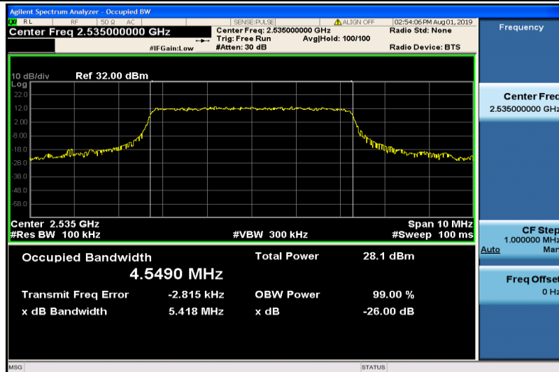
Band7-5MHz-16QAM-21100-25RB#0-4.5490
