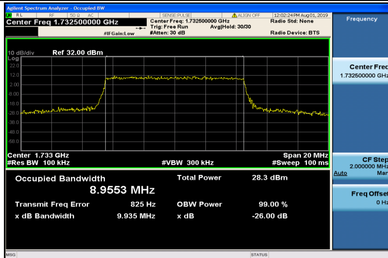
Band4-10MHz-16QAM-20175-50RB#0-8.9553
