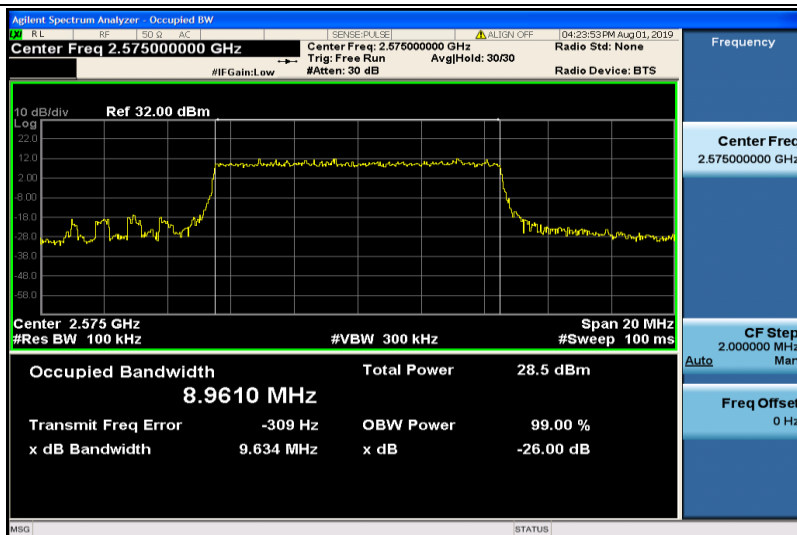
Band38-10MHz-QPSK-37800-50RB#0-8.9610
