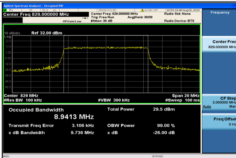
Band5-10MHz-QPSK-20450-50RB#0-8.9413
