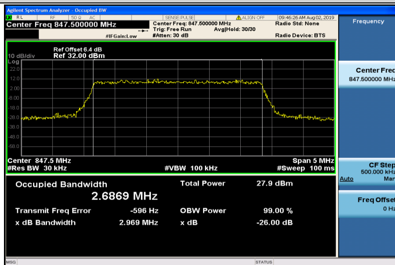
Band5-3MHz-16QAM-20635-15RB#0-2.6869
