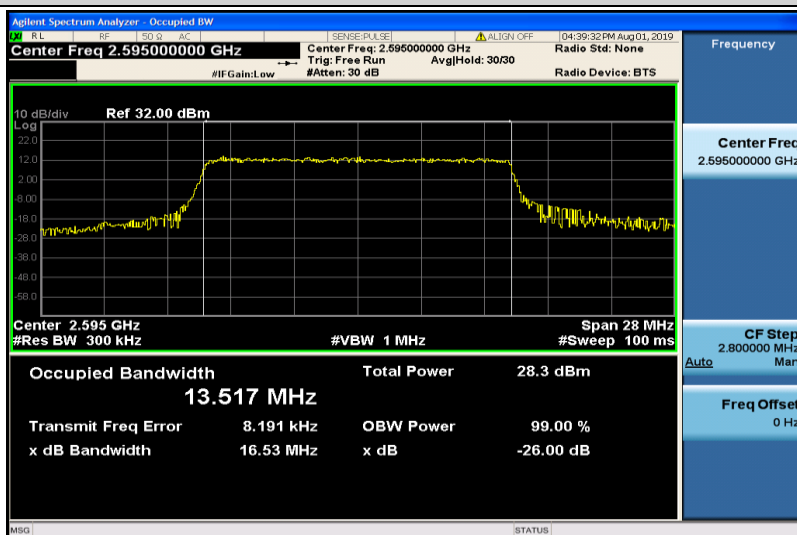
Band38-15MHz-16QAM-38000-75RB#0-13.517
