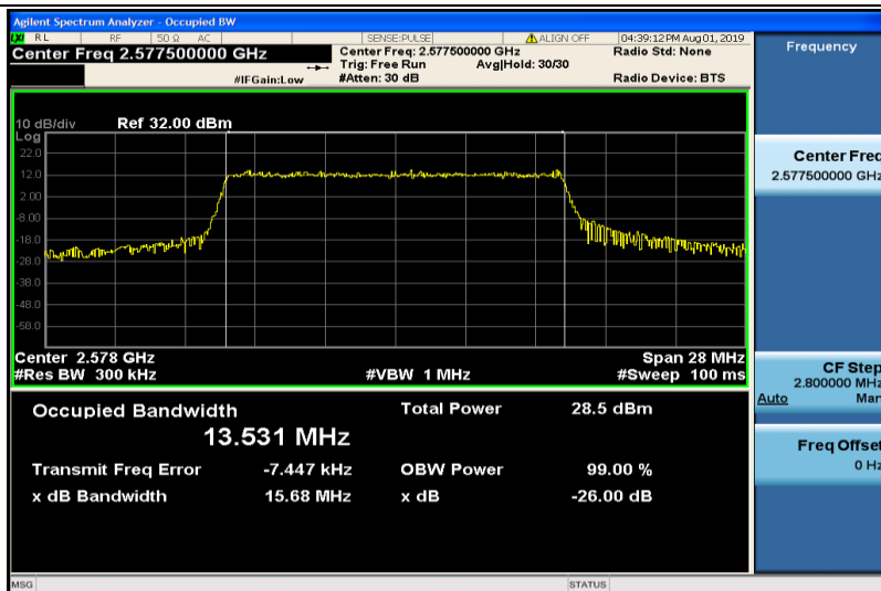
Band38-15MHz-16QAM-37825-75RB#0-13.531
