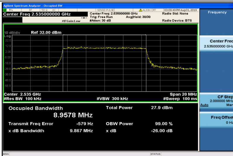
Band7-10MHz-16QAM-21100-50RB#0-8.9578
