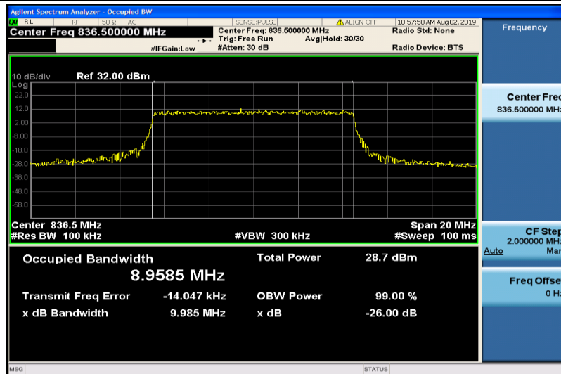
Band5-10MHz-16QAM-20525-50RB#0-8.9585
