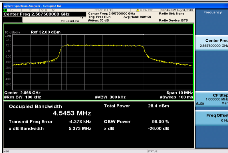
Band7-5MHz-16QAM-21425-25RB#0-4.5453
