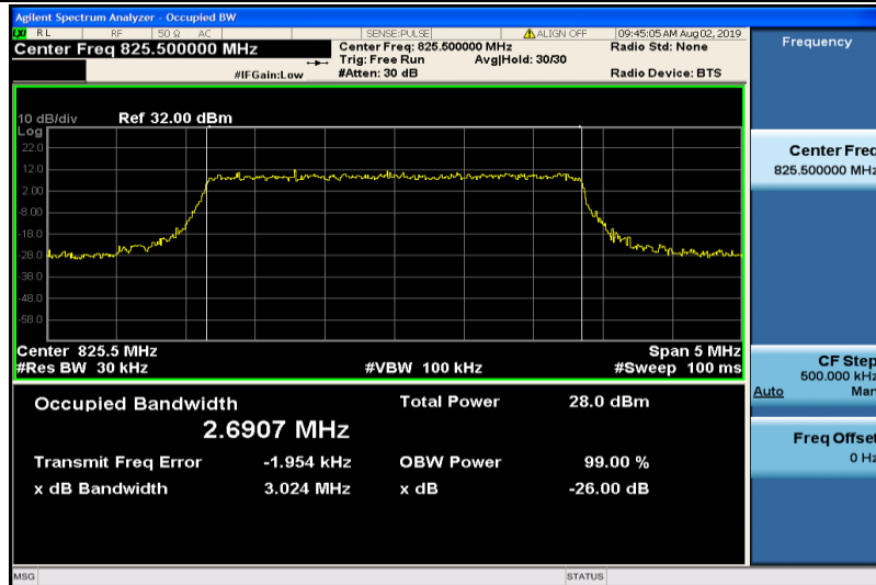
Band5-3MHz-16QAM-20415-15RB#0-2.6907
