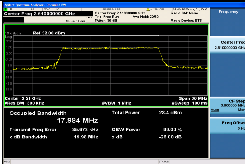
Band7-20MHz-16QAM-20850-100RB#0-17.984
