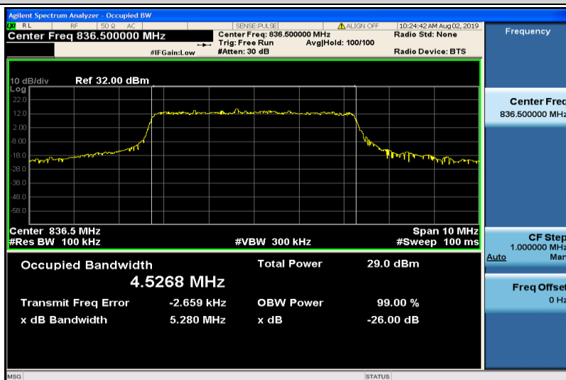
Band5-5MHz-16QAM-20525-25RB#0-4.5268
