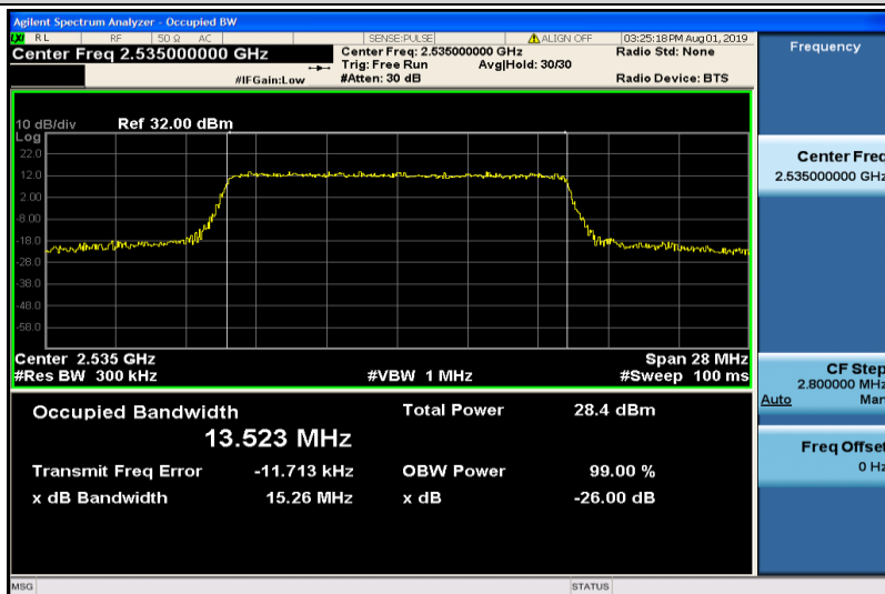
Band7-15MHz-16QAM-21100-75RB#0-13.523
