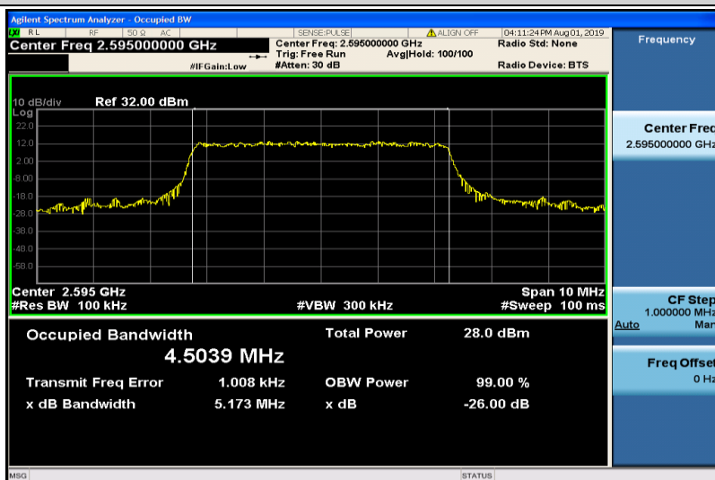
Band38-5MHz-16QAM-38000-25RB#0-4.5039
