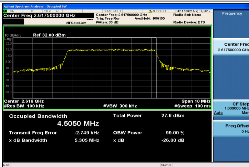
Band38-5MHz-16QAM-38225-25RB#0-4.5050
