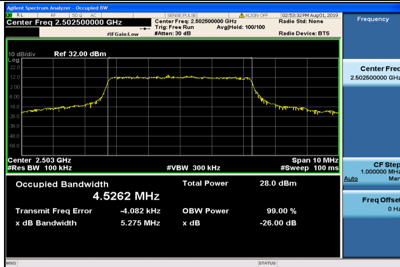
Band7-5MHz-16QAM-20775-25RB#0-4.5262
