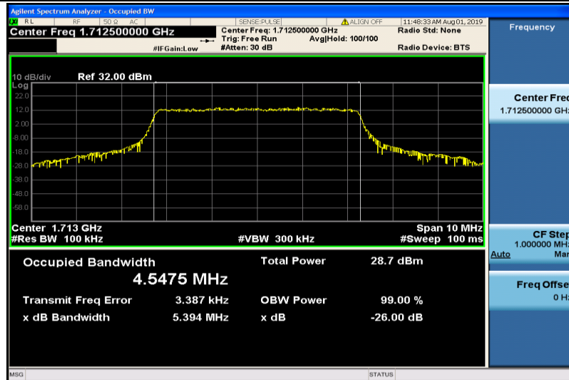
Band4-5MHz-16QAM-19975-25RB#0-4.5475
