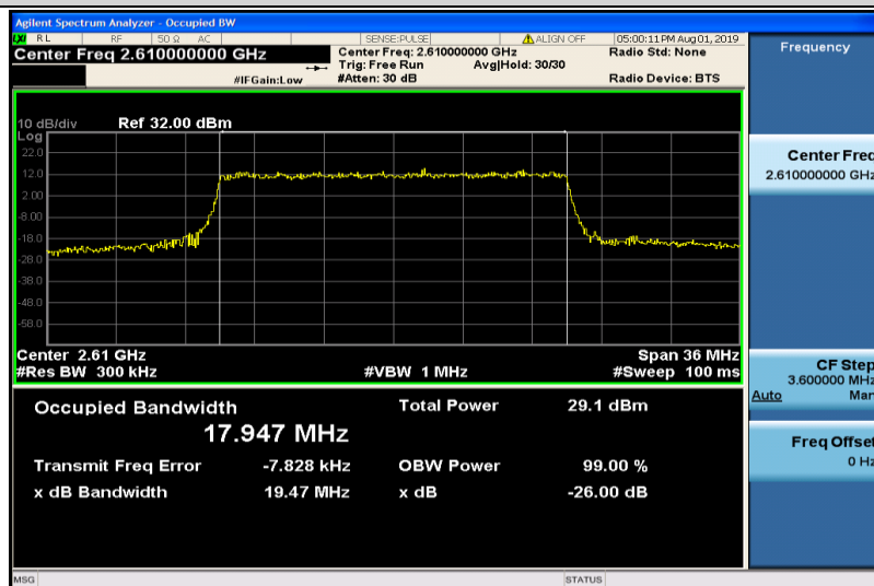
Band38-20MHz-QPSK-38150-100RB#0-17.947
