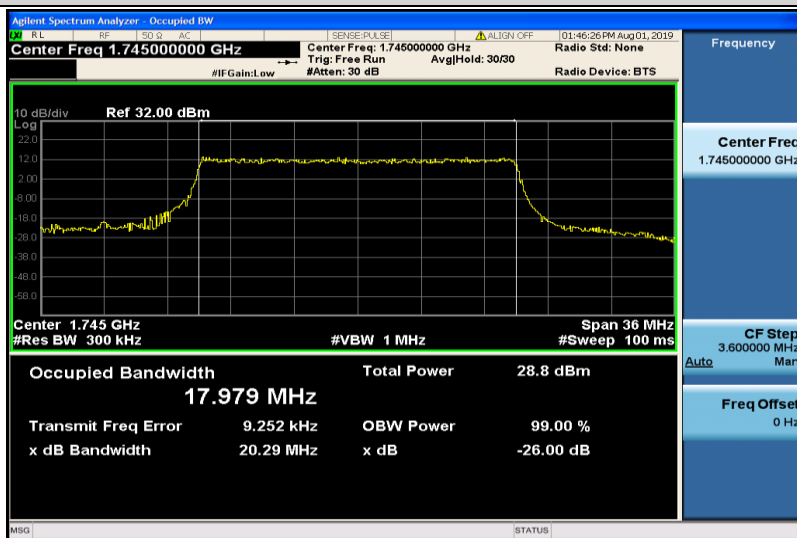
Band4-20MHz-16QAM-20300-100RB#0-17.979
