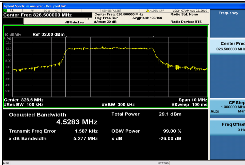
Band5-5MHz-16QAM-20425-25RB#0-4.5283
