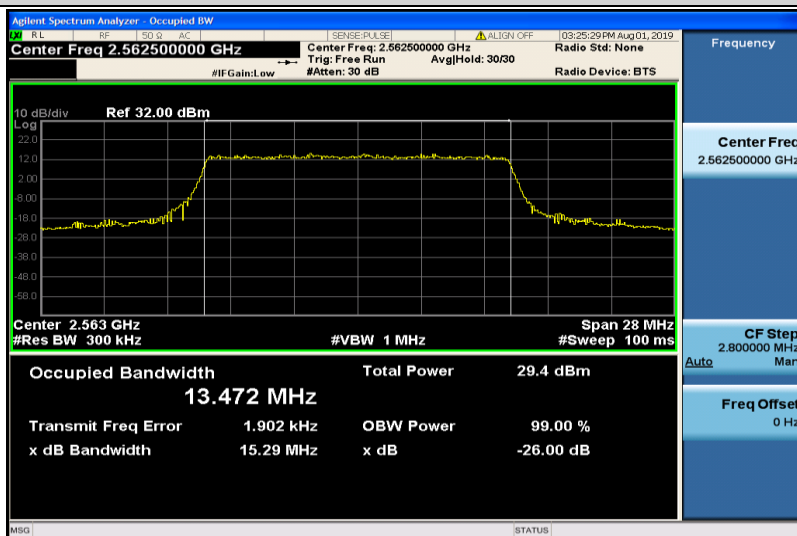
Band7-15MHz-QPSK-21375-75RB#0-13.472
