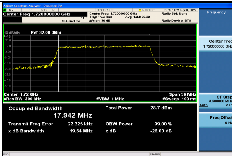
Band4-20MHz-16QAM-20050-100RB#0-17.942
