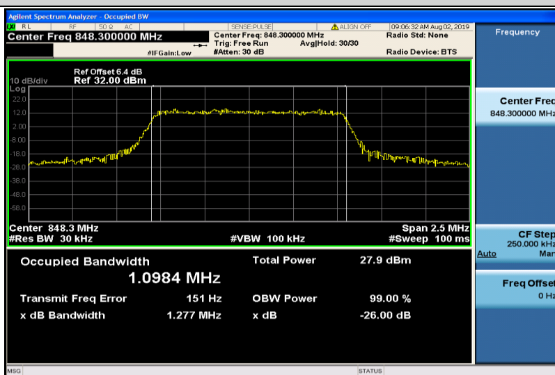
Band5-1.4MHz-16QAM-20643-6RB#0-1.0984
