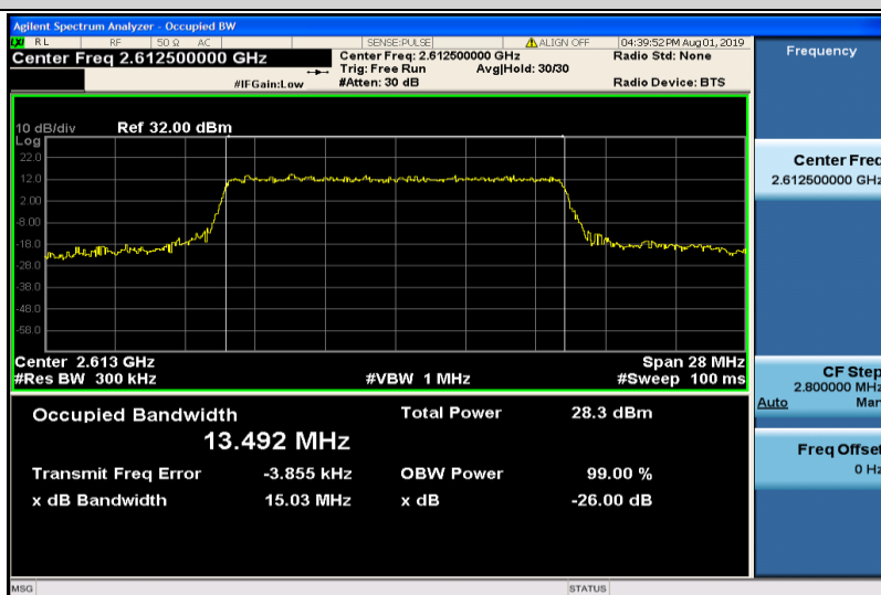
Band38-15MHz-16QAM-38175-75RB#0-13.492
