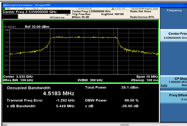
Band7-5MHz-QPSK-21100-25RB#0-4.5183
