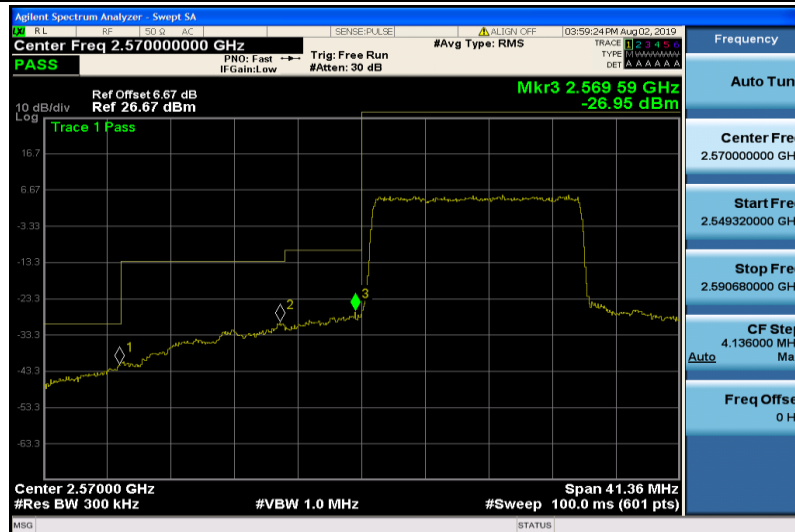
Band38-15MHz-16QAM-37825-75RB#0
