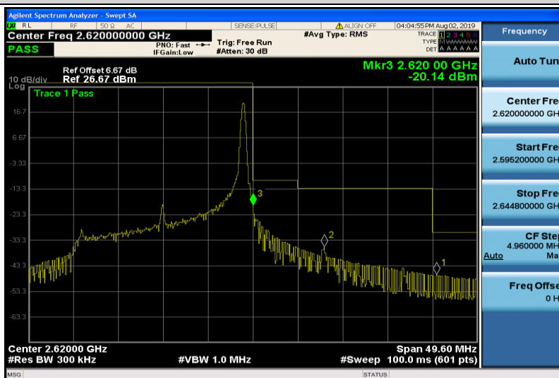
Band38-20MHz-16QAM-38150-1RB#99
