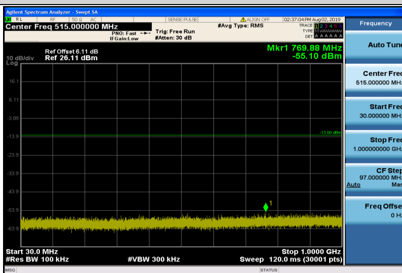
Band2-5MHz-QPSK-18900-1RB#0-30~1000MHz
