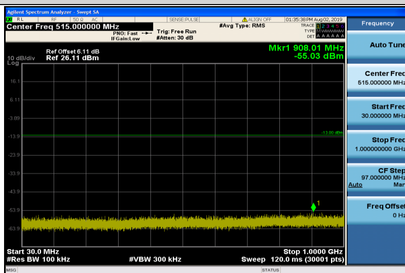
Band2-1.4MHz-16QAM-18900-1RB#0-30~1000MHz
