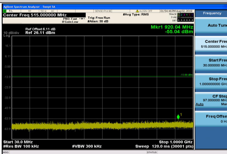
Band2-3MHz-16QAM-18900-1RB#0-30~1000MHz
