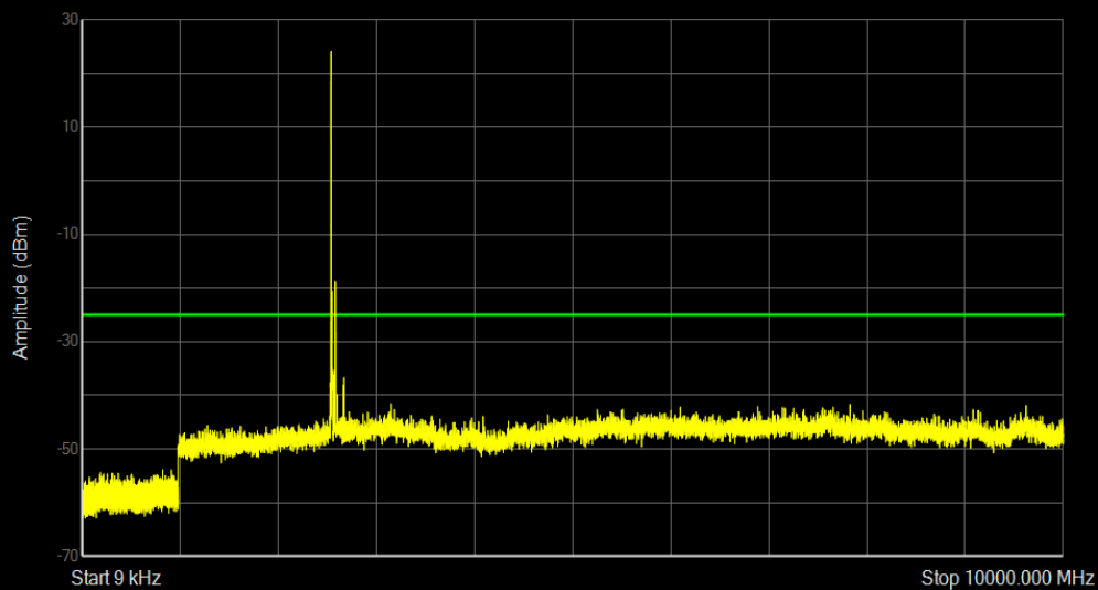
Band41 QPSK BW=20MHz Channel=40340 RB Size=1 Position=#0
