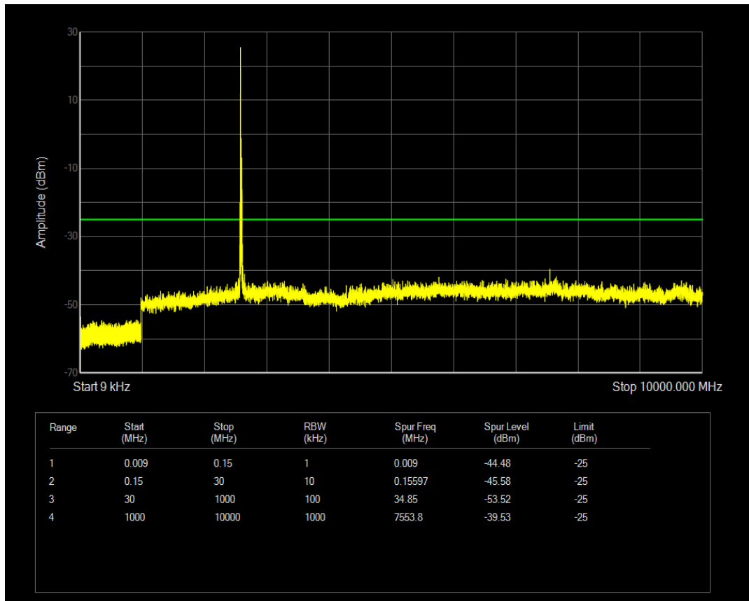
Band41 QAM16 BW=20MHz Channel=40740 RB Size=1 Position=#0
