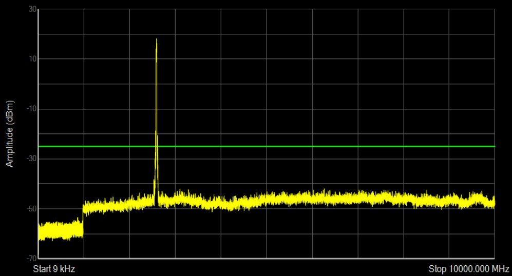
Band41 QAM16 BW=20MHz Channel=40740 RB Size=100 Position=#0
