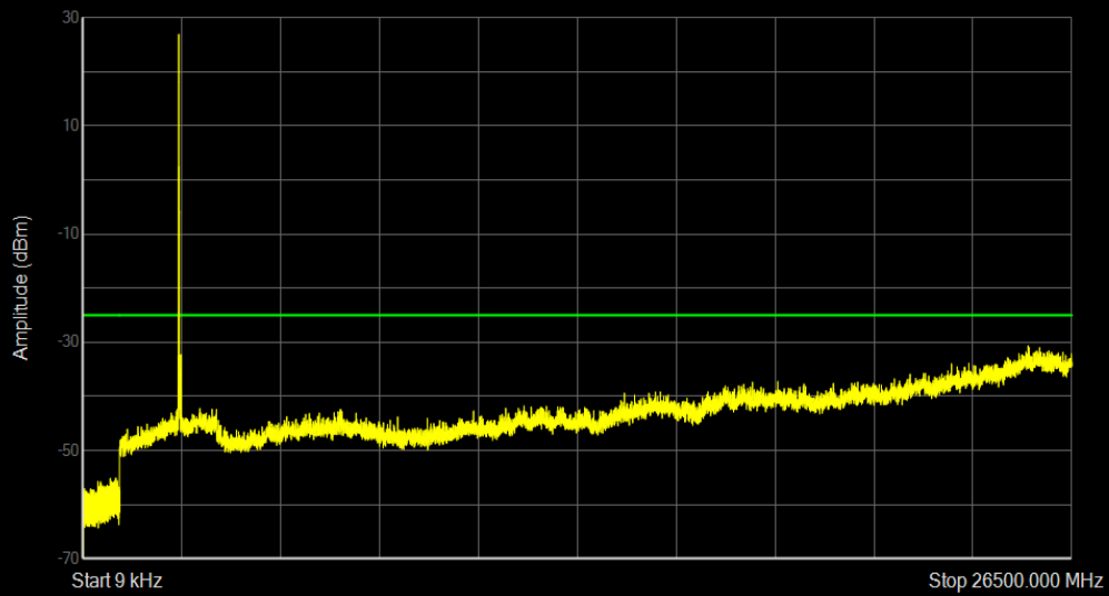
Band38 QAM16 BW=20MHz Channel=38000 RB Size=1 Position=#0
