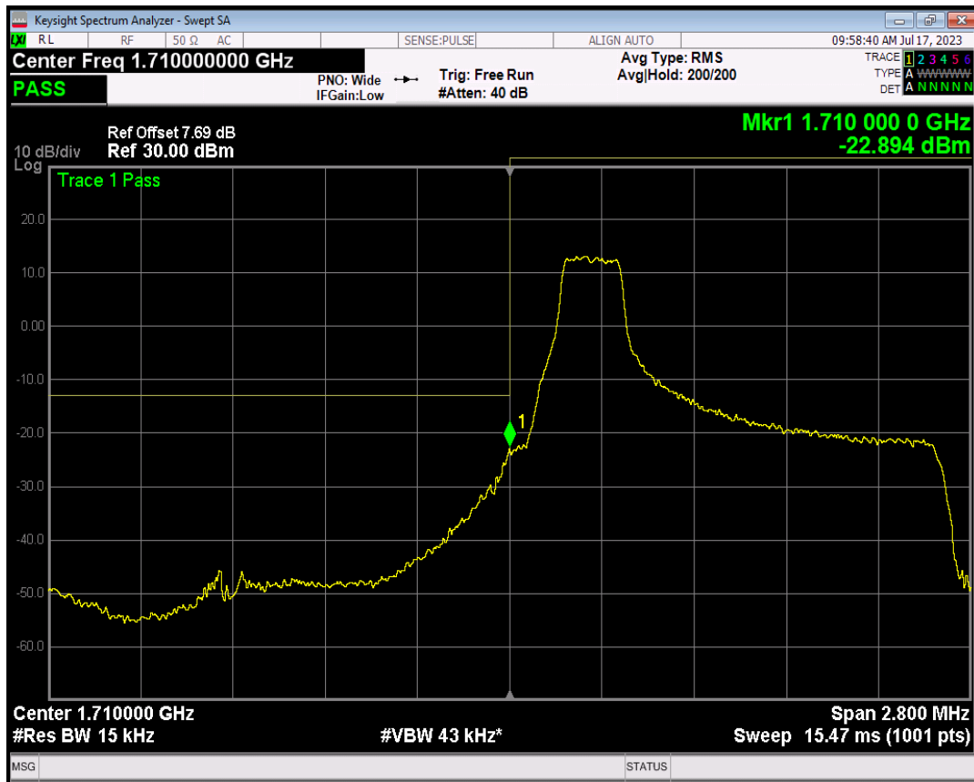
Band66 16QAM BW=1.4MHz Channel=131979 RB Size=1 Position=#Max
