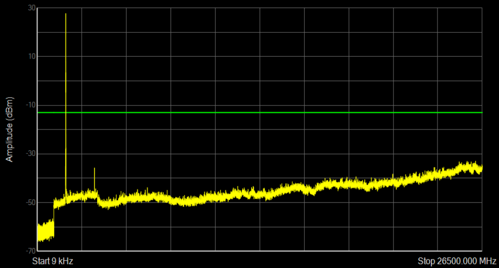
Band4 16QAM BW=10MHz Channel=20000 RB Size=1 Position=#0
