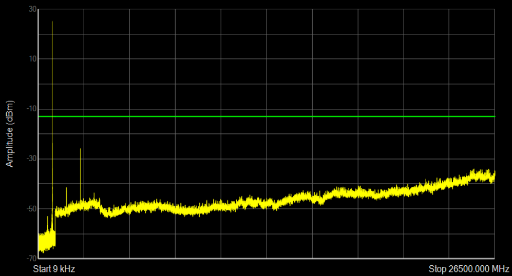
Band5 16QAM BW=1.4MHz Channel=20407 RB Size=1 Position=#0
