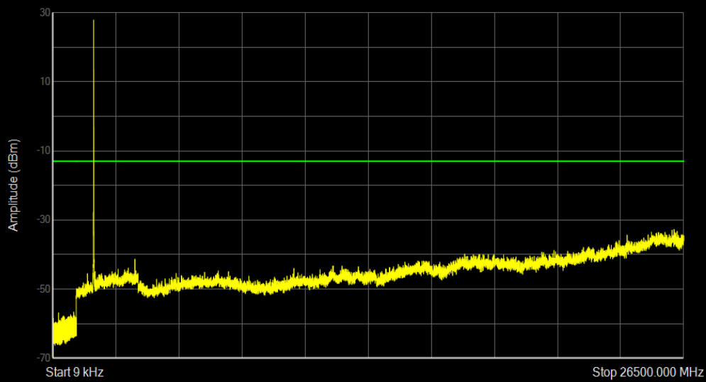
Band4 16QAM BW=5MHz Channel=20175 RB Size=1 Position=#0
