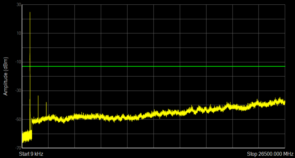
Band26a QPSK BW=5MHz Channel=26765 RB Size=1 Position=#0
