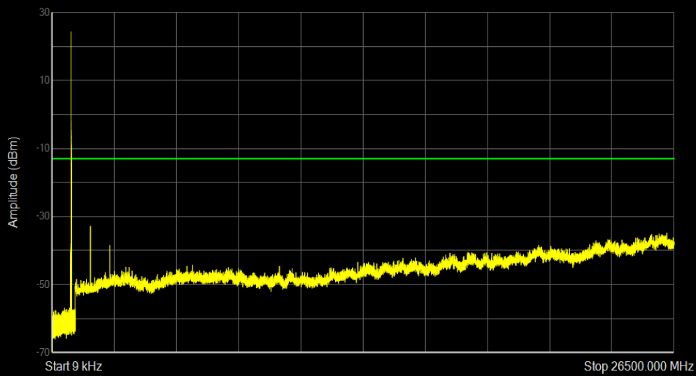
Band26b QPSK BW=10MHz Channel=26840 RB Size=1 Position=#0
