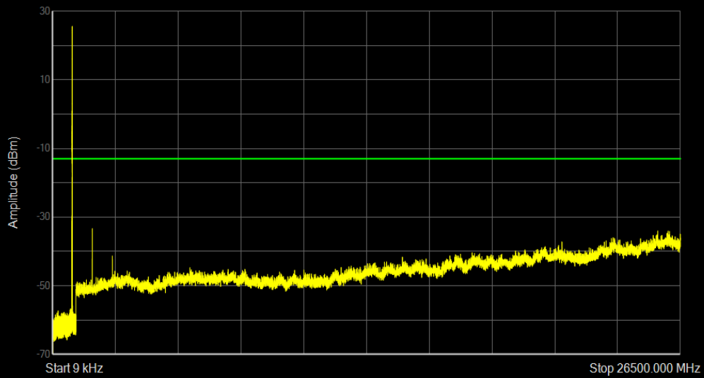
Band26b 16QAM BW=3MHz Channel=27025 RB Size=1 Position=#0
