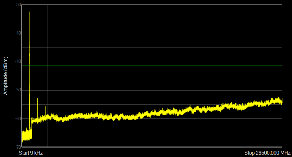
Band26a 16QAM BW=3MHz Channel=26705 RB Size=1 Position=#0
