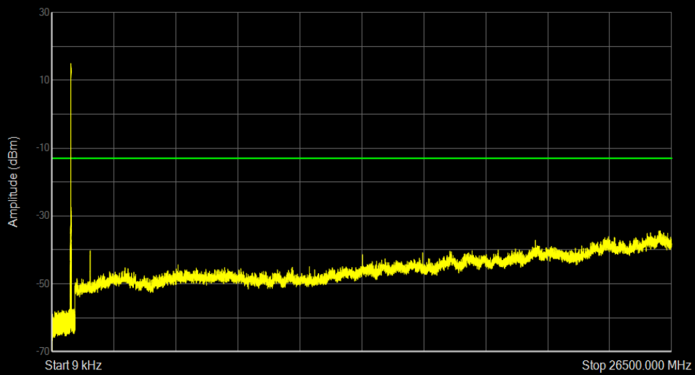
Band26b 16QAM BW=5MHz Channel=26815 RB Size=25 Position=#0
