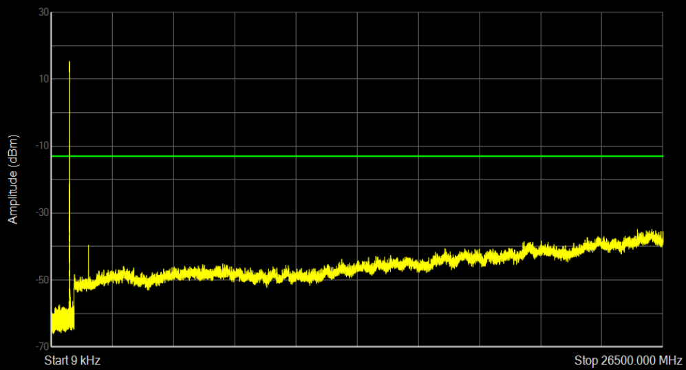
Band26a 16QAM BW=3MHz Channel=26705 RB Size=15 Position=#0
