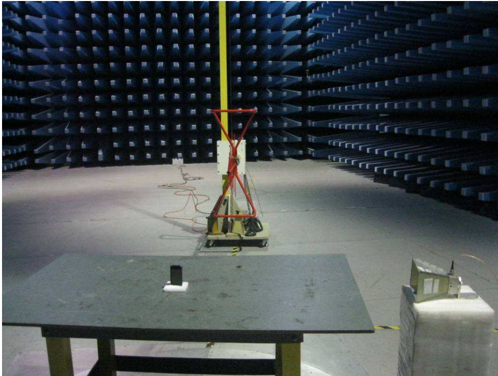
Below 1GHz: Radiated Emissions - Front View (GPS Receiving)
