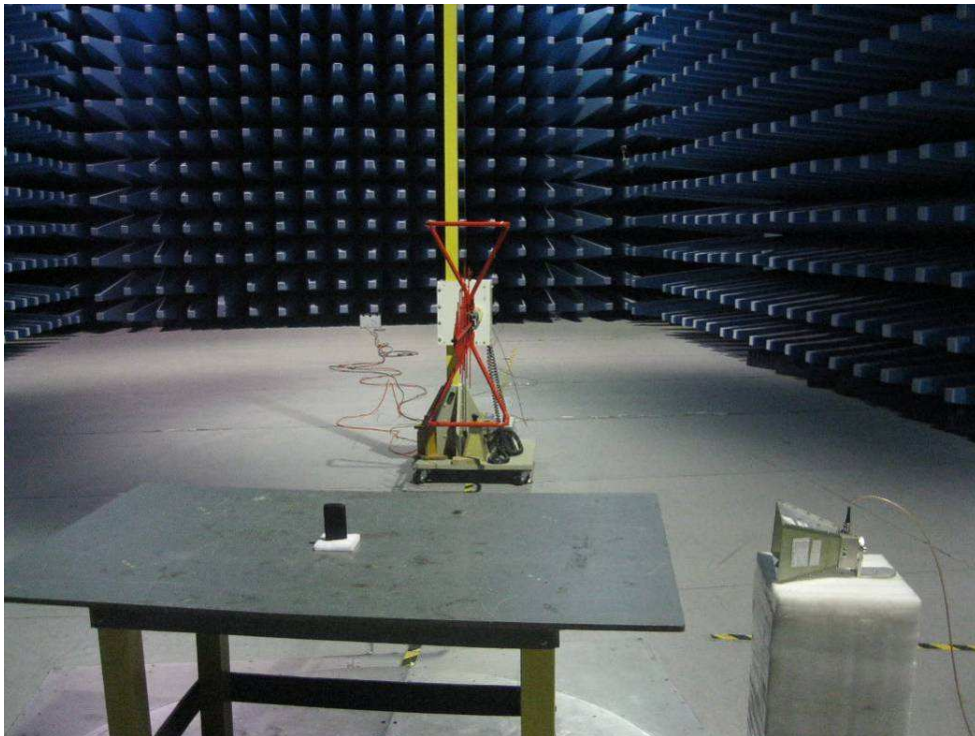
Below 1GHz: Radiated Emissions - Rear View (GPS Receiving)
