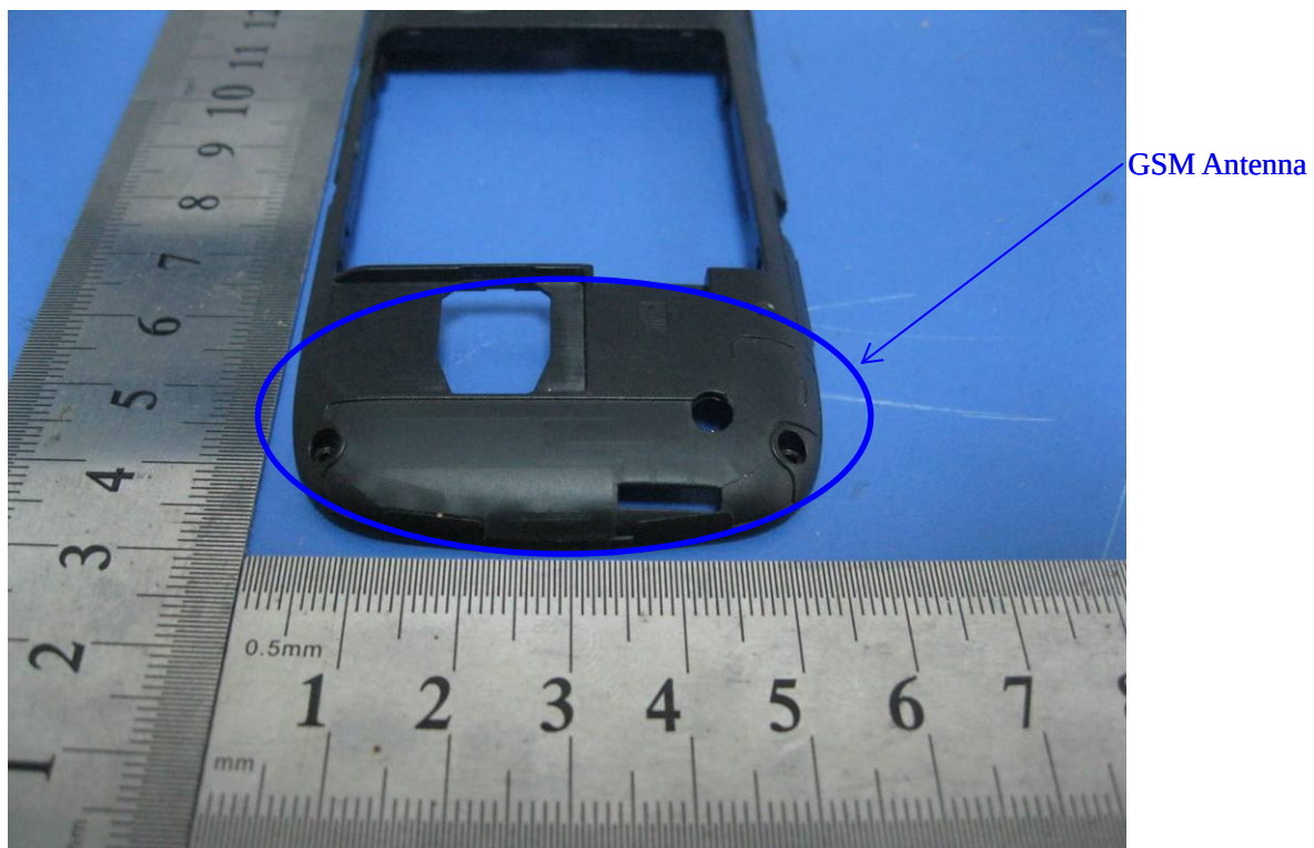
GSM Antenna - Top View
