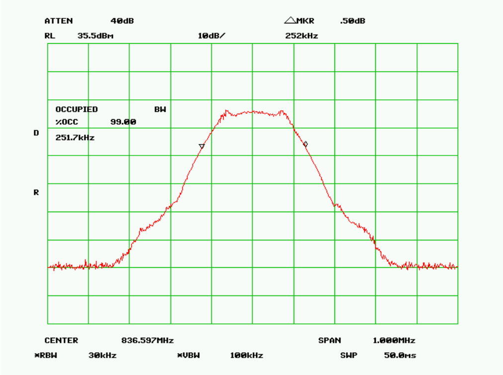
99% Occupied Bandwidth
