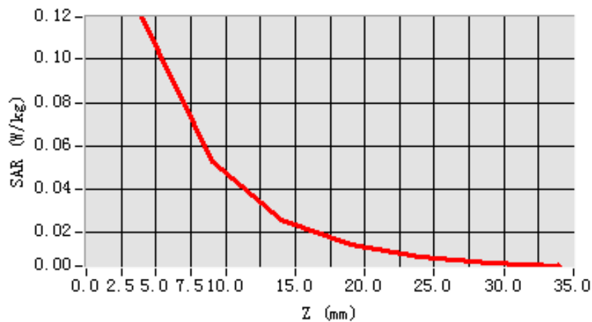
SAR, Z Axis Scan (X = -55, Y = -55)
