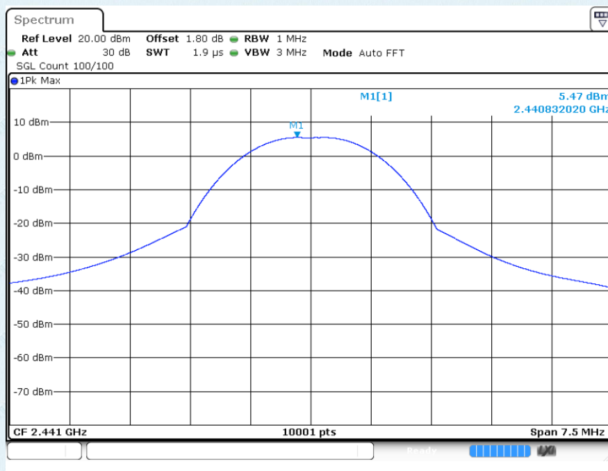
Middle channel
