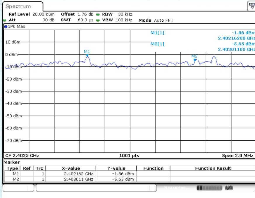
Lowest channel
