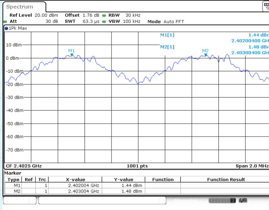
Lowest channel
