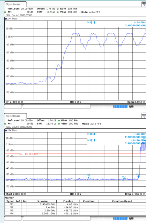
Hopping mode
