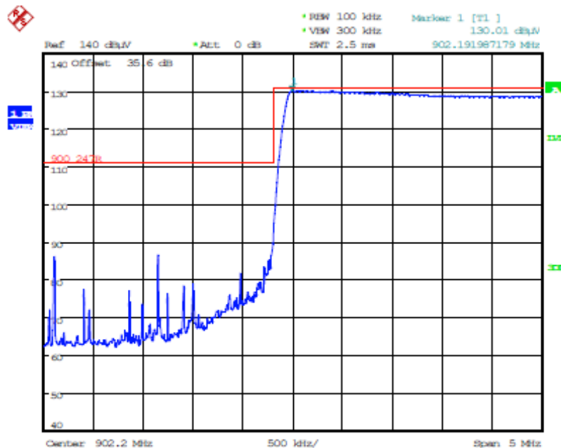
Plot 5.5.3.5.3.2. Band-Edge RF Radiated Emissions at 3 m, Horizontal Polarization Pseudorandom Hopping Mode, Low End of Frequency Band, 902.2 MHz, GFSK DSSS8, 10 kbps Left Antenna
