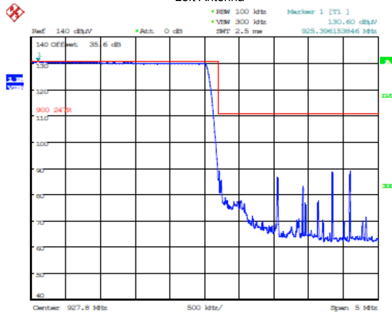
Plot 5.5.3.5.3.8. Band-Edge RF Radiated Emissions at 3 m, Vertical Polarization Pseudorandom Hopping Mode, High End of Frequency Band, 927.8 MHz, GFSK DSSS8, 10 kbps
