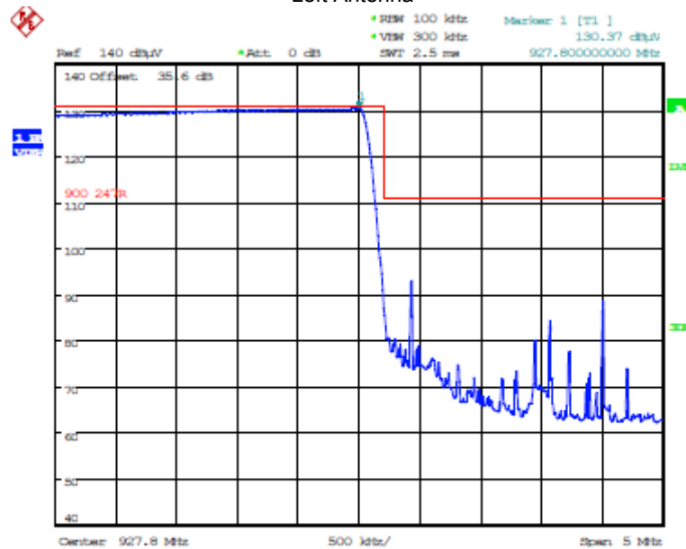
Plot 5.5.3.5.3.6. Band-Edge RF Radiated Emissions at 3 m, Horizontal Polarization Pseudorandom Hopping Mode, High End of Frequency Band, 927.8 MHz, GFSK DSSS8, 10 kbps
