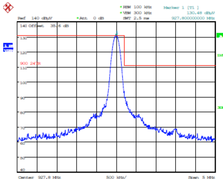
Plot 5.5.3.5.5.5. Band-Edge RF Radiated Emissions at 3 m, Horizontal Polarization Single Frequency Mode, High End of Frequency Band, 927.8 MHz, GFSK DSSS8, 10 kbps Left Antenna
