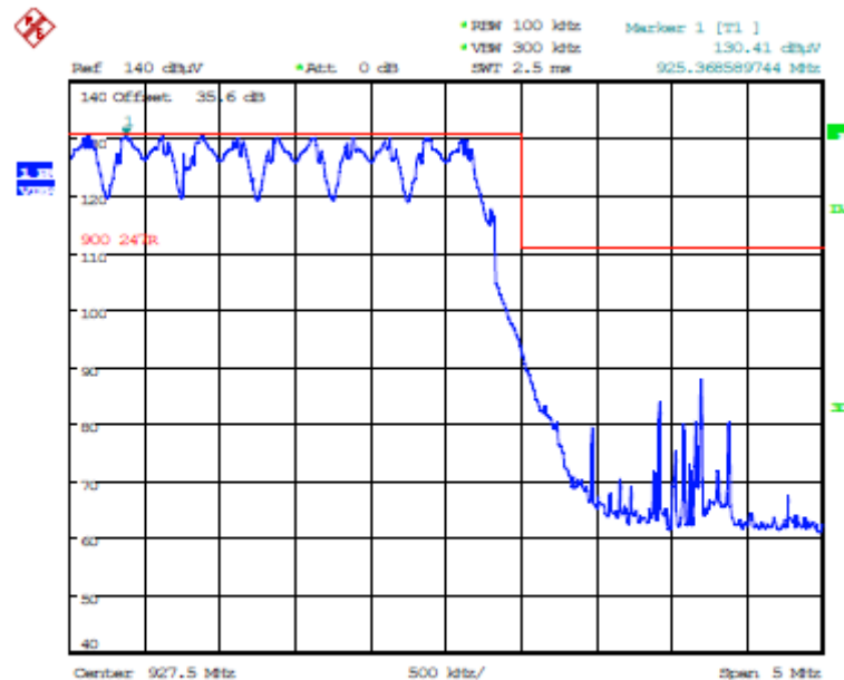
Plot 5.5.3.5.3.16. Band-Edge RF Radiated Emissions at 3 m, Vertical Polarization Pseudorandom Hopping Mode, High End of Frequency Band, 927.5 MHz, GFSK DSSS1, 400 kbps
