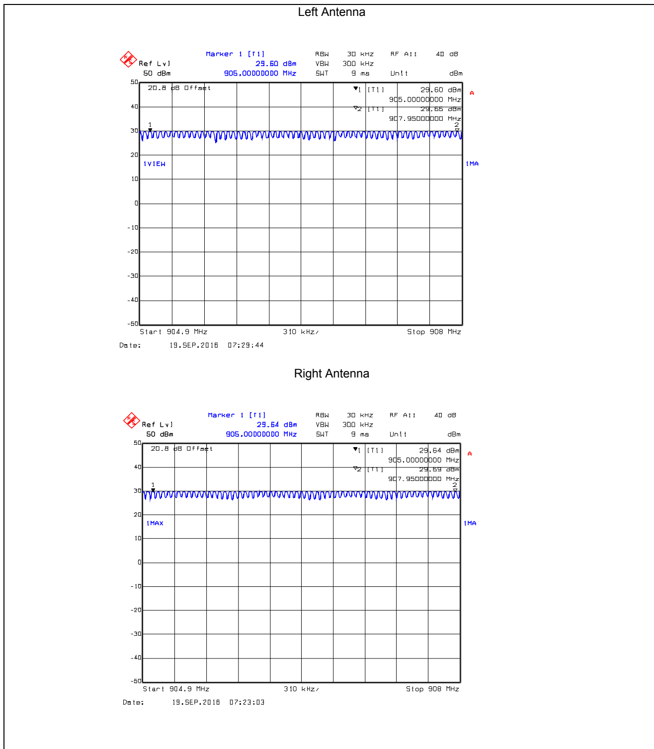
Plot 5.3.4.66. Number of Hopping Frequencies, DSSS8, 10 kbps 60 Hopping Channels from 905 – 908 MHz
