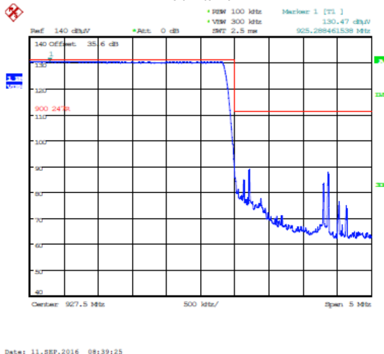
Plot 5.5.3.5.5.8. Band-Edge RF Radiated Emissions at 3 m, Vertical Polarization Pseudorandom Hopping Mode, High End of Frequency Band, 927.8 MHz, GFSK DSSS8, 10 kbps
