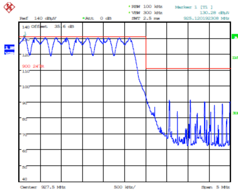
Plot 5.5.3.5.16. Band-Edge RF Radiated Emissions at 3 m, Vertical Polarization Pseudorandom Hopping Mode, High End of Frequency Band, 927.5 MHz, GFSK DSSS1, 400 kbps Left Antenna
