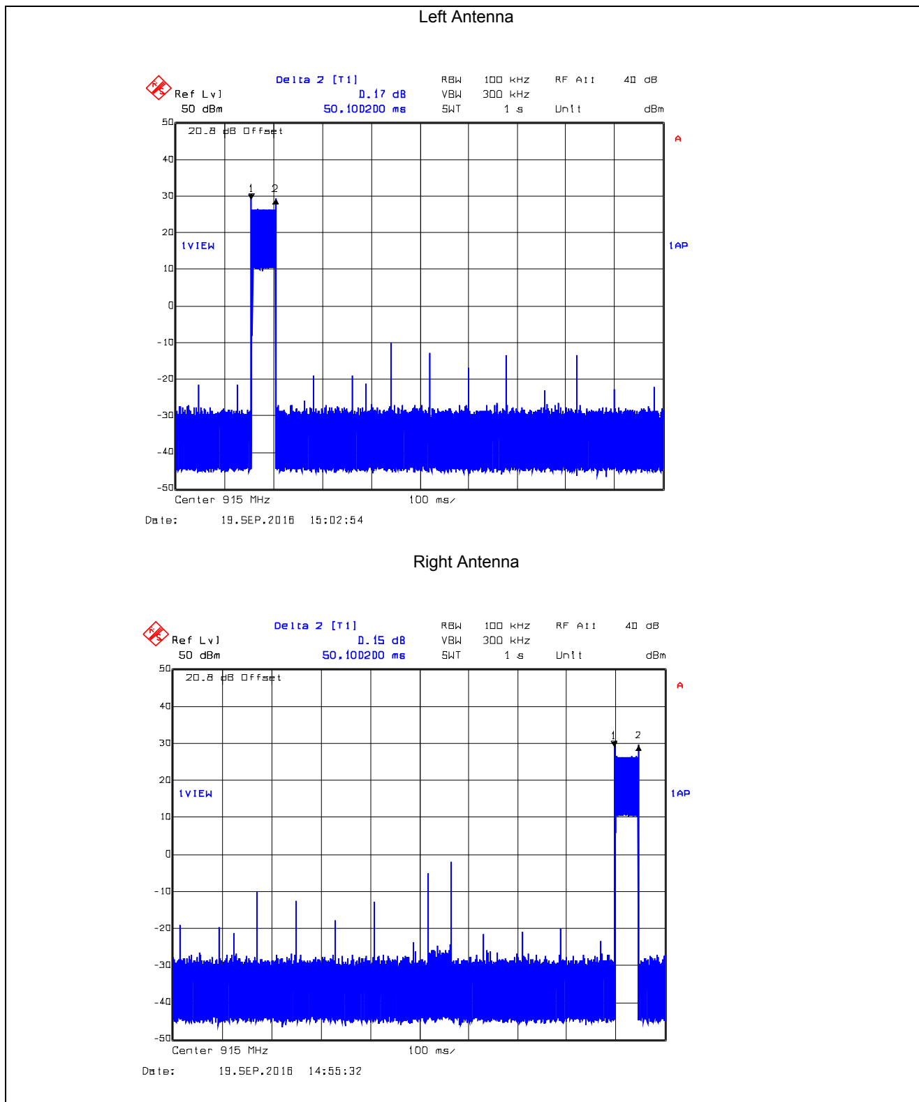
Plot 5.3.4.87. Time of Occupancy, 915.0 MHz, DSSS8, 400 kbps Dwell Time @ 915.0 MHz = 50.1 ms
