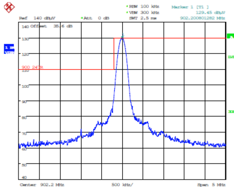
Plot 5.5.3.5.4.1. Band-Edge RF Radiated Emissions at 3 m, Horizontal Polarization Single Frequency Mode, Low End of Frequency Band, 902.2 MHz, GFSK DSSS8, 10 kbps Left Antenna
