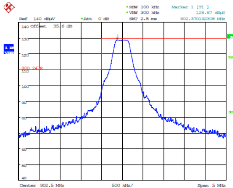
Plot 5.5.3.5.4.11. Band-Edge RF Radiated Emissions at 3 m, Vertical Polarization Single Frequency Mode, Low End of Frequency Band, 902.5 MHz, GFSK DSSS1, 400 kbps
