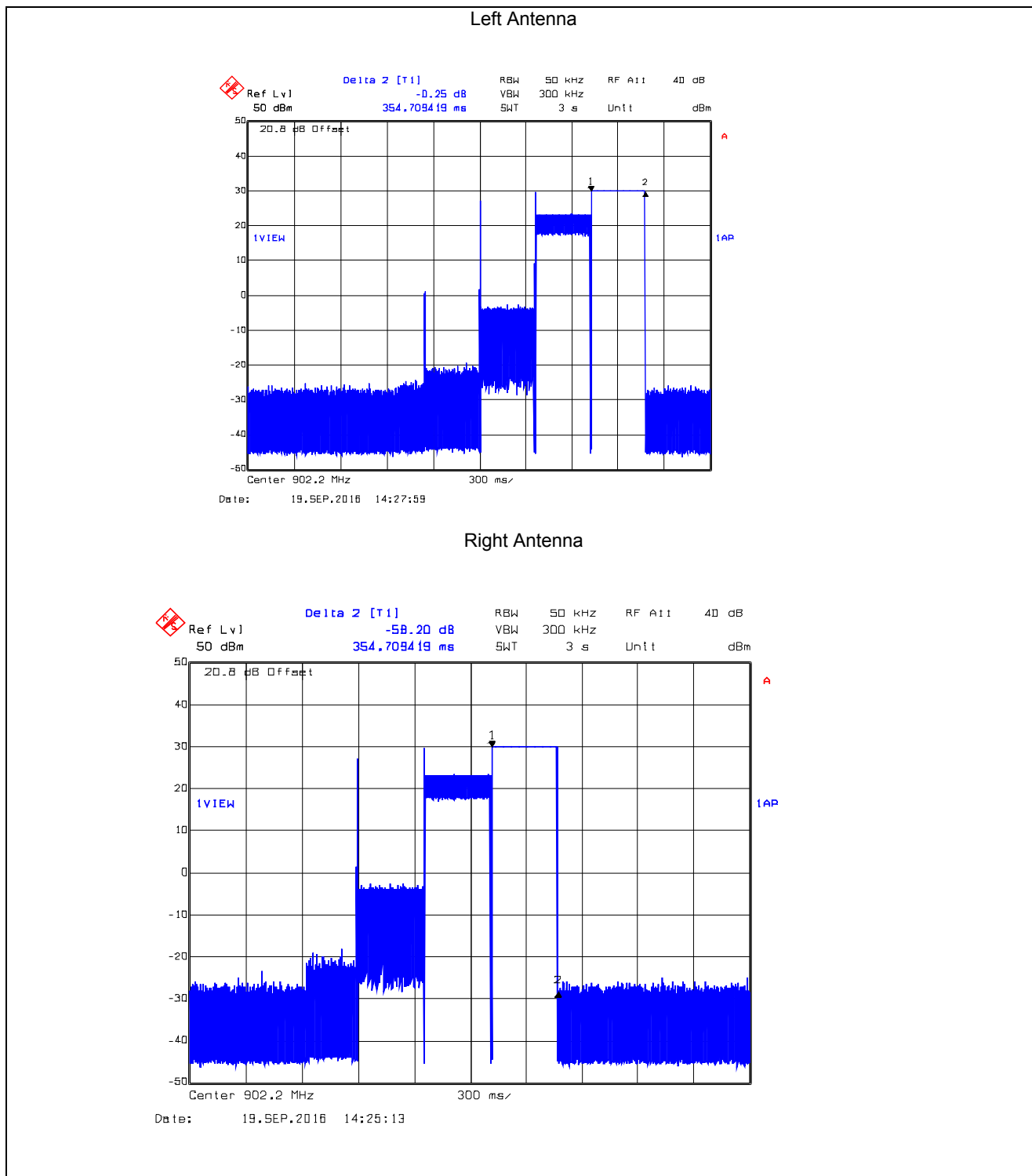
Plot 5.3.4.79. Time of Occupancy, 902.2 MHz, DSSS8, 10 kbps Dwell Time @ 902.2 MHz = 354.71ms
