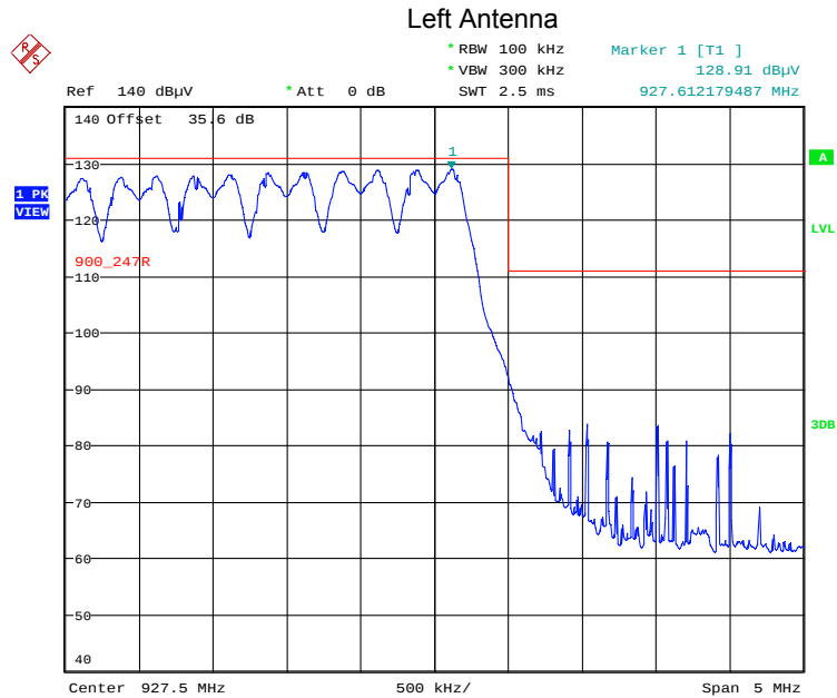
Plot 5.3.5.2.16. Band-Edge RF Radiated Emissions at 3 m, Vertical Polarization Pseudorandom Hopping Mode, High End of Frequency Band, 927.5 MHz, GFSK DSSS1, 400 kbps
