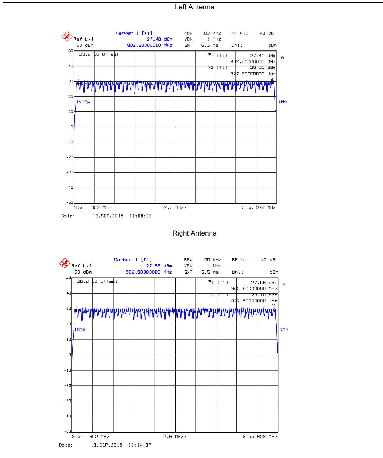
Plot 5.3.4.78. Total Number of Hopping Frequencies, DSSS8, 400 kbps 51 Hopping Channels from 902 – 928 MHz ( 15+20+16 = 51 )
