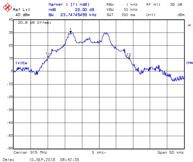
Plot 5.3.4.4. 20 dB Bandwidth, 915 MHz, GFSK, 10 kbps-Right Antenna
