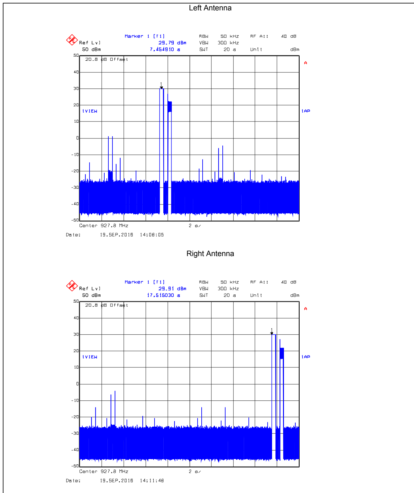
Plot 5.3.4.84. Time of Occupancy, 927.8 MHz DSSS8, 10 kbps Average time of occupancy = 1 \times (T_{on}) in 20s = 1 \times 354.71 \text{ ms} = 354.71 \text{ ms} < 400 \text{ ms}
