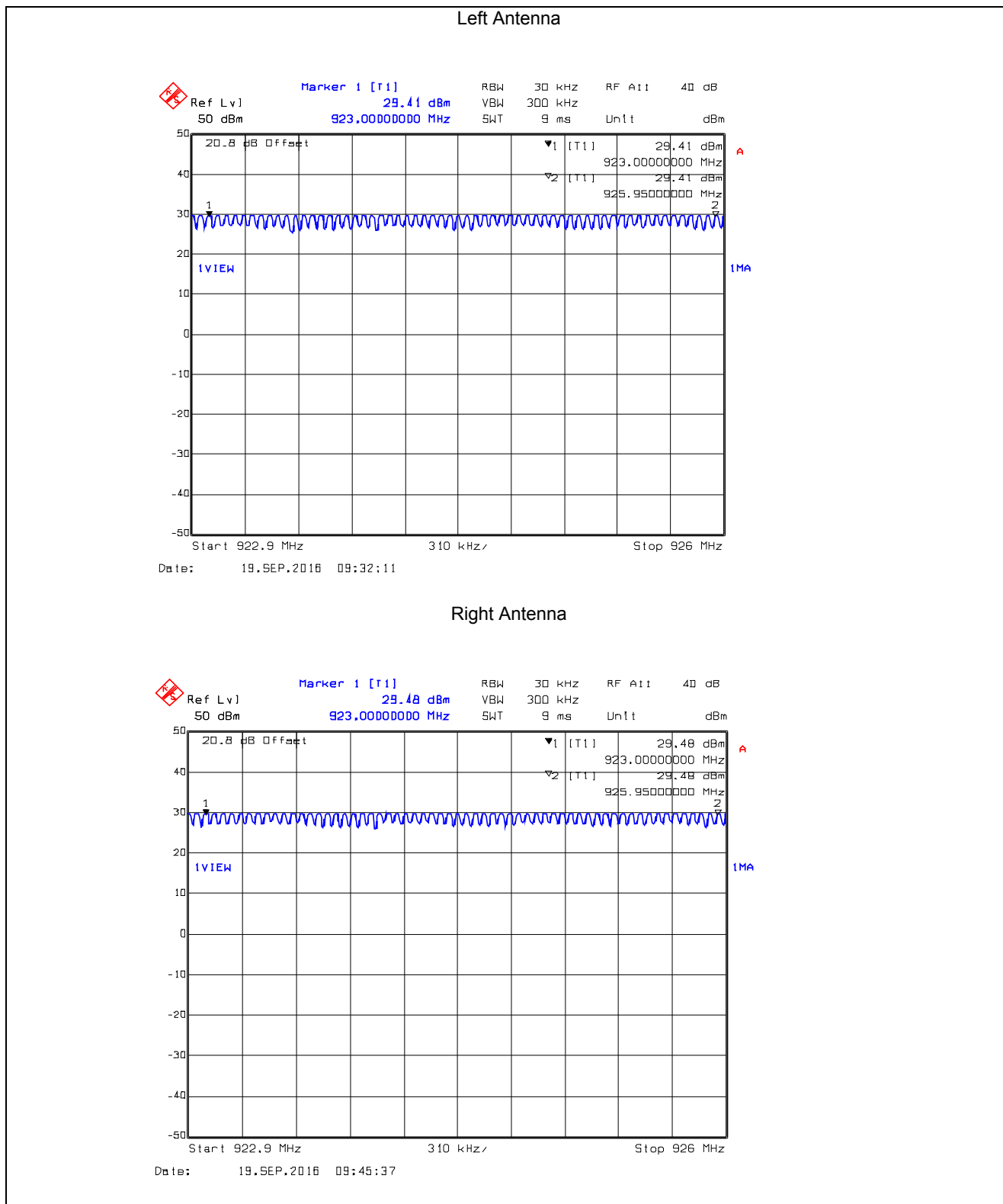
Plot 5.3.4.72. Number of Hopping Frequencies, DSSS8, 10 kbps 60 Hopping Channels from 923 – 926 MHz
