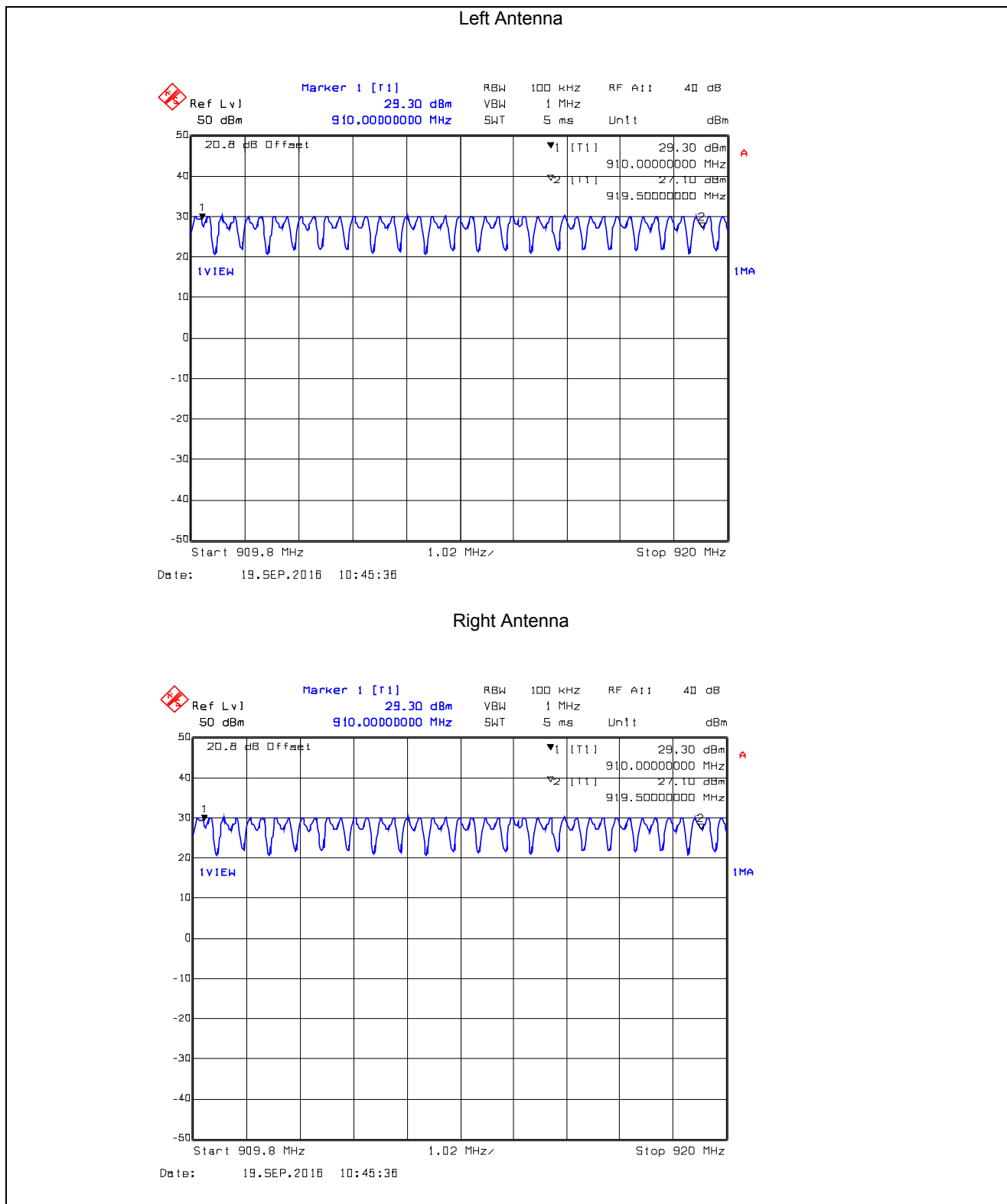
Plot 5.3.4.76. Number of Hopping Frequencies, DSSS8, 400 kbps 20 Hopping Channels from 910 – 919.5 MHz
