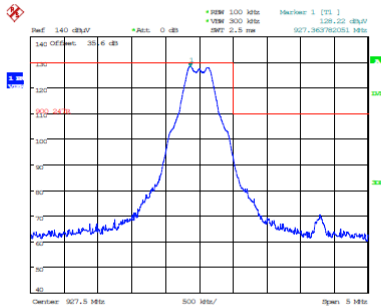
Plot 5.5.3.5.4.13. Band-Edge RF Radiated Emissions at 3 m, Horizontal Polarization Single Frequency Mode, High End of Frequency Band, 927.5 MHz, GFSK DSSS1, 400 kbps Left Antenna
