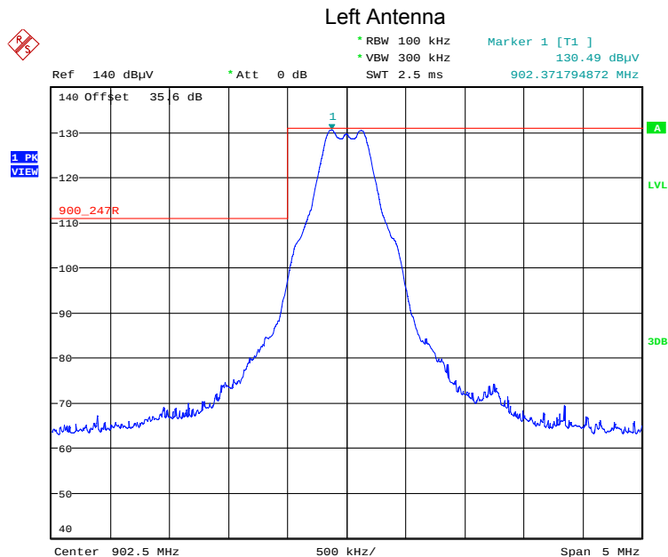
Plot 5.5.3.5.2.11. Band-Edge RF Radiated Emissions at 3 m, Vertical Polarization Single Frequency Mode, Low End of Frequency Band, 902.5 MHz, GFSK DSSS1, 400 kbps
