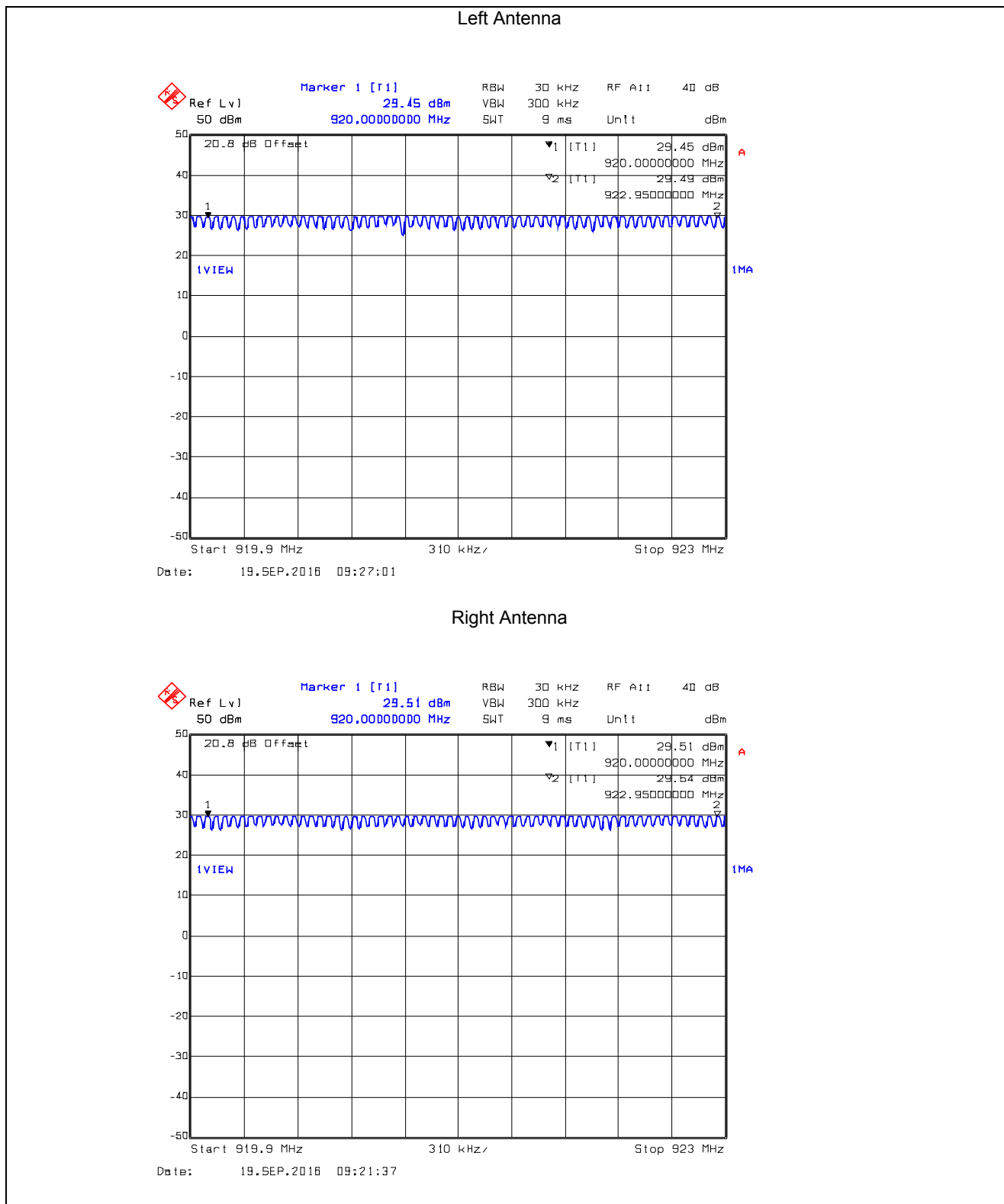
Plot 5.3.4.71. Number of Hopping Frequencies, DSSS8, 10 kbps 60 Hopping Channels from 920 – 923 MHz
