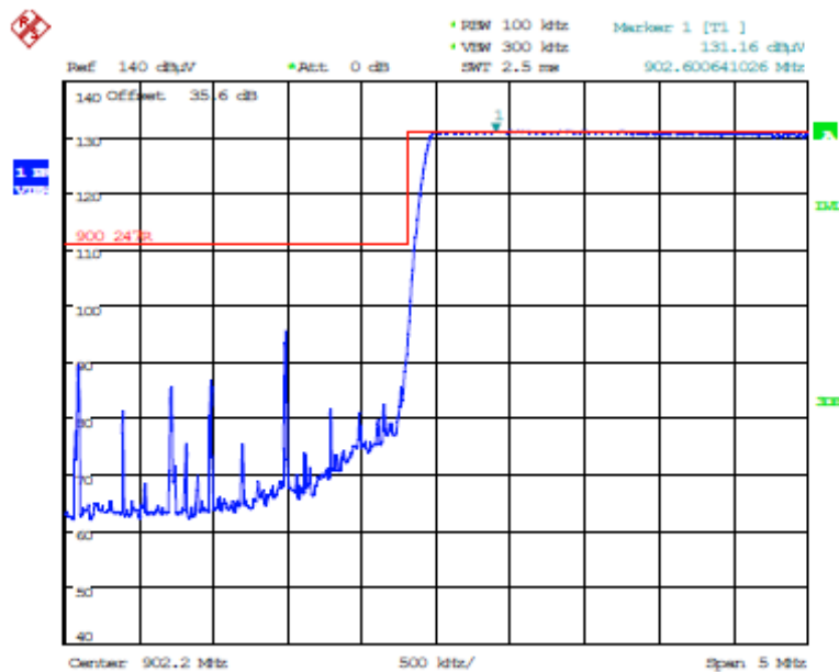
Plot 5.5.3.5.4. Band-Edge RF Radiated Emissions at 3 m, Vertical Polarization Pseudorandom Hopping Mode, Low End of Frequency Band, 902.2 MHz GFSK DSSS8, 10 kbps
