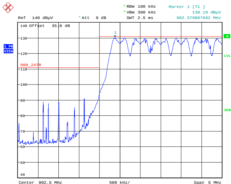
Plot 5.5.3.5.2.12. Band-Edge RF Radiated Emissions at 3 m, Vertical Polarization Pseudorandom Hopping Mode, Low End of Frequency Band, 902.5 MHz, GFSK DSSS1, 400 kbps Left Antenna
