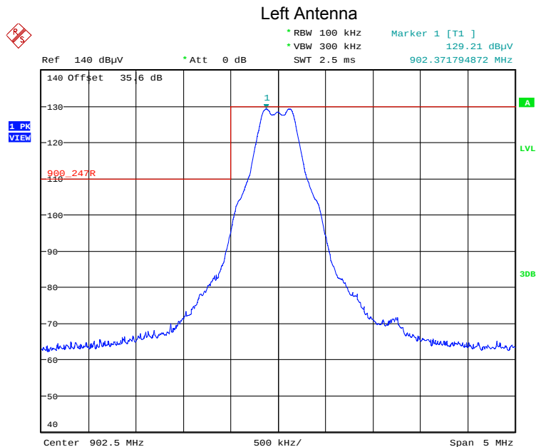
Plot 5.5.3.5.2.9. Band-Edge RF Radiated Emissions at 3 m, Horizontal Polarization Single Frequency Mode, Low End of Frequency Band, 902.5 MHz, GFSK DSSS1, 400 kbps
