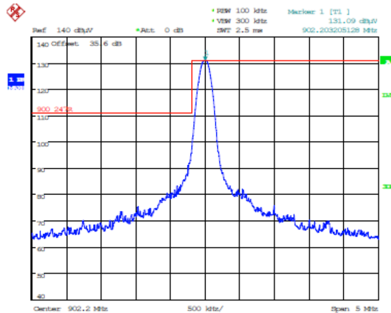
Plot 5.5.3.5.3. Band-Edge RF Radiated Emissions at 3 m, Vertical Polarization Single Frequency Mode, Low End of Frequency Band, 902.2 MHz, GFSK DSSS8, 10 kbps
