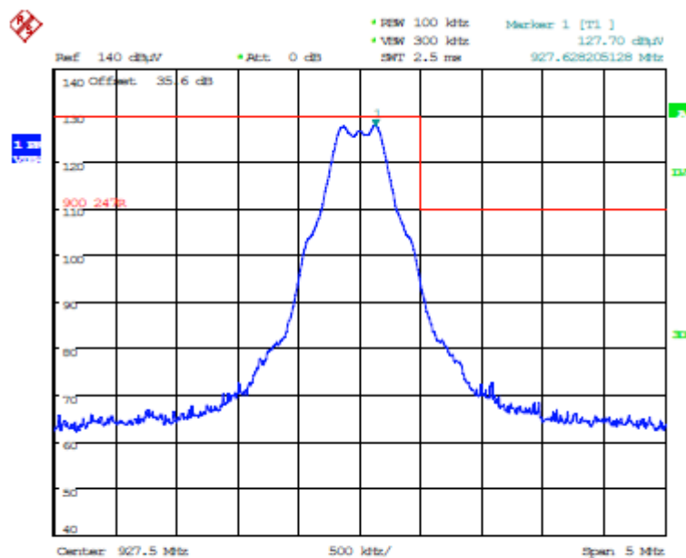
Plot 5.5.3.5.4.15. Band-Edge RF Radiated Emissions at 3 m, Vertical Polarization Single Frequency Mode, High End of Frequency Band, 927.5 MHz, GFSK DSSS1, 400 kbps
