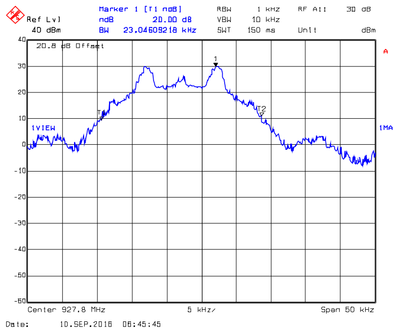
Plot 5.3.4.6. 20 dB Bandwidth, 927.8 MHz, GFSK, 10 kbps-Right Antenna
