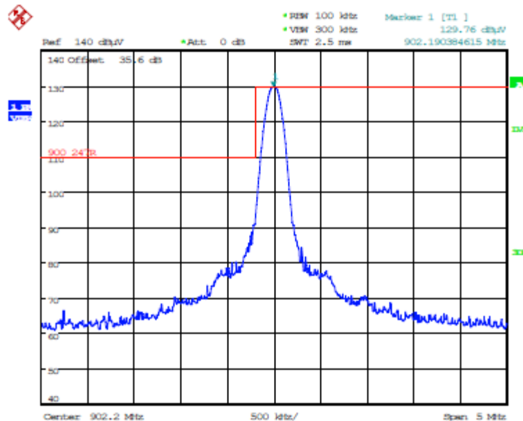
Plot 5.5.3.5.4.3. Band-Edge RF Radiated Emissions at 3 m, Vertical Polarization Single Frequency Mode, Low End of Frequency Band, 902.2 MHz, GFSK DSSS8, 10 kbps
