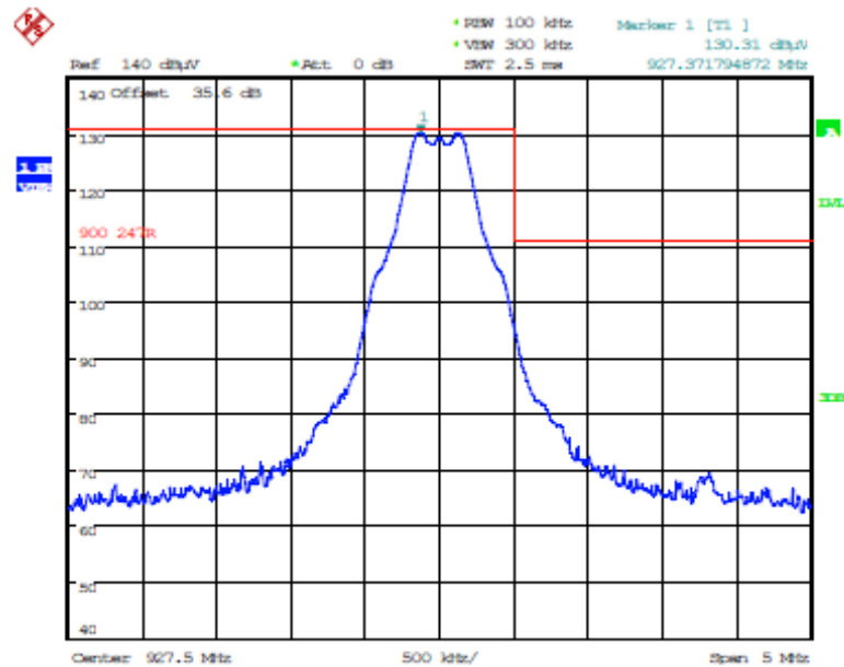
Plot 5.5.3.5.15. Band-Edge RF Radiated Emissions at 3 m, Vertical Polarization Single Frequency Mode, High End of Frequency Band, 927.5 MHz, GFSK DSSS1, 400 kbps
