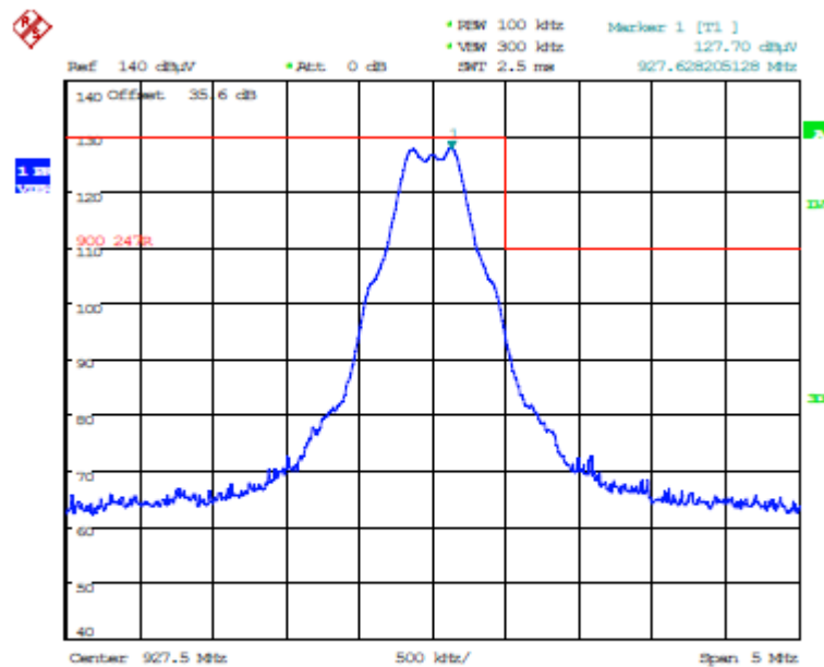
Plot 5.5.3.5.4.15. Band-Edge RF Radiated Emissions at 3 m, Vertical Polarization Single Frequency Mode, High End of Frequency Band, 927.5 MHz, GFSK DSSS1, 400 kbps Left Antenna
