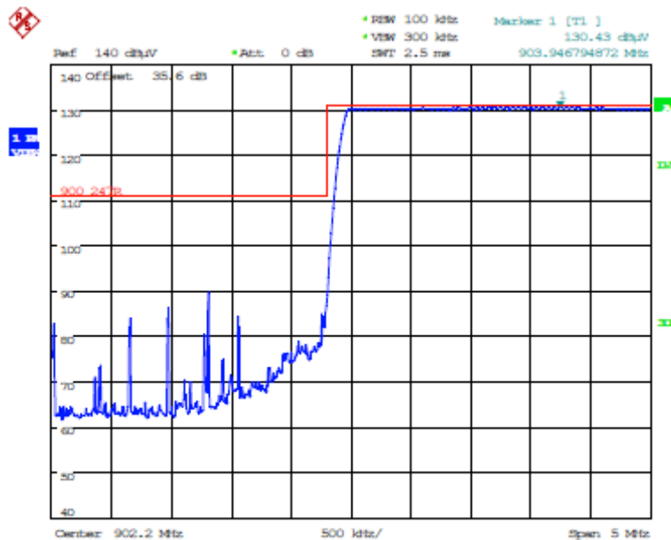
Plot 5.5.3.5.2. Band-Edge RF Radiated Emissions at 3 m, Horizontal Polarization Pseudorandom Hopping Mode, Low End of Frequency Band, 902.2 MHz, GFSK DSSS8, 10 kbps
