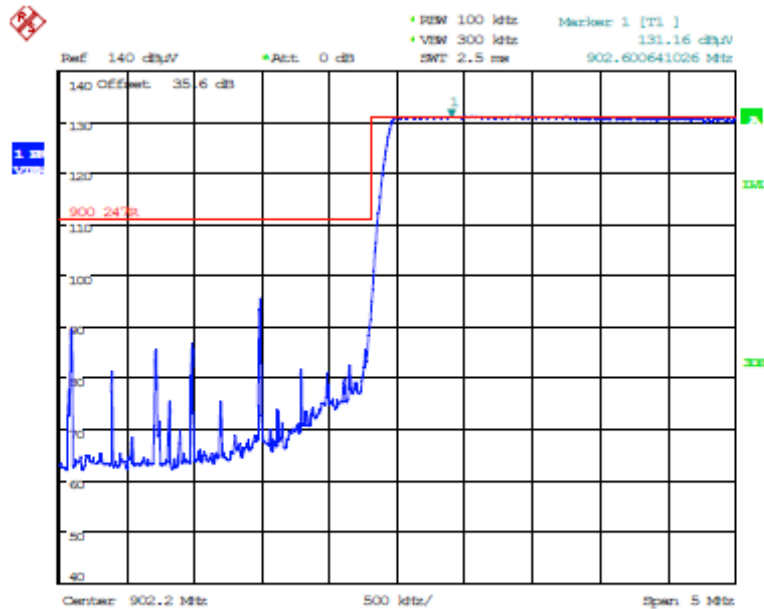
Plot 5.5.3.5.4. Band-Edge RF Radiated Emissions at 3 m, Vertical Polarization Pseudorandom Hopping Mode, Low End of Frequency Band, 902.2 MHz GFSK DSSS8, 10 kbps
