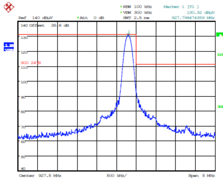
Plot 5.5.3.5.7. Band-Edge RF Radiated Emissions at 3 m, Vertical Polarization Single Frequency Mode, High End of Frequency Band, 927.8 MHz, GFSK DSSS8, 10 kbps
