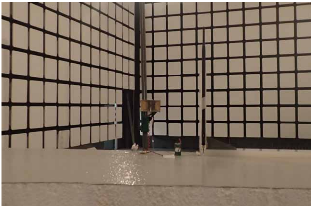
Radiated Emissions @ 3 m, Orthogonal Position 3 EUT with 5.0 dBi Dipole Antenna
