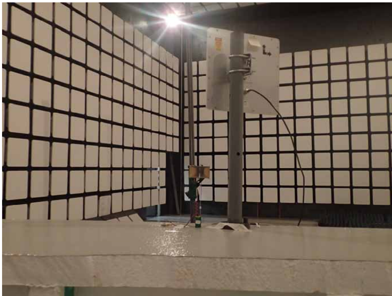
Radiated Emissions @ 3 m EUT with 9.0 dBi Flat Panel Antenna
