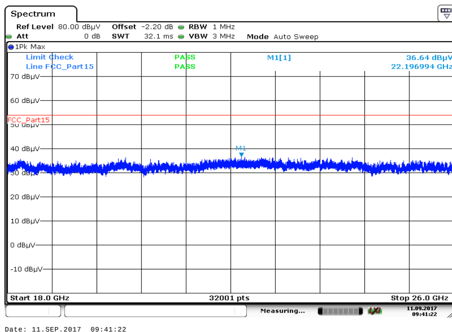
Plot 2: 18 GHz to 26 GHz, RX / idle – mode, lowest channel, vertical & horizontal polarization
