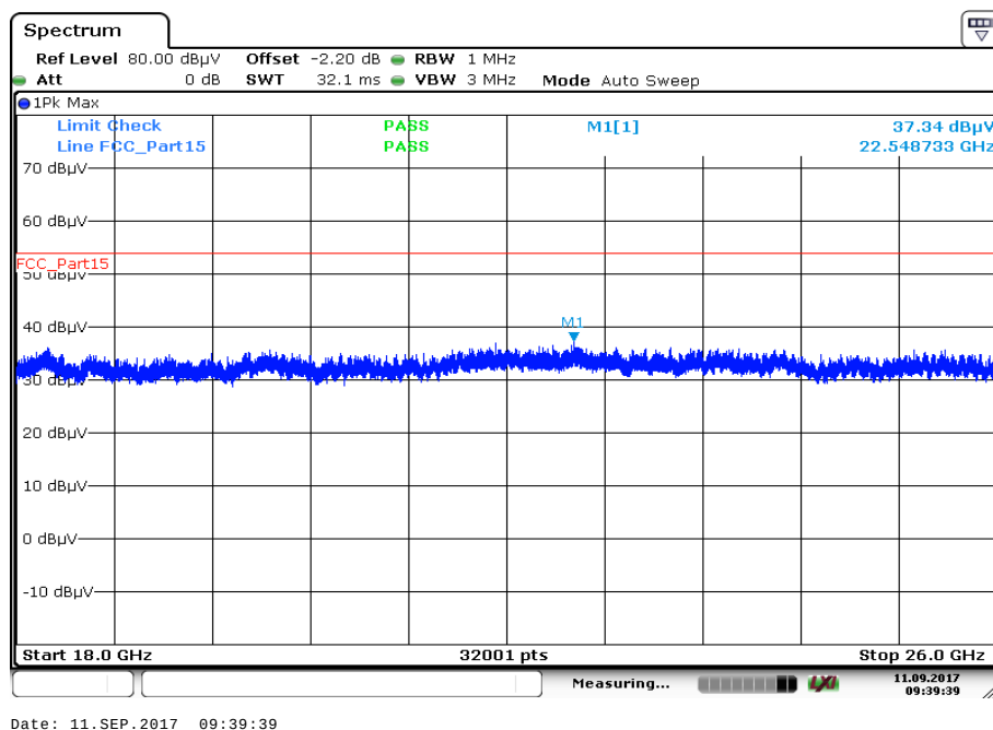
Plot 4: 18 GHz to 26 GHz, RX / idle – mode, highest channel, vertical & horizontal polarization
