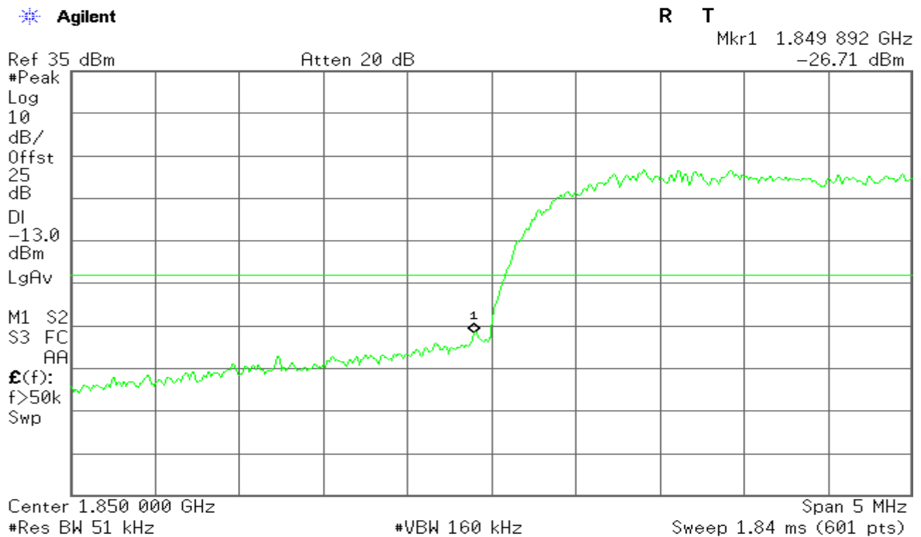
Figure 10-1: Band Edge emissions –HSDPA CH Low
