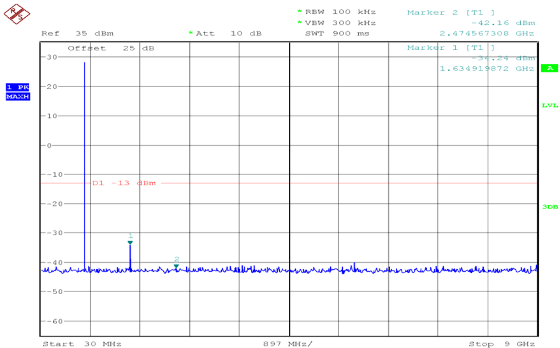
Figure 16-1: Out of Band emission at antenna terminals – GPRS CH Low
