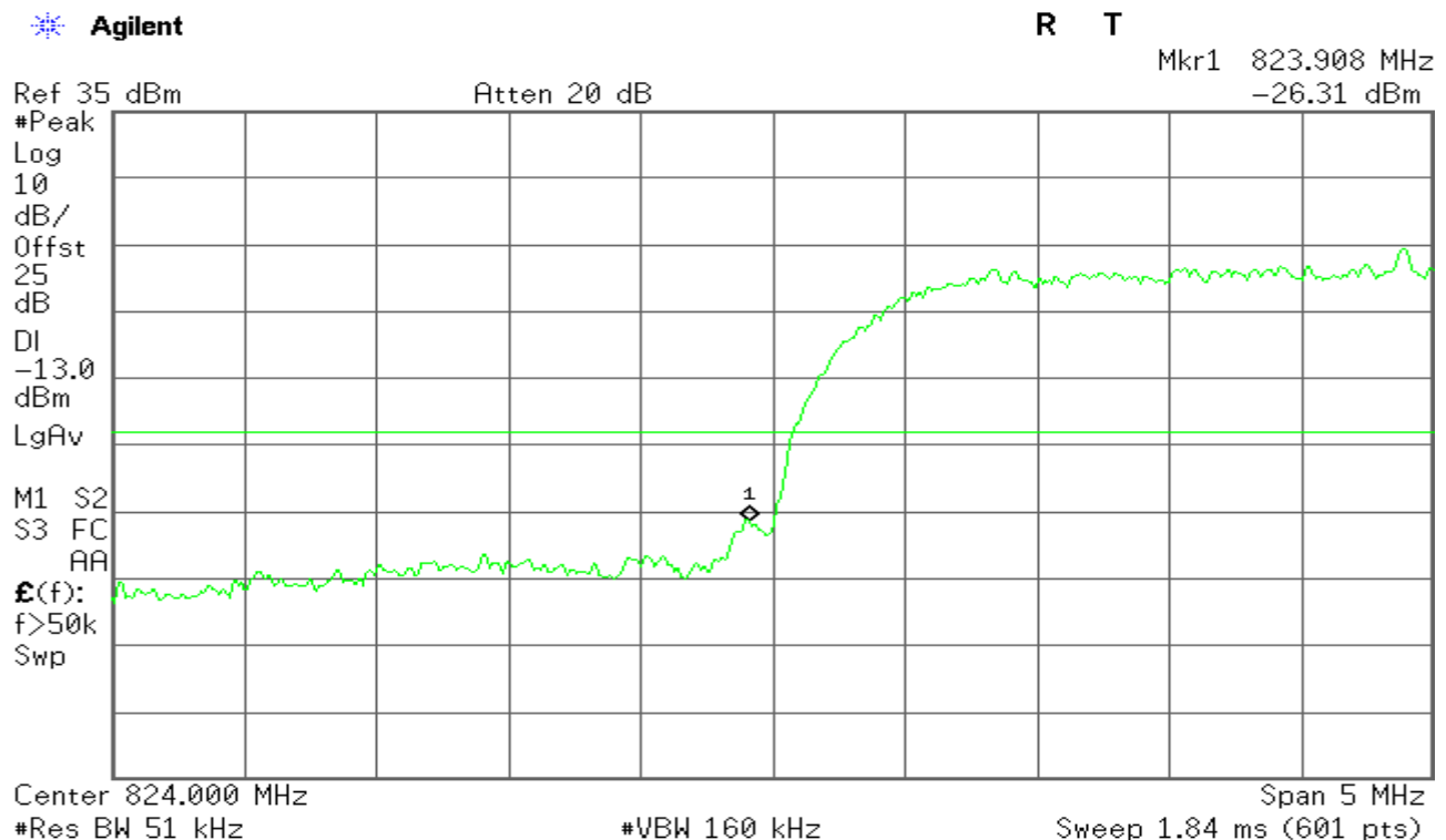
Figure 12-1: Band Edge emissions –WCDMA CH Low
