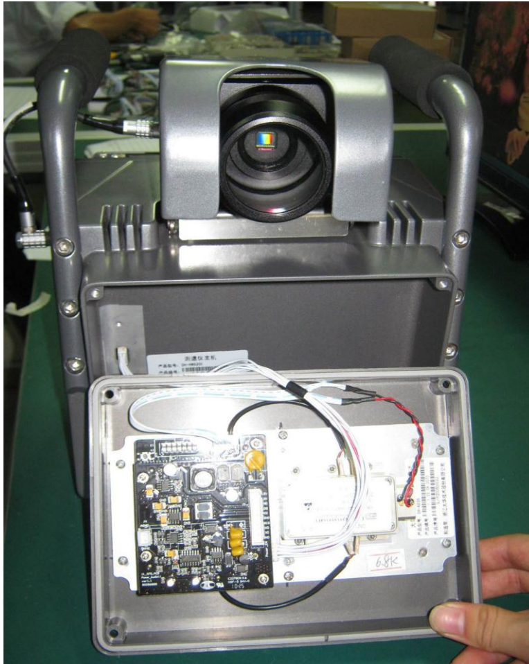
Radar Inside (Right side is Transmitter)
