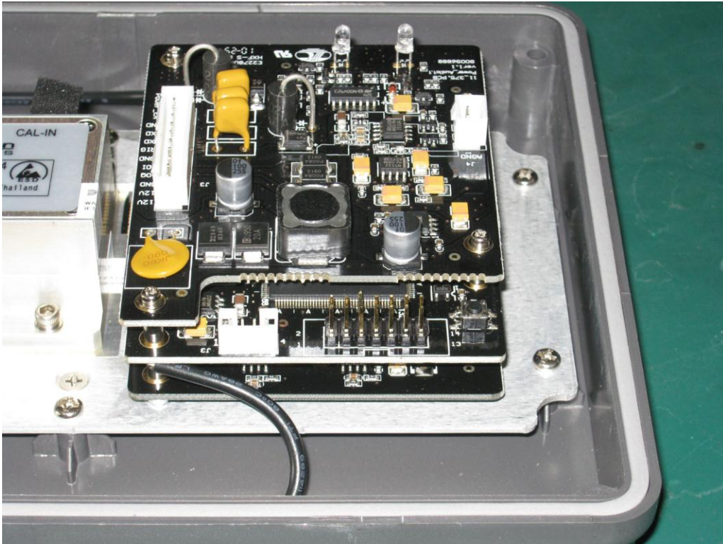
Rad Main Board Side View
