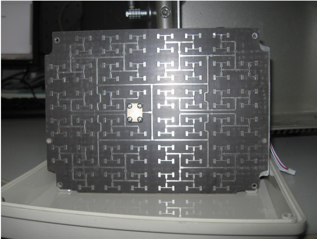
Top Side of Main Board
