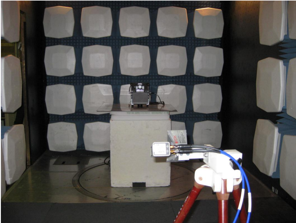
Radiated Measurements Fundamental #1
