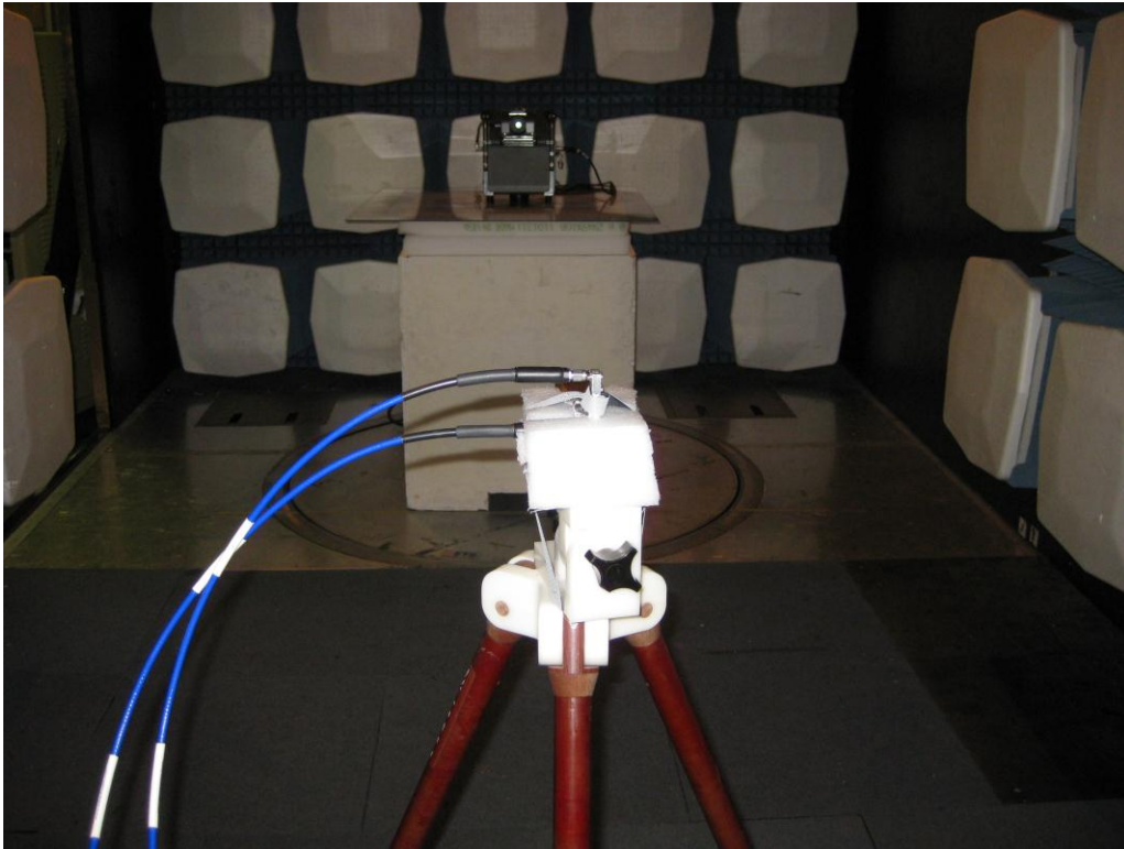
Radiated Measurements Harmonics #2
