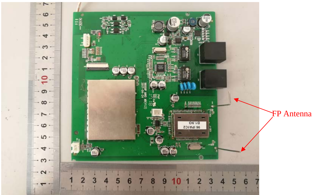
EUT – PCB-4 Top View
