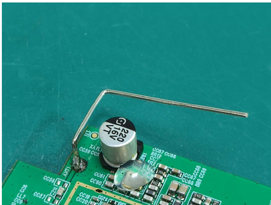
DECT ANT1
